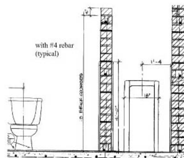
bond beam
