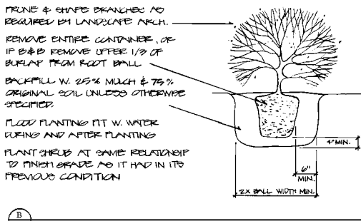
planting detail
