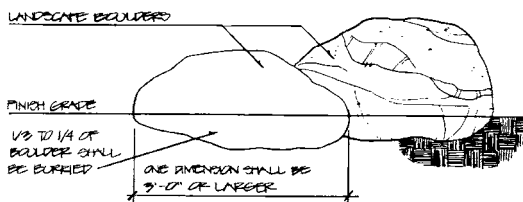
boulder detail
