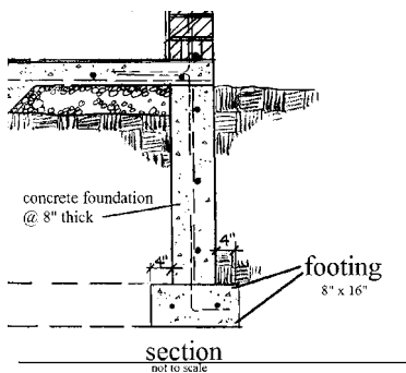
footing
