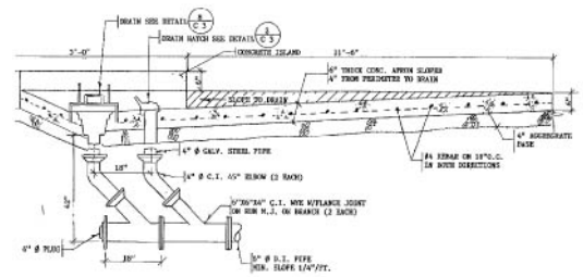
dump station apron and drains
