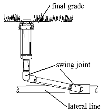
rotor pop-up sprinkler head
