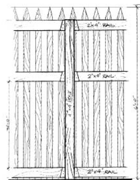
picket fence
