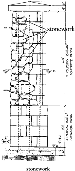
stonework
