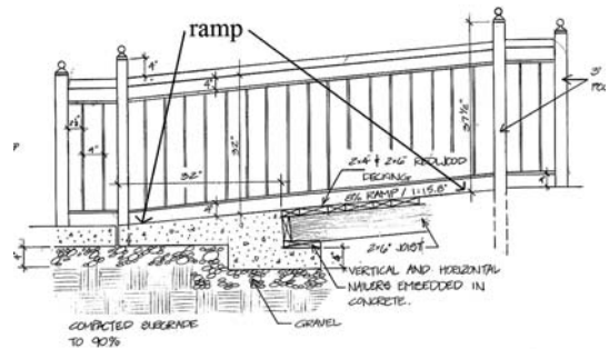
ramp
