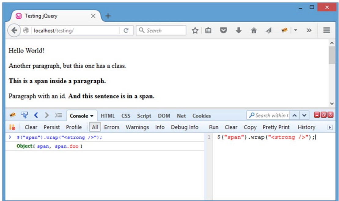
Figure 2-8. The spans appear bold after wrapping them with strong tags
