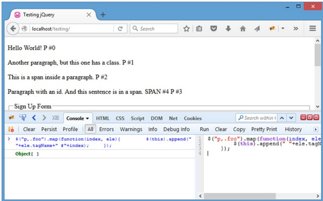
Figure 2-19. The test page after mapping a callback function to display names and indexes for each element
