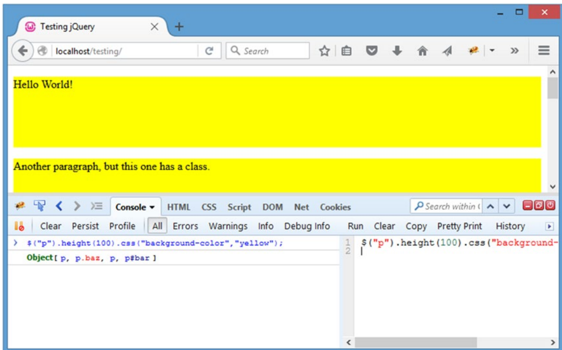
Figure 2-18. The modified height and backgrounds of all document paragraphs
