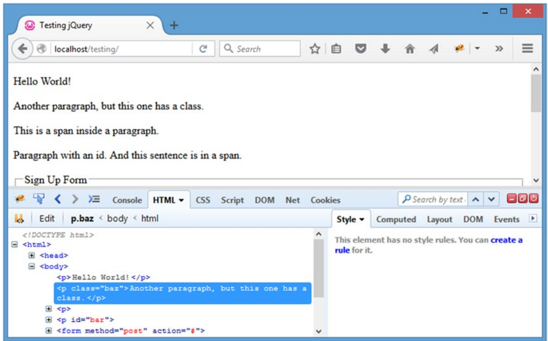
Figure 2-17. The foo class is removed, and the baz class is added
