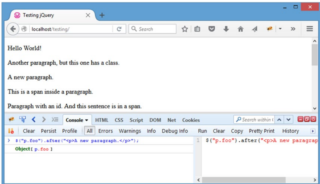
Figure 2-7. A new paragraph inserted after the paragraph with class foo
