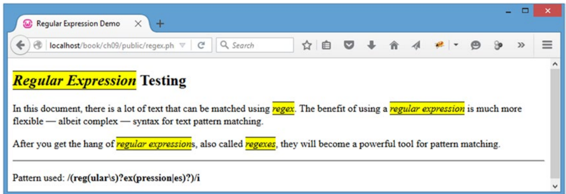
Figure 9-13. Adding alternation to match expression
