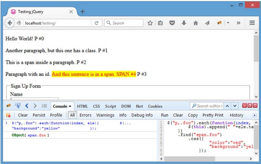
Figure 2-20. Using .each() , the expected results are produced
