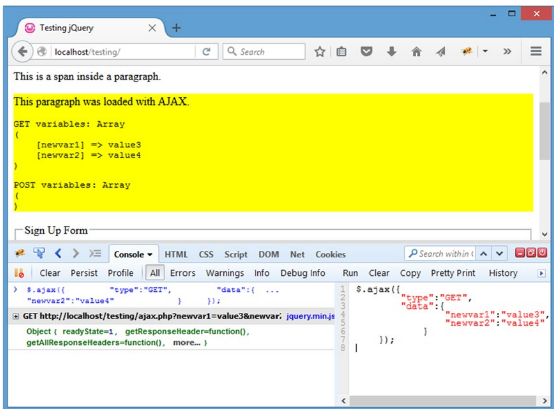
Figure 2-24. The result after overriding the default type option with GET
