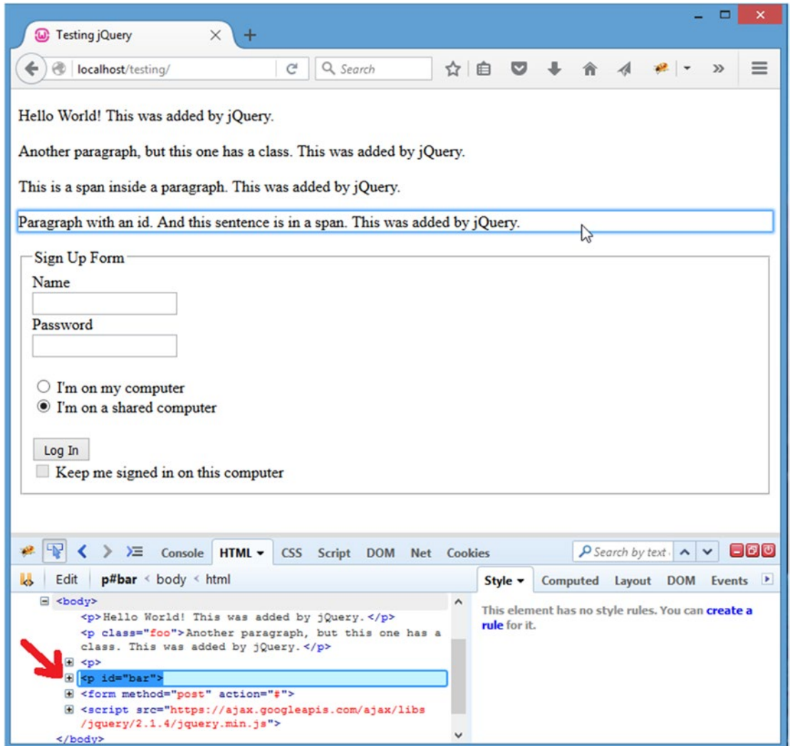
Figure 2-4. The collapsed element as displayed after hovering over and clicking it
