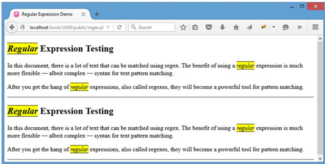
Figure 9-4. A more complex replacement
