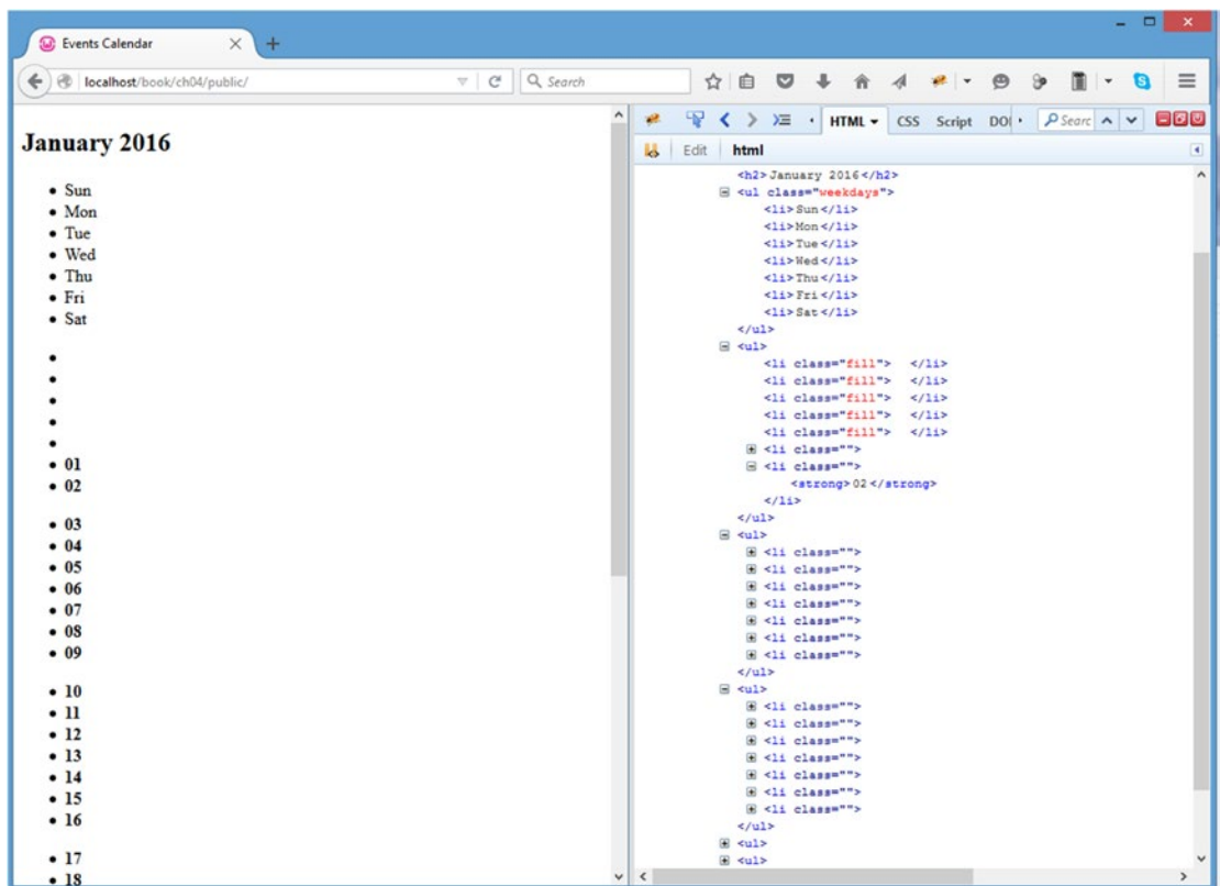
Figure 4-5. The markup as generated by buildCalendar()
