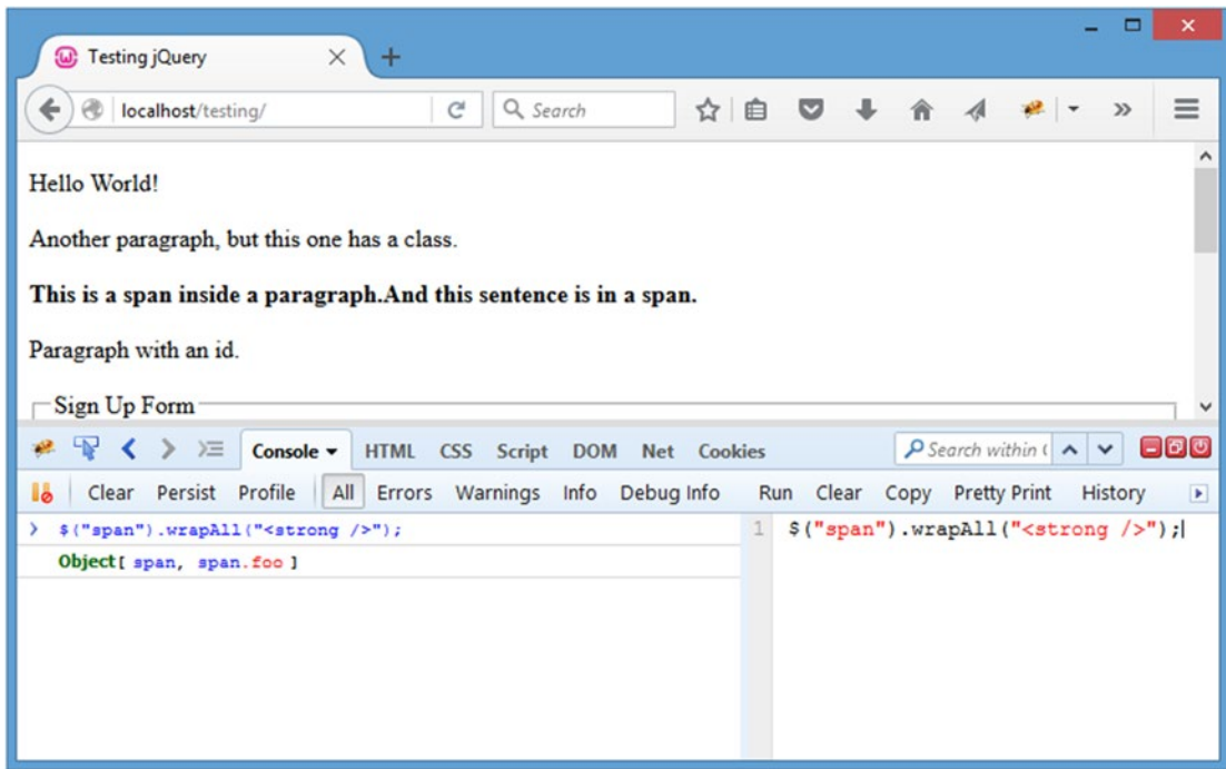
Figure 2-13. The spans are relocated to be next to one another so both can be wrapped
