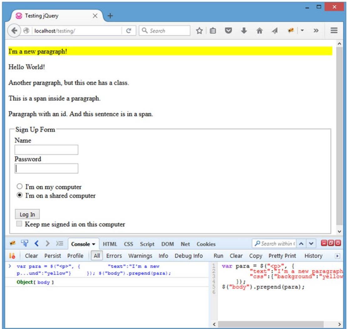
Figure 2-6. The new paragraph as it appears after prepending it to the body element
