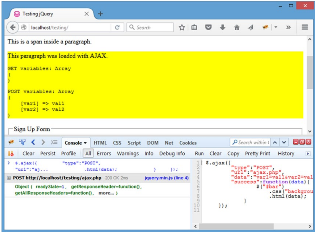
Figure 2-22. The loaded AJAX information from ajax.php
