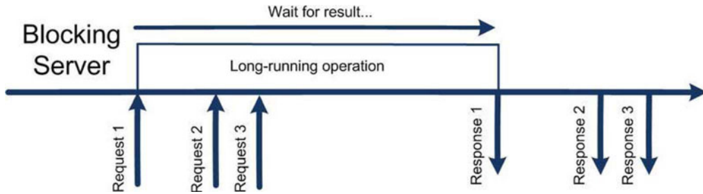
Figure 10-1. Blocking server flow
