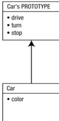
Figure 1-11. The properties defined on the prototype are available to the object
