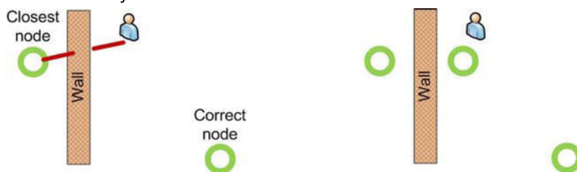
Figure 13-13. On the left, the problem with a naive pathfinding graph: due to the mistake of the level designer, the character attempts to move through the wall to reach the node. The corrected version is on the right.
