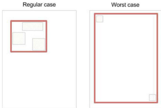
Figure 7-22. We have a small dirty rectangle in a regular case, but the worst case results in repainting the entire area.
