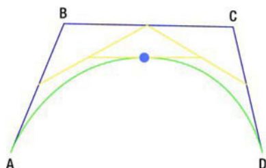
Figure 2-17. Example of a Bézier curve
