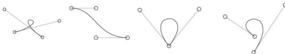
Figure 2-18. More Bézier curves
