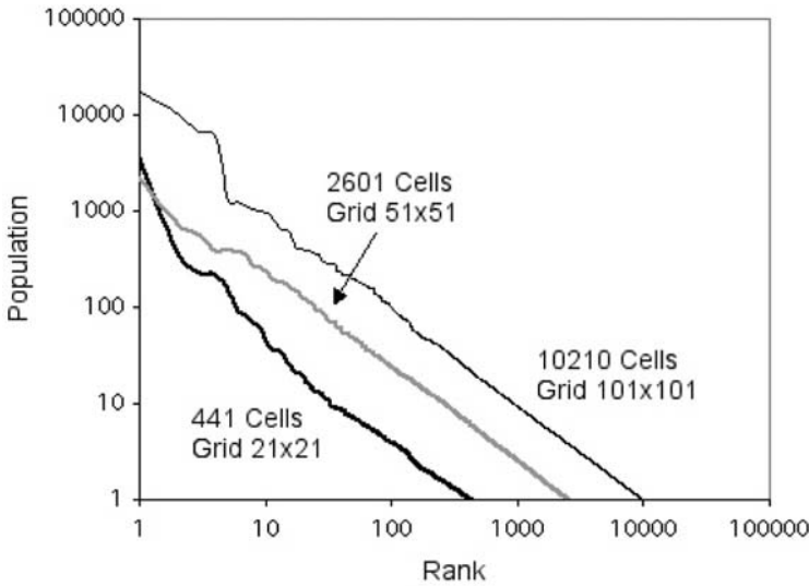
Figure 6: Consistent Scaling Behaviour for Different Sizes of Lattice
