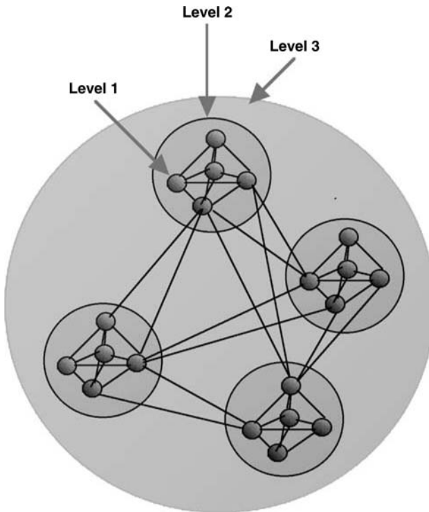
Figure 4: Organisation levels: living systems are self-organizing by assembling in networks. That leads to a hierarchy of nested levels. For example an organism (level 3) is composed of organs (level 2, even if not properly a level of organisation) and organs composed of cells (level 1); in ecology, a community (level 3) is constituted by interacting populations (level 2), themselves sets of interconnected organisms (level 1).
