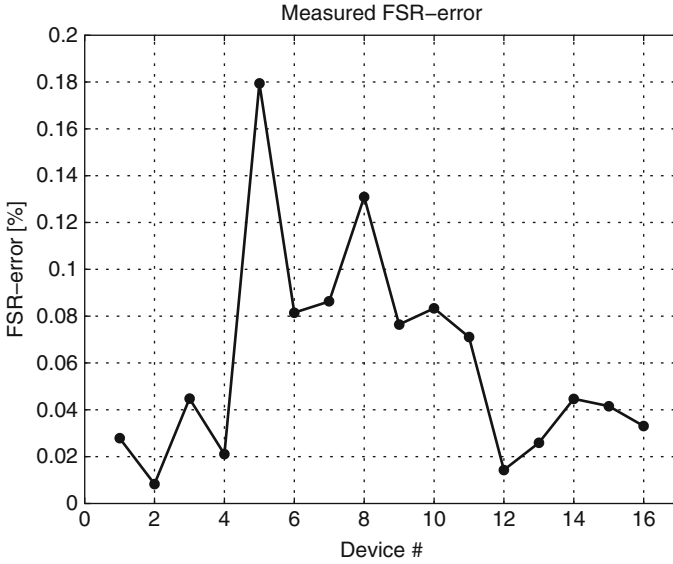
Fig. 5.29 FSR-error for different devices
