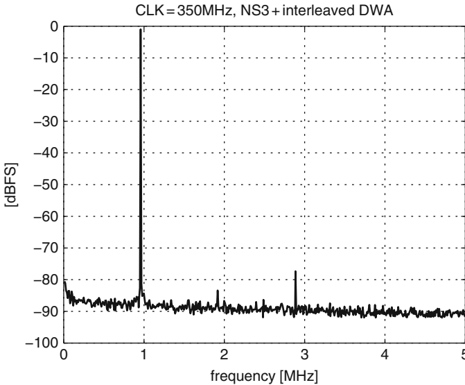
Fig. 5.30 1 MHz single-tone output spectrum
