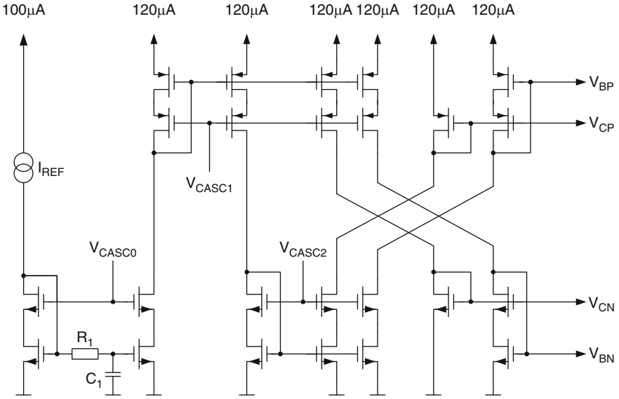
Fig. 5.21 Low-noise biasing
