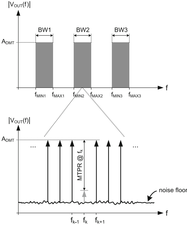
Fig. 2.9 Missing tone power ratio
