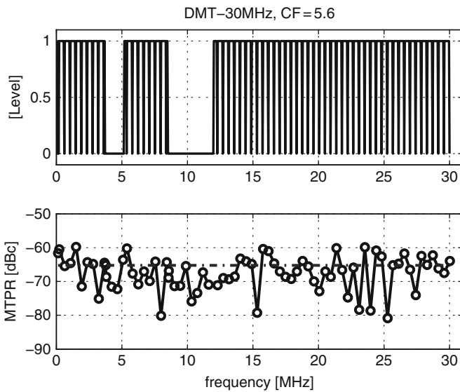
Fig. 6.23 30 MHz DMT-performance of full TX-chain
