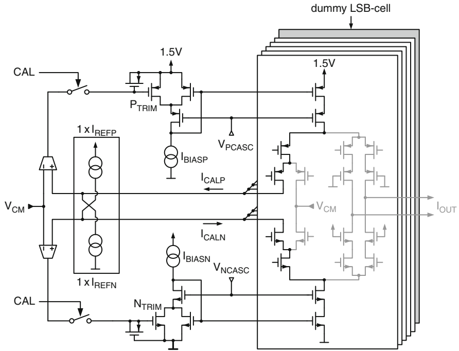
Fig. 6.33 LLSB-array with calibrated bias mirror
