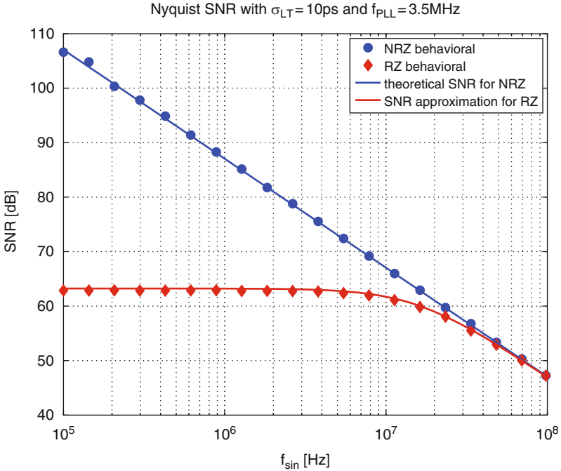
Fig. 2.25 Nyquist SNR with \sigma_{LT} = 10\text{ps} and f_{PLL} = 3.5\text{MHz}
