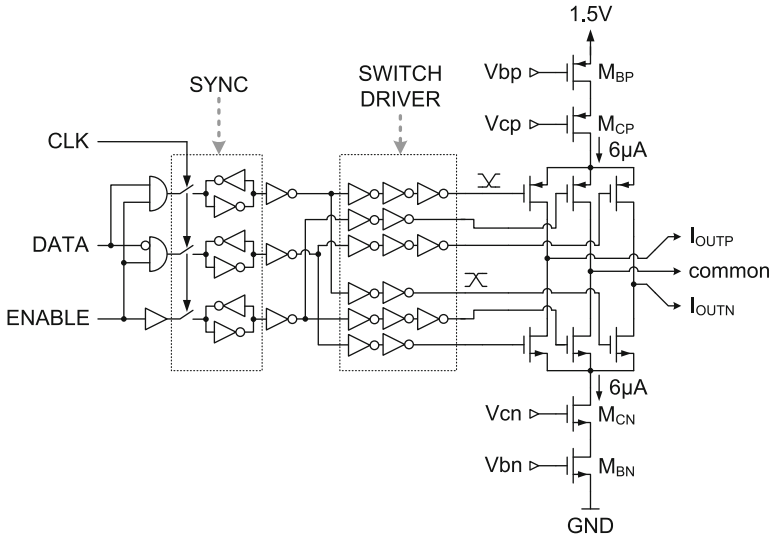
Fig. 5.20 Unit current cell for interleaved DAC
