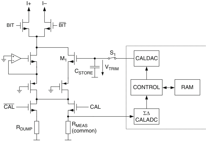
Fig. 3.15 Trimmable floating current source
