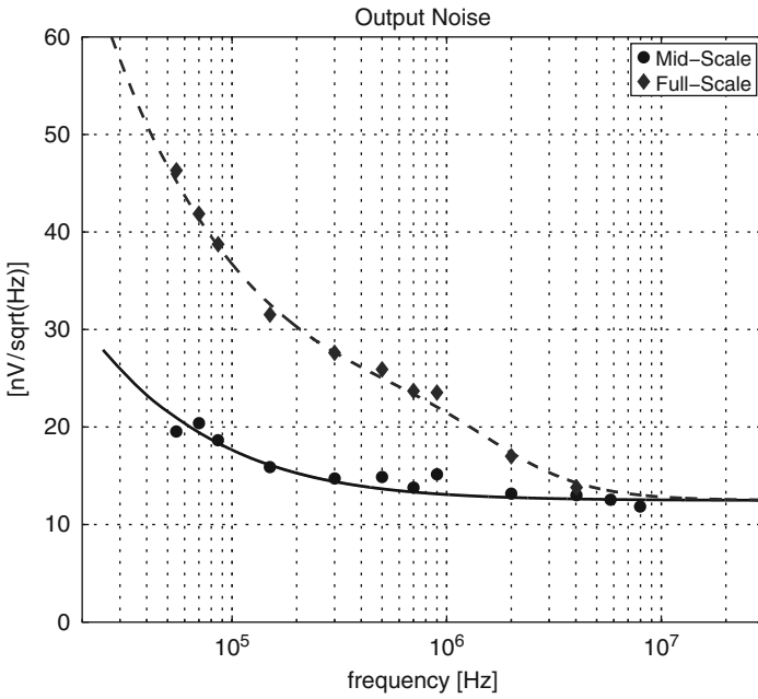
Fig. 5.22 Measured output noise
