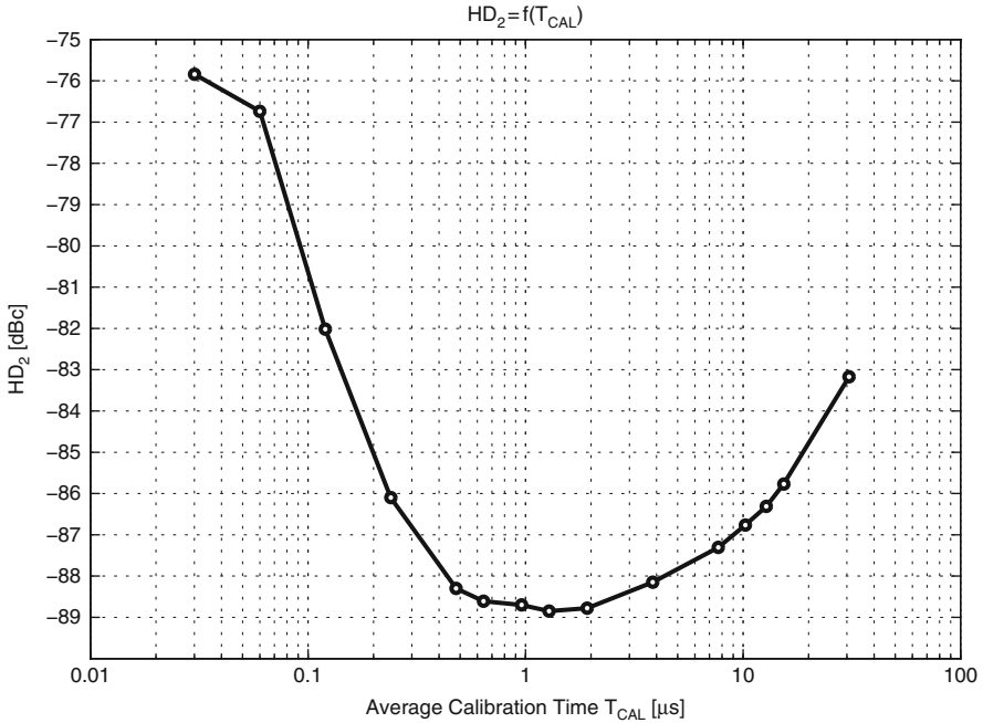
Fig. 6.15 HD_2 as function of the calibration slot length
