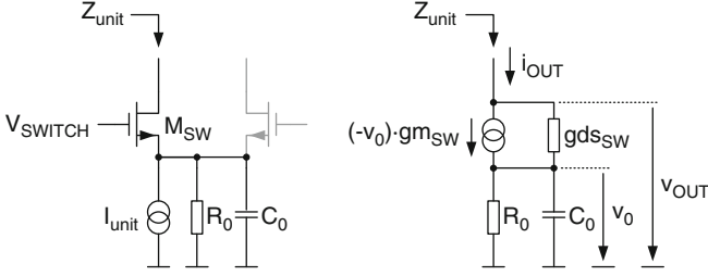
Fig. 4.1 Output impedance of single-polarity current cell
