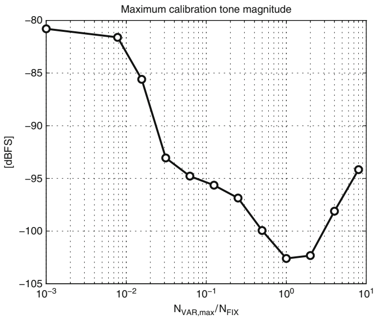
Fig. 6.17 Calibration spur magnitude vs. randomization
