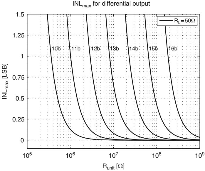
Fig. 3.7 INL_{\max} = f(R_{\text{unit}}) of differential converter
