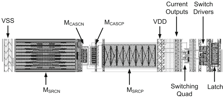
Fig. 5.5 Layout of unit current cell
