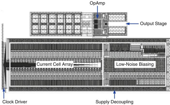
Fig. 5.6 DAC-core layout
