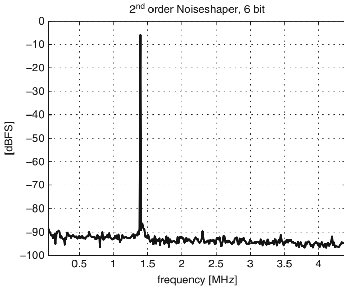
Fig. 6.25 1.4 MHz single-tone with noiseshaped MSB-segment
