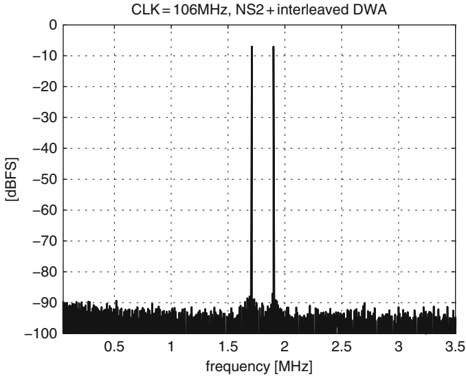
Fig. 5.34 Two-tone output spectrum
