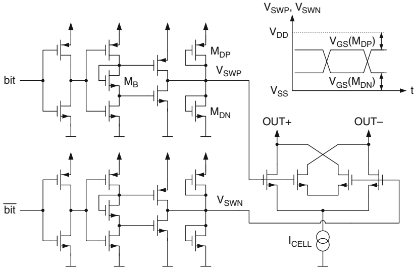
Fig. 4.15 Reduced swing switch driver
