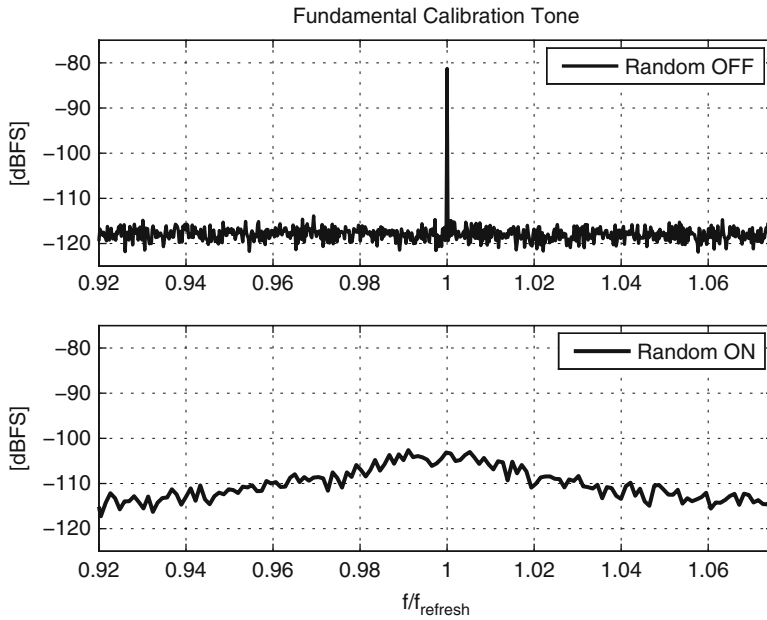
Fig. 6.16 Effect of randomization on calibration spur
