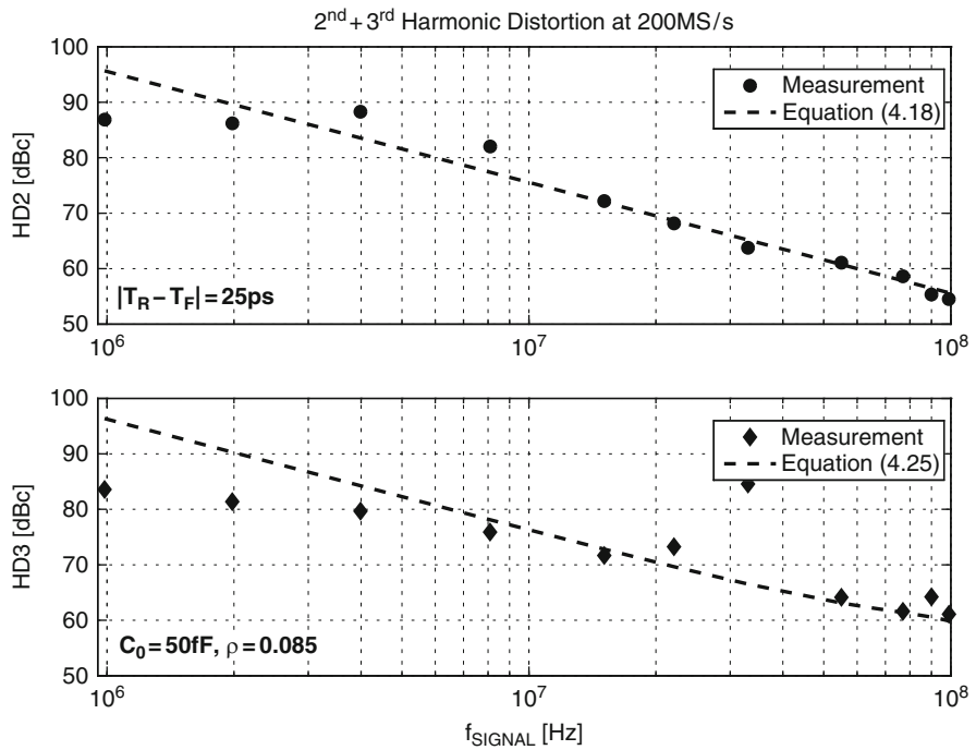
Fig. 6.20 HD 2 and HD 3 for 200 MS/s
