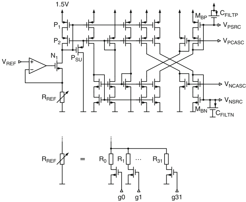
Fig. 6.35 Programmable converter biasing
