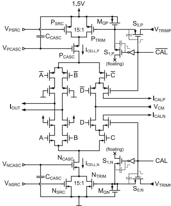
Fig. 6.29 Calibrated dual-polarity current cell
