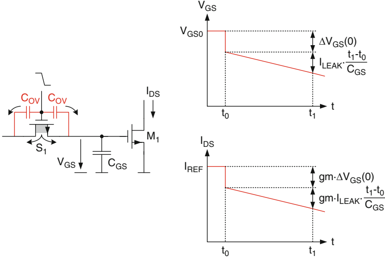
Fig. 3.17 Charge injection at the end of the calibration slot
