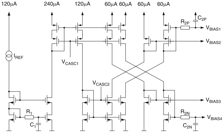
Fig. 5.4 Low-noise biasing
