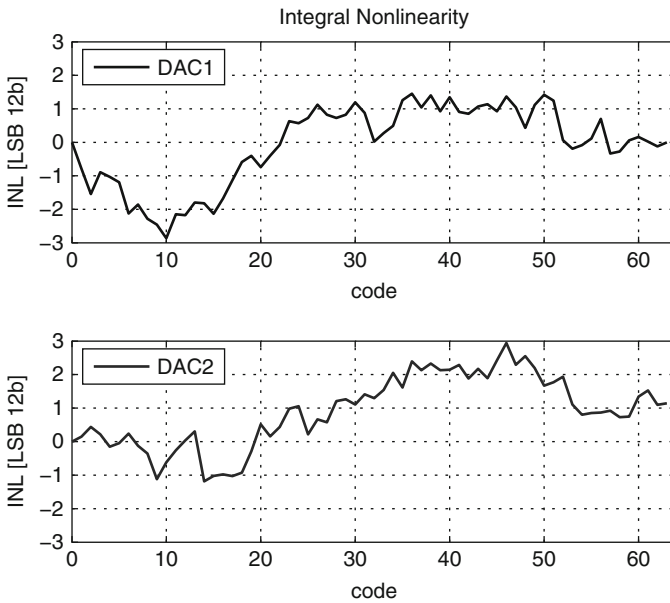
Fig. 5.28 INL of interleaved D/A-converter
