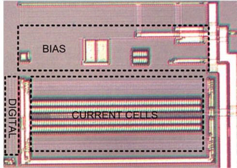
Fig. 6.40 Die photograph of converter core
