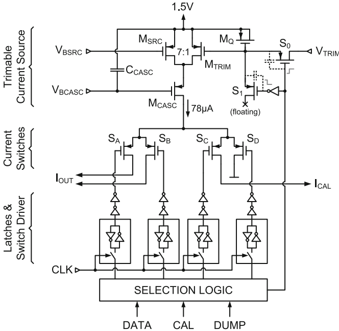
Fig. 6.2 Trimmable PMOS current cell
