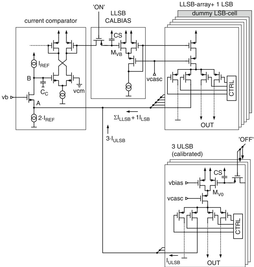
Fig. 6.10 Calibration of the LLSB-array
