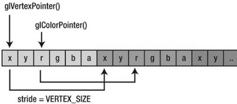
Figure 7-8. Our FloatBuffer holding the vertices, start addresses for OpenGL ES from which to read position/color, and stride used to jump to the next position/color
