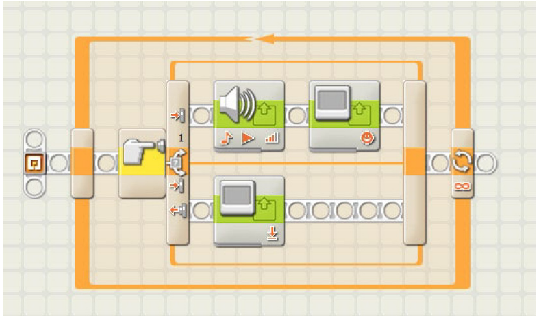
Figure 6-3. Loop block surrounding Switch block logic
