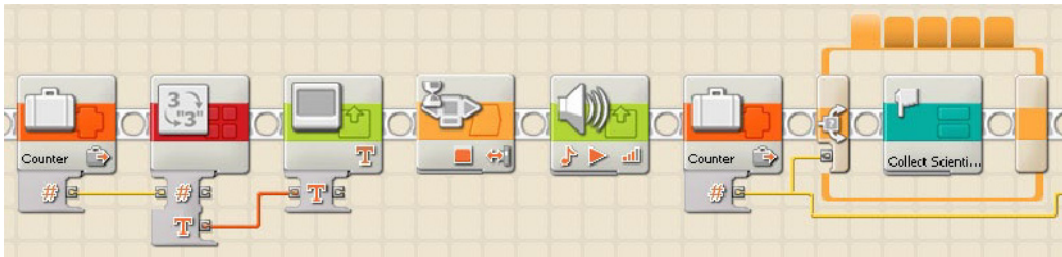
Figure 11-9. A simple sequencer with feedback such as tones and displays
