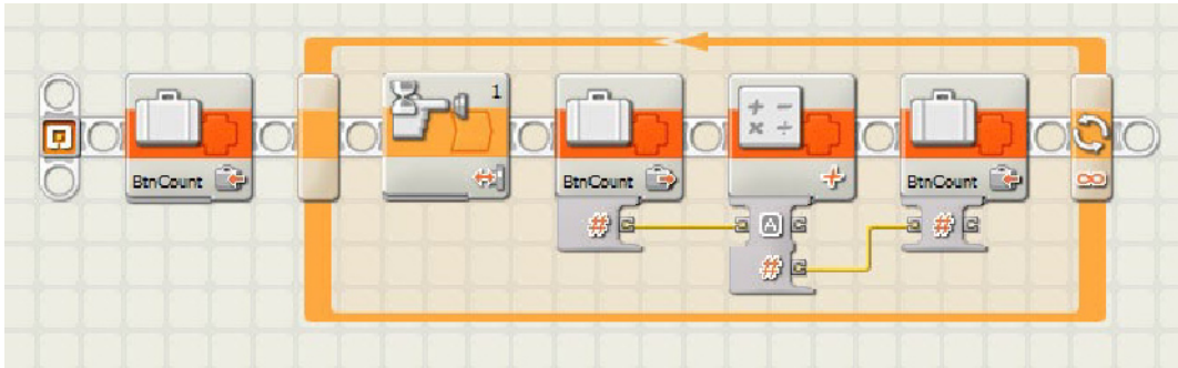
Figure 5-16. Touch counter code sequence
