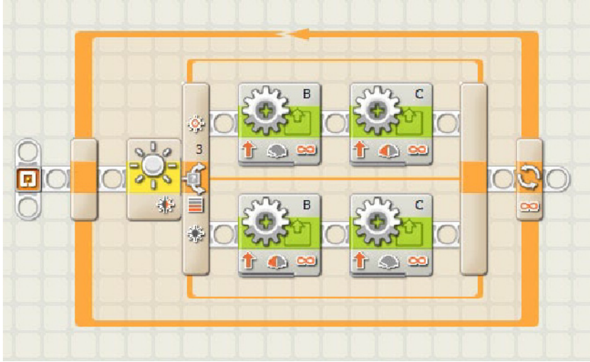
Figure 8-8. A simple line-following program that zigzags back and forth over the line
