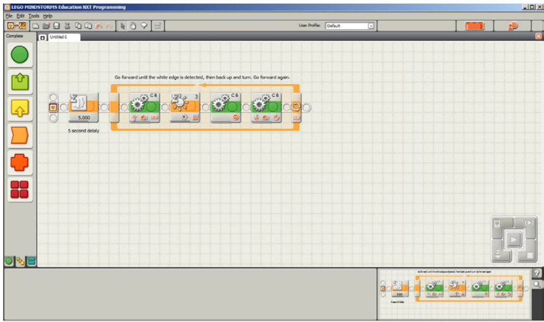
Figure 10-6. A simple Sumo Bot program with edge detection
