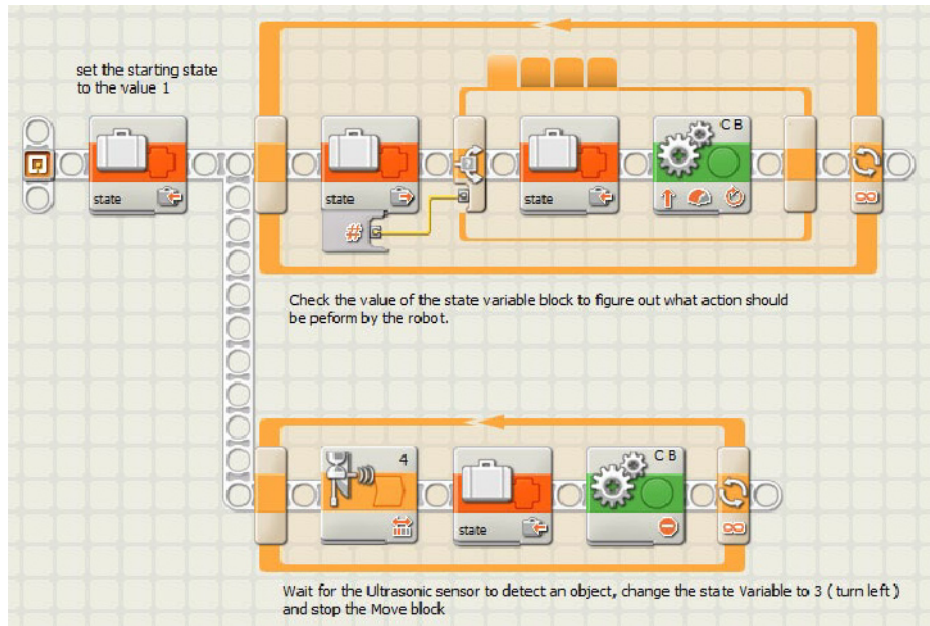
Figure 11-6. A second sequence beam to check the Ultrasonic sensor and change the robot's state to 3 (turn left) if an obstacle is found
