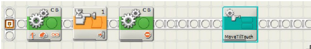
Figure 14-23. Wait For Touch code and My Block
