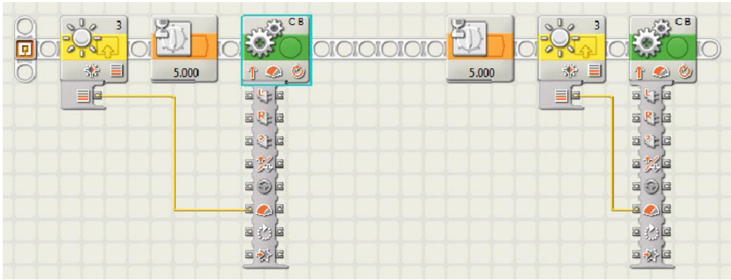
Figure 14-6. Data flow examples
