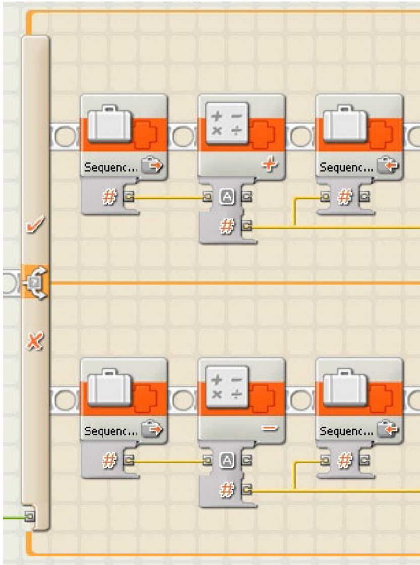
Figure 11-14. A Switch block to test if we need to add or subtract from the sequence value
