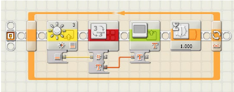
Figure 8-6. A calibrated light value viewer to display the calibrated Light sensor value on the NXT screen
