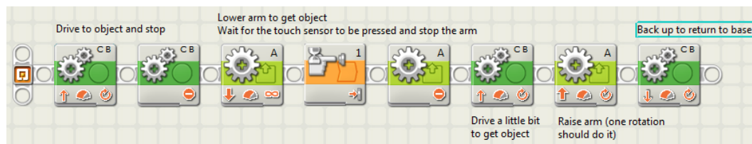
Figure 9-10. Use of a Touch sensor as a Limit switch
