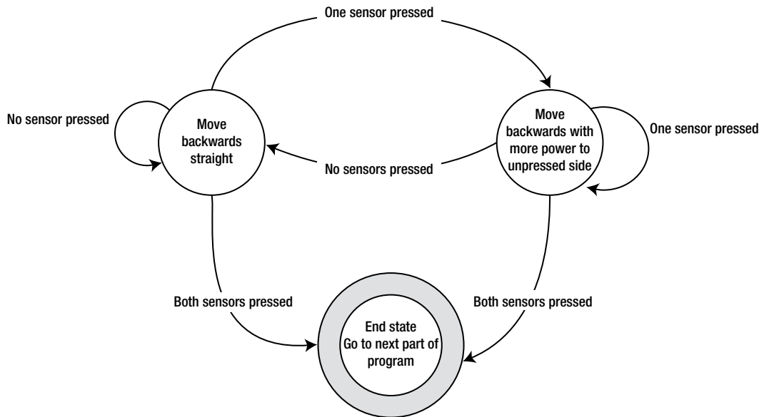
A State machine diagram for squaring
