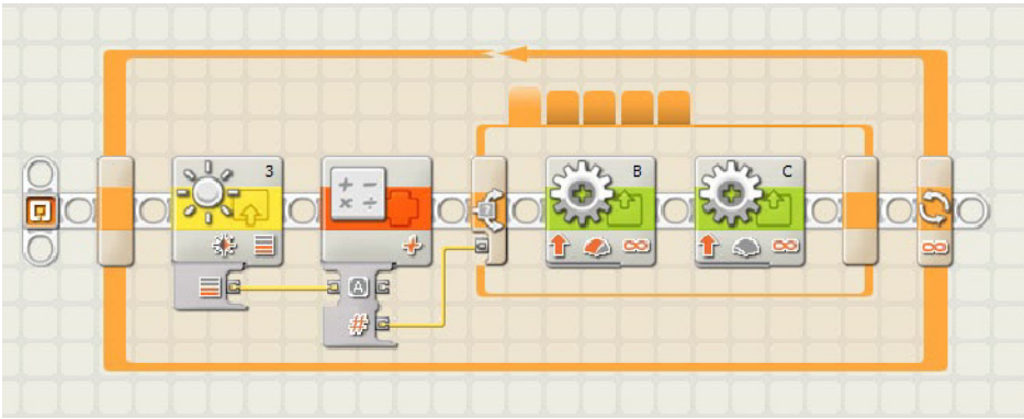
Figure 8-9. Complex condition line-following program with five conditions in the Switch block
