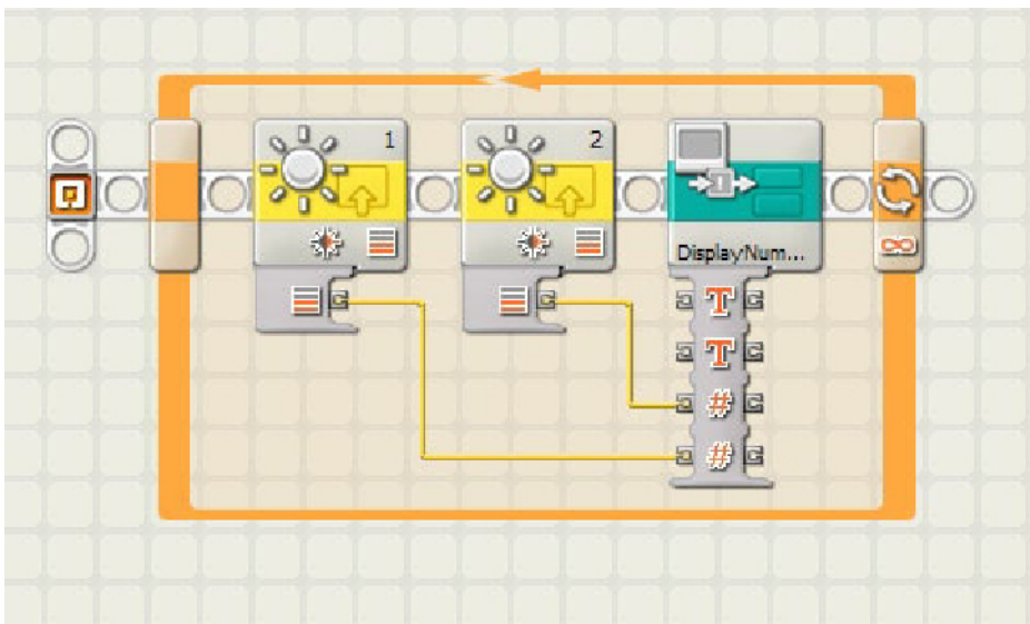
Figure 4-9. DisplayNumber My Block being used to display two Light sensor values
