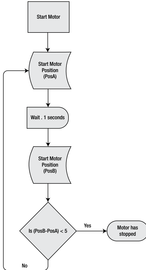
Figure 7-23. Flowchart diagram of the motor stall logic
