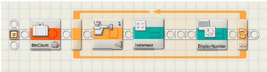
Figure 5-19. New Increment My Block
