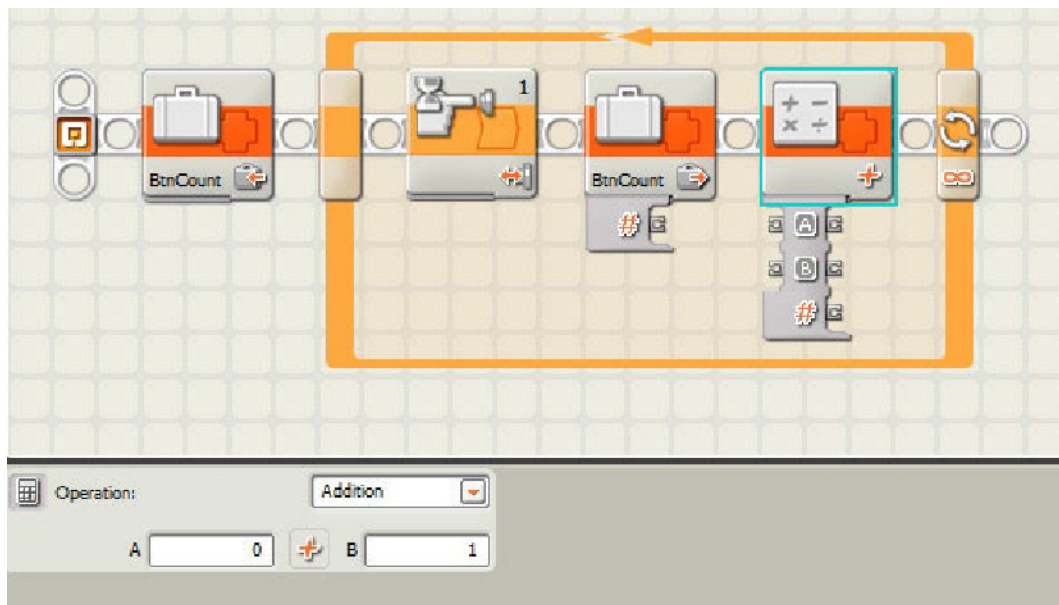
Figure 5-15. Math block added to the code
