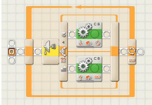
Figure 6-27. A Switch block using an Ultrasonic sensor sample program that will reverse the robot when it approaches a wall
