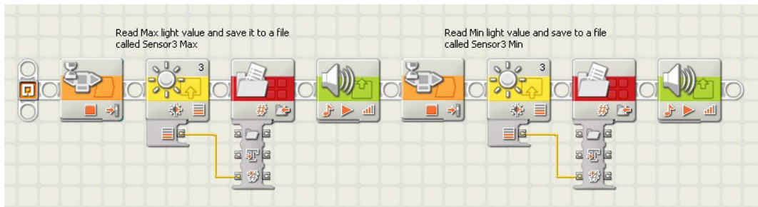
Figure 8-5. An NXT-G calibration program that writes the max and min values to a text file
