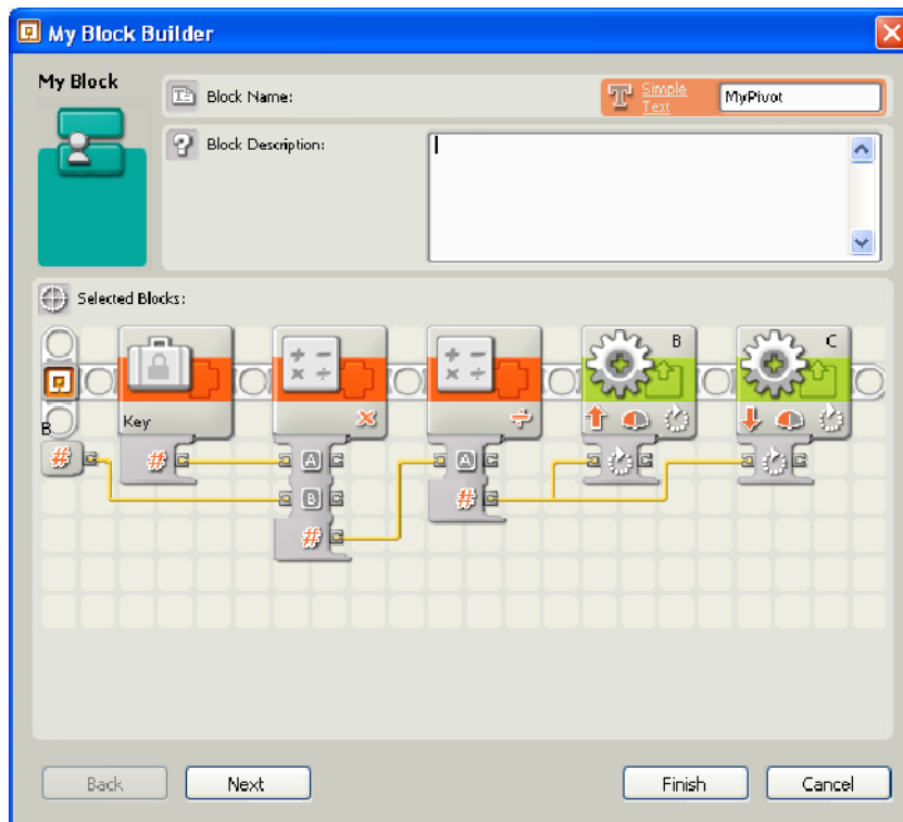
Figure 7-18. The My Block Builder with your code blocks for the MyPivot block. The wired parameter labeled “B” will be your input of degrees
