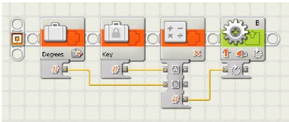
Figure 7-22. The MyTurn block: similar to the MyPivot block but with only one Motor block and a single Math block
