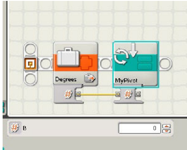
Figure 7-19. Here you can see the new MyPivot block connected to the Variable block that we left out of the MyPivot definition
