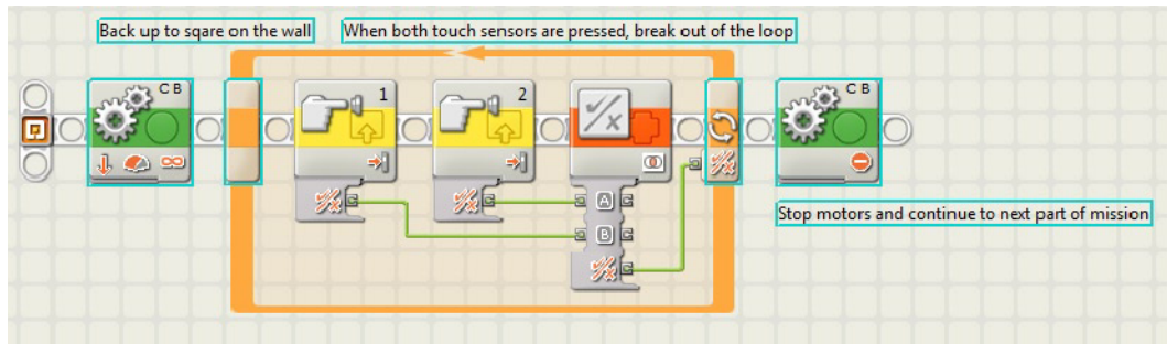
Figure 9-7. A program to square the robot by driving backward until both Touch sensors are pressed
