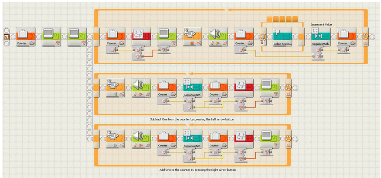
Figure 11-17. Revised master program with the new SequenceMath block included
