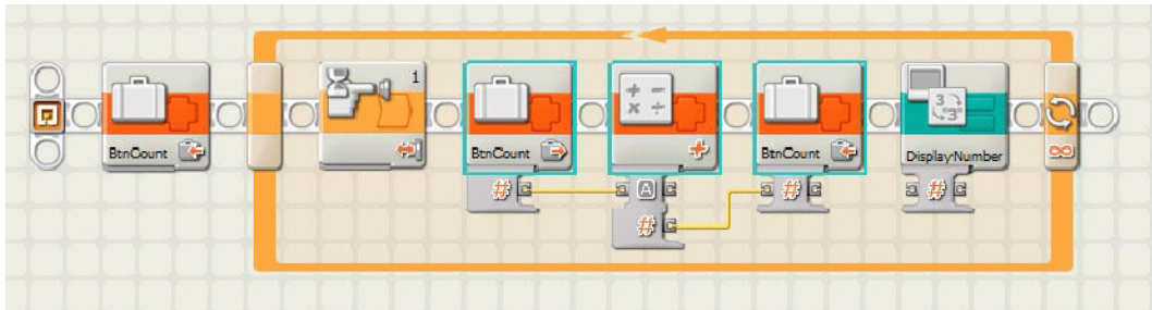
Figure 5-18. Select the counting logic
