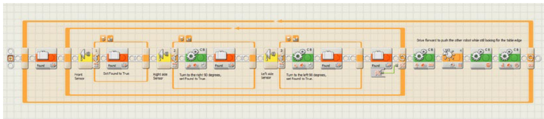
Figure 10-13. A Sumo Bot program using three Ultrasonic sensors
