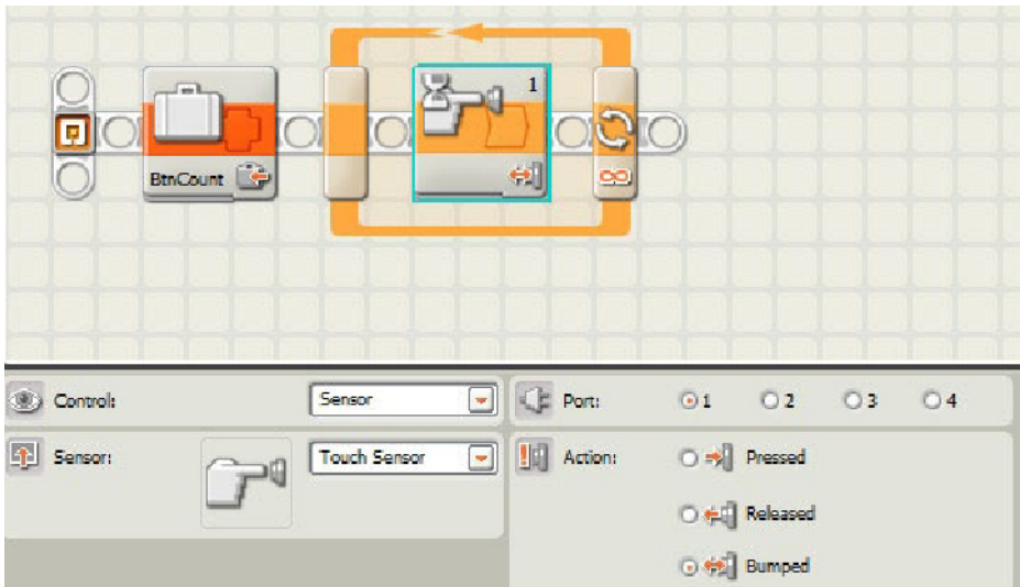
Figure 5-14. Touch sensor Wait inside the Loop
