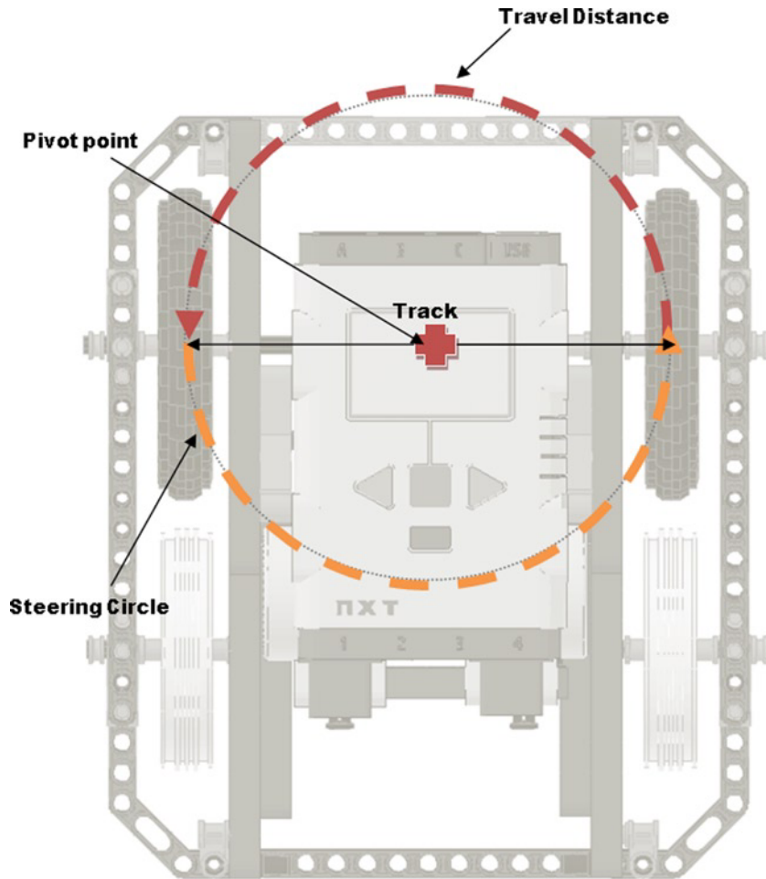
Figure 7-13. A robot making a 180-degree pivot turn with both motors would create a steering circle with the diameter being that of the robot's track. The center of the steering circle would be the center point of the robot track
