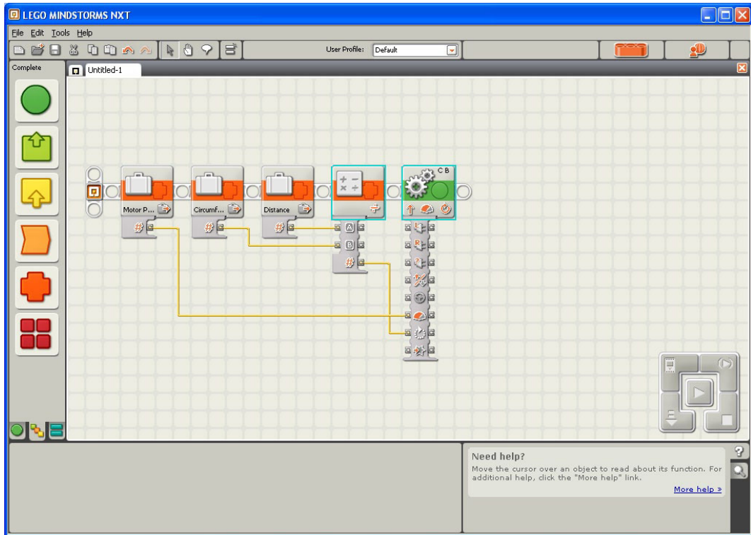
Figure 7-6. Highlighting just the Math and Move blocks—the variables are left out so that they become parameters for your MyMove block
