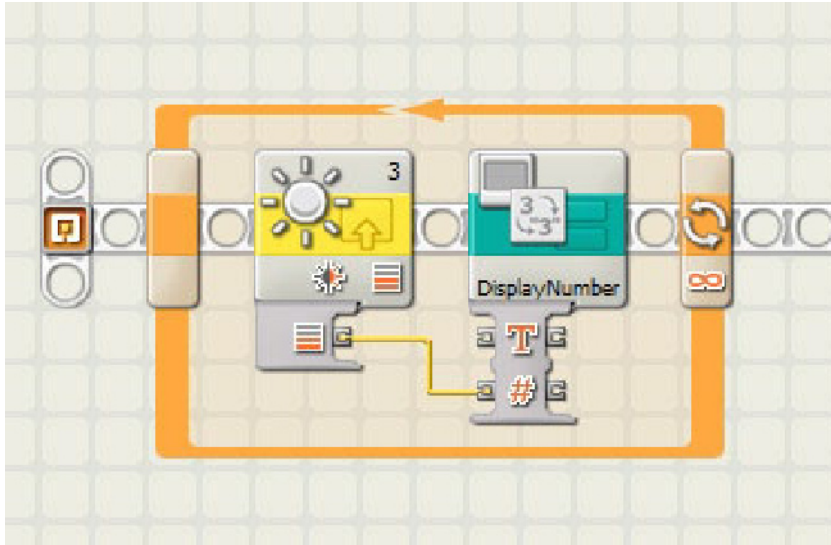
Figure 4-7. DisplayNumber My Block included in code
