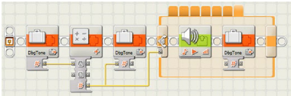
Figure 14-10. DebugTone My Block code
