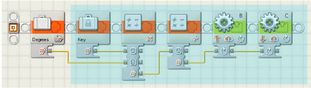
Figure 7-17. Selected blocks that will be a part of your new MyPivot block
