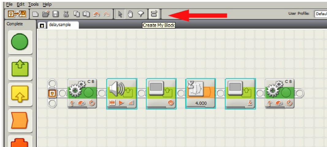
Figure 3-4. Selected blocks to make new My Block. Notice the cyan borders around the selected blocks
