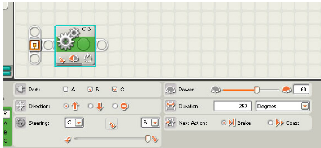
Figure 7-14. A Move block being set to pivot the robot 180-degrees by using a value of 257.4 as the Duration, and the steering set all the way to the far right
