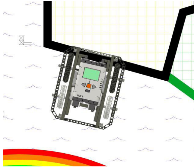
Figure 8-18. The robot then pivots on the first sensor's corner until the second sensor detects the line
