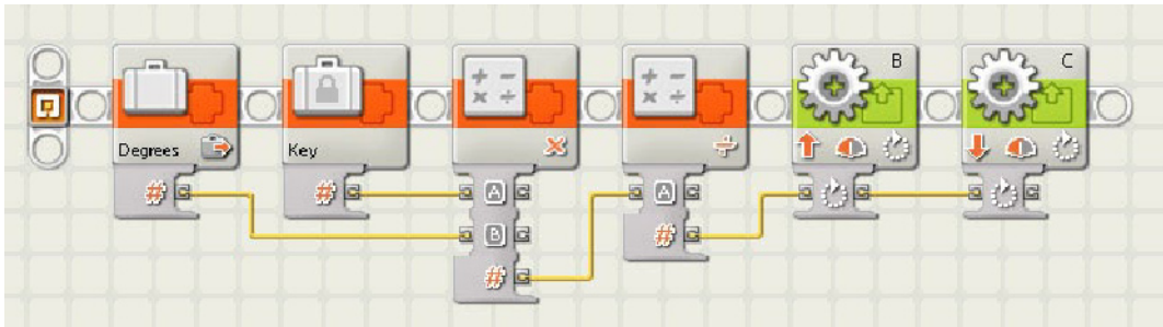
Figure 7-16. The definition of MyPivot block, which allows the user to pass in the desired turn degrees and have the duration calculated automatically
