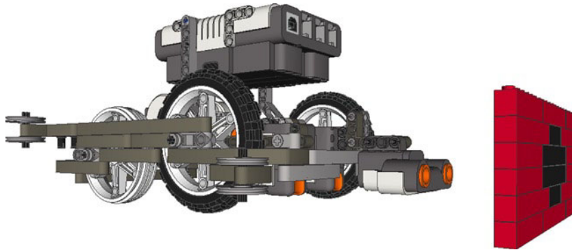
Figure 10-3. A robot with an Ultrasonic sensor that is detecting a sensor wall
