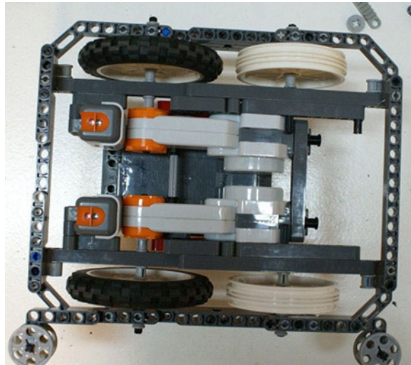
Figure 8-12. A robot with dual Light sensors installed
