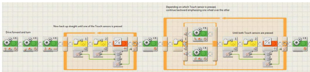
Figure 9-8. An alternate method for squaring the robot
