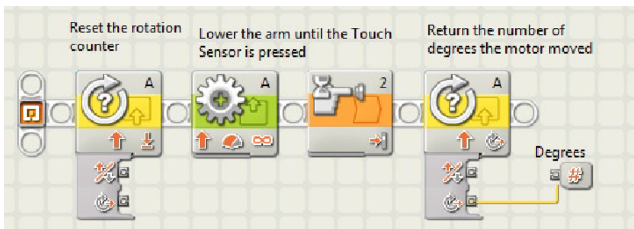
Figure 13-19. My Block to move an arm using a Touch sensor as a Limit switch
