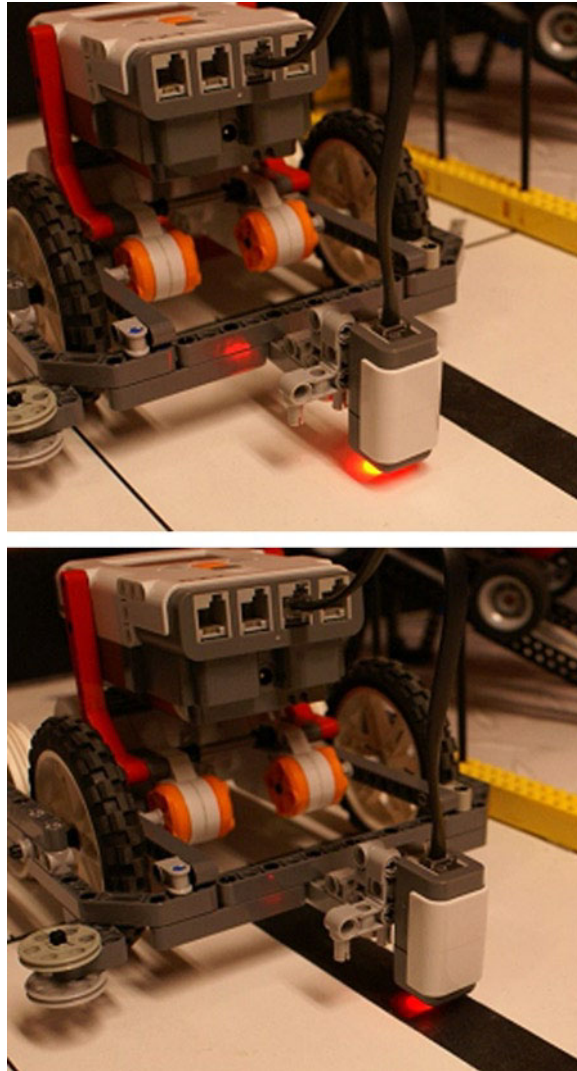
Figure 8-4. Calibrating the Light sensor over a light-colored area and a black line
