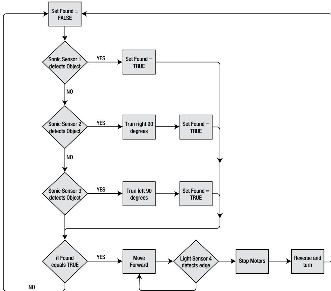
Figure 10-12. A flow diagram mapping out the logic of using three Ultrasonic sensors for a Sumo Bot
