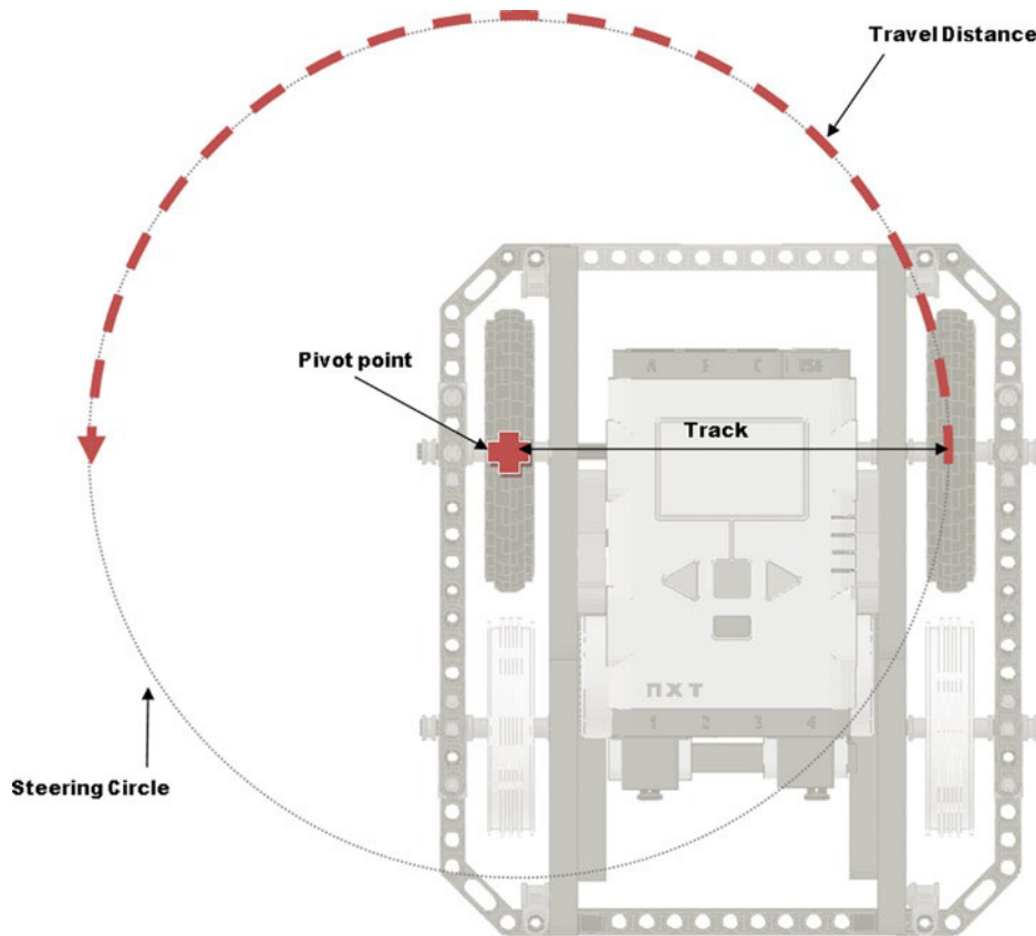
Figure 7-12. Robot making a 180-degree turn with a single motor
