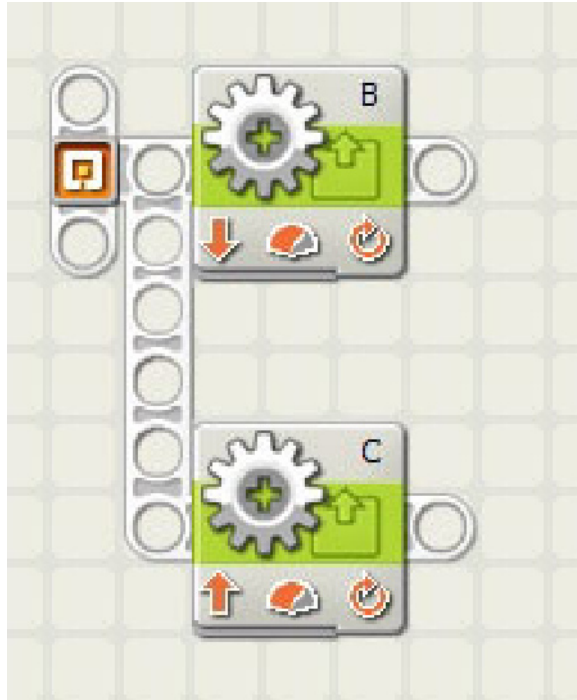
Figure 7-9. Motor blocks on different sequence beams
