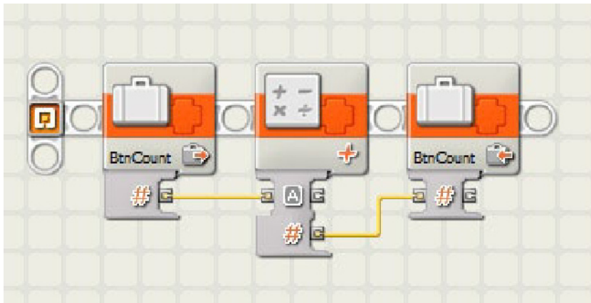
Figure 5-21. Increment My Block code
