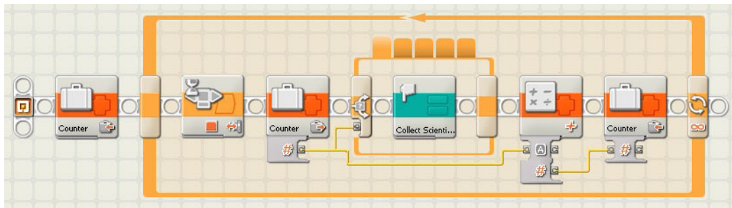
Figure 11-8. A simple sequencer master program
