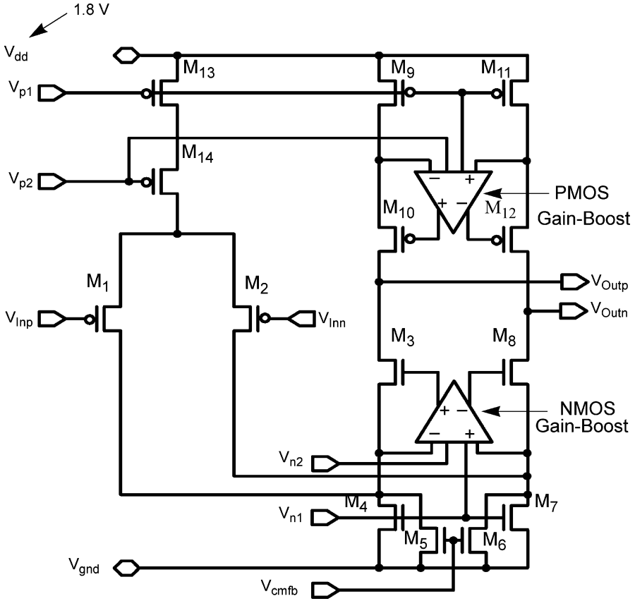
Fig. 5.4 Operational amplifier main stage
