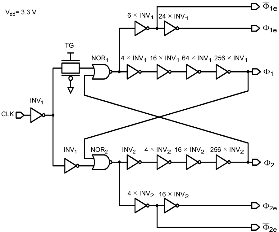
Fig. 5.2 Two-phase nonoverlapping clock generator
