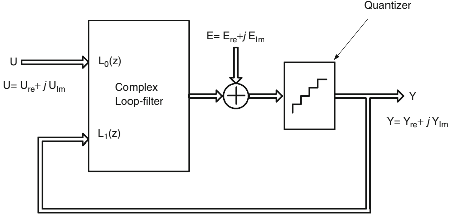
Fig. 3.1 A complex \Delta\Sigma modulator structure
