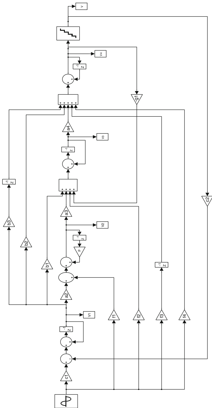
Fig. A.6 Simulink model of the complex \Delta\Sigma modulator
