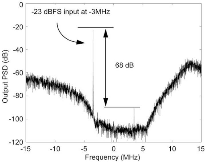
Fig. 5.32 Image rejection measurement with a three-stage polyphase filter at the input of the IC spectrum of the \Delta\Sigma modulator for a -3 MHz input signal. For the input signal frequencies between 2.75 MHz and 4.5 MHz, the image rejection of the \Delta\Sigma ADC was measured as greater than 65 dB.
