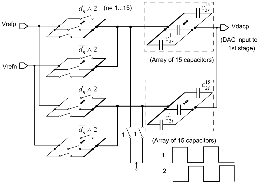
Fig. 4.16 Multi level DAC
