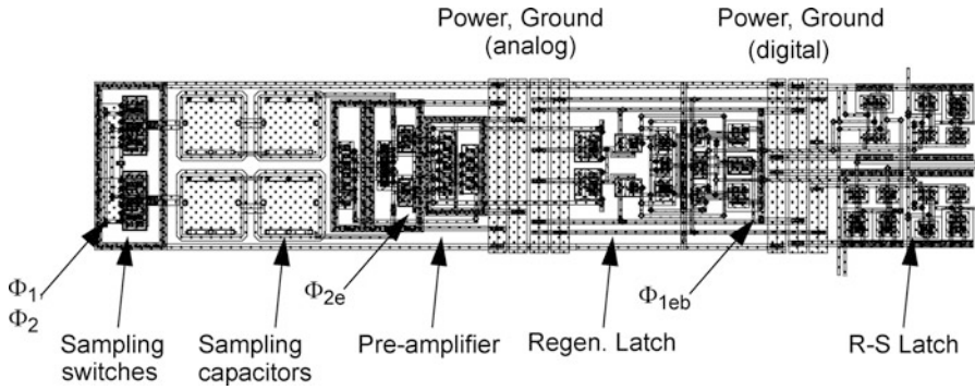
Fig. 5.17 Comparator layout
