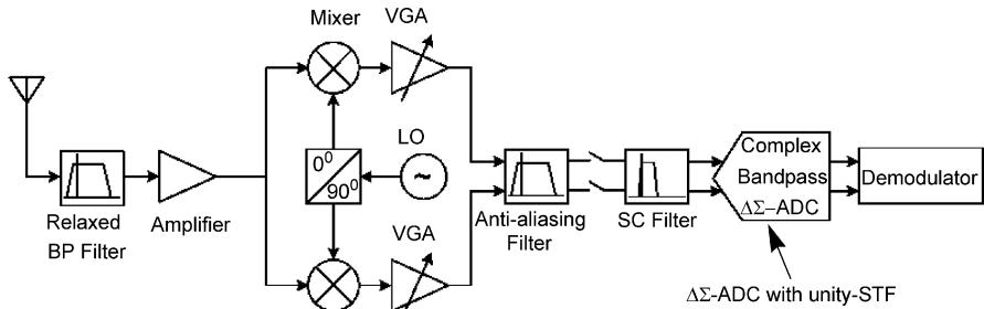
Fig. 3.41 A quadrature-IF system using a complex Low-IF \Delta\Sigma modulator and a SC filter for channel filtering and selectivity
