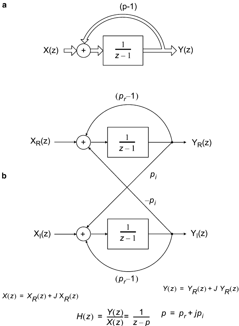
Fig. 4.1 Realizing a complex pole at p = p_r + jp_i using (a) a complex signal flow graph and (b) a two-input two-output real linear signal flow graph
