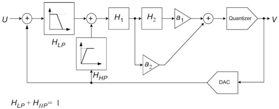
Fig. 2.12 \Delta\Sigma modulator with additional low pass and high pass filters in forward and feedback paths to implement a filtering STF [14]
