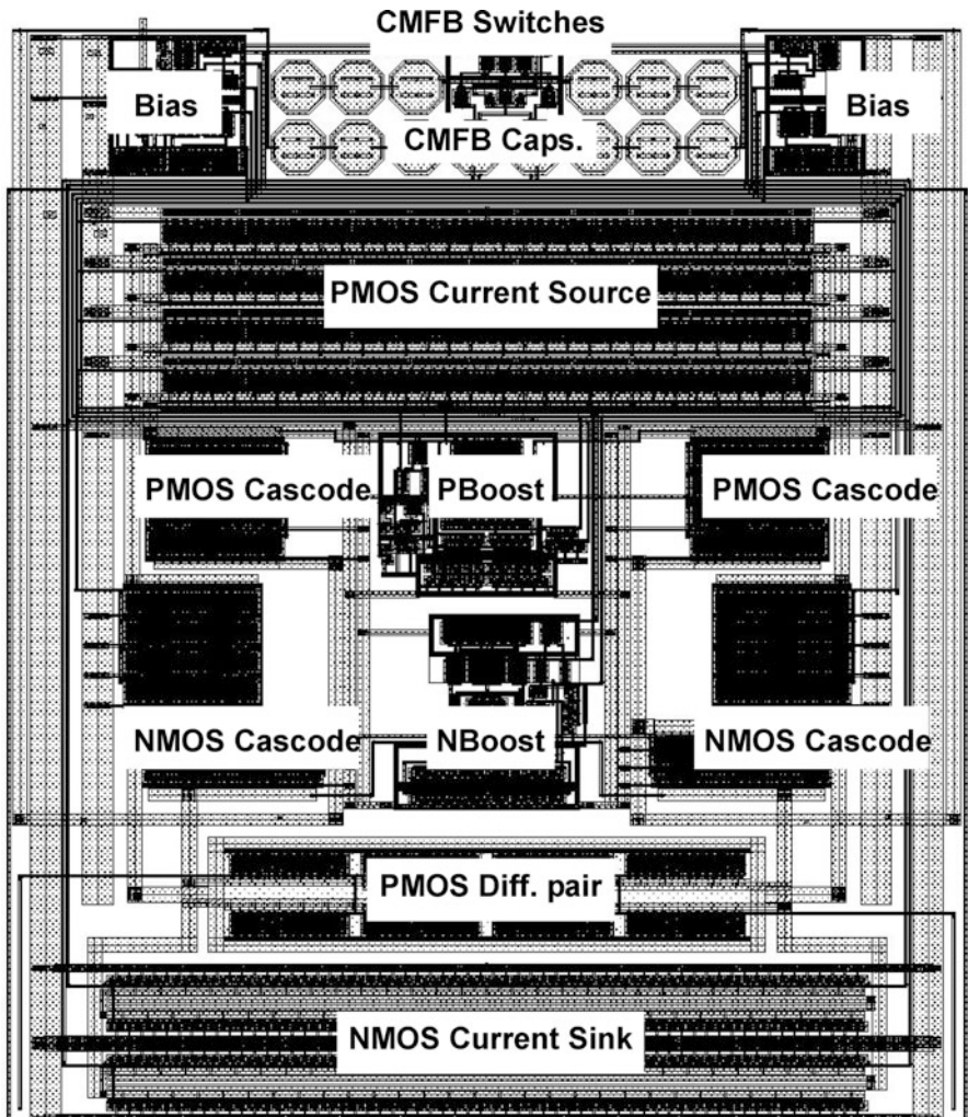
Fig. 5.18 Amplifier layout
