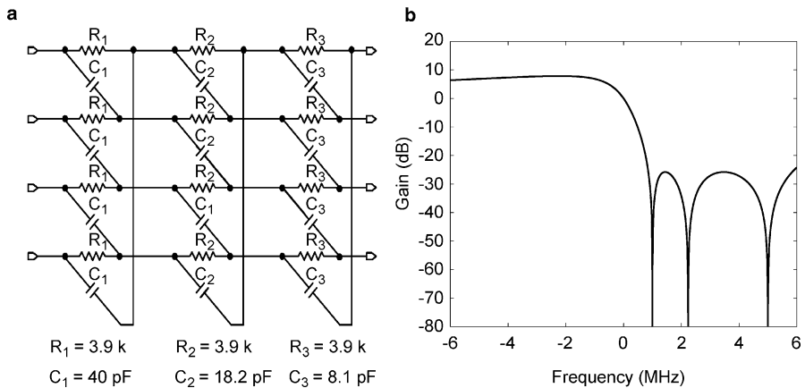
Fig. 5.24 RC Polyphase filter designed to attenuate the image at the input of the test chip: (a) circuit diagram showing the component values, (b) frequency response of the three-stage polyphase filter
