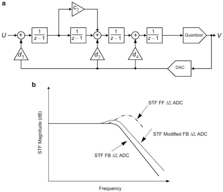
Fig. 2.11 (a) Modified feedback \Delta\Sigma modulator [13], (b) STFs for the modulator architectures
