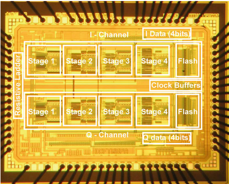
Fig. 5.20 Microphotograph of the fourth-order \Delta\Sigma modulator
