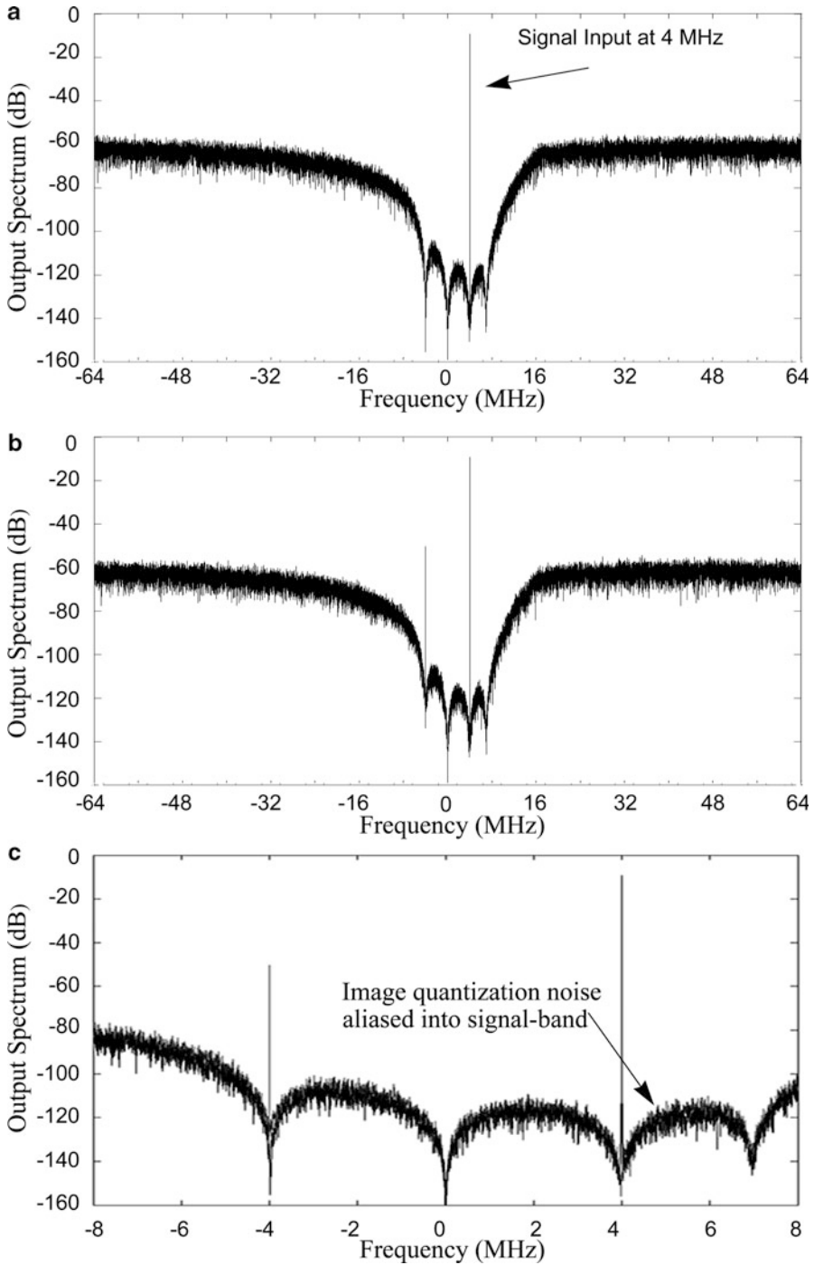
Fig. 4.11 Output spectrum of the modified modulator: (a) Ideal spectrum, (b) with 0.5% mismatch, (c) Zoom-in of image quantization aliased into signal-band
