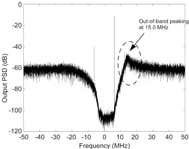
Fig. 5.34 Output PSD measured with -3 dBFS input at a sampling frequency of 100 MHz
