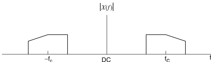
Fig. 2.1 Spectrum of a bandpass signal
