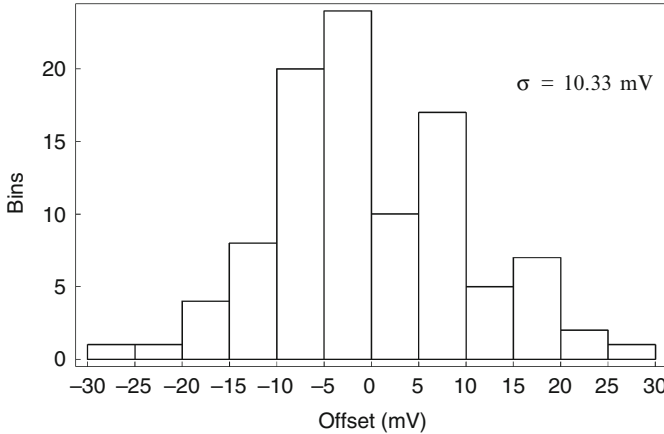
Fig. 5.13 Result of the Monte Carlo transient simulation performed to determine the input-referred offset of the comparator
