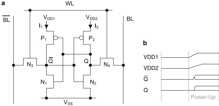
Fig. 10.24 Preselection using V_{DD} pins (a) Schematic. E med ; (b) Timing diagram
