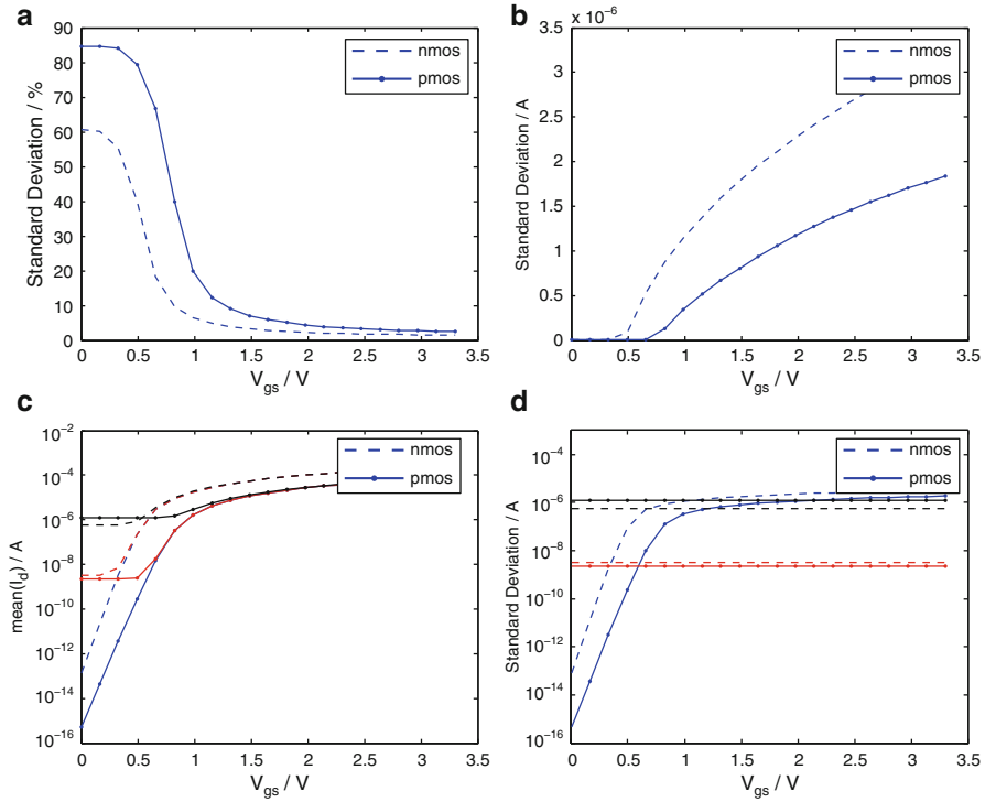
Fig. 6.10 Influence of mismatch at different V_{GS} : (a) Standard deviation of I_D in %. (b) Standard deviation of I_D in A. (c) Mean I_D noiseless (blue), noisy (1 Hz–1 GHz) (red), noisy (1 Hz–100 GHz) (black). (d) Std I_D (blue), RMS noise (1 Hz–1 GHz) (red), RMS noise (1 Hz–100 GHz) (black)
