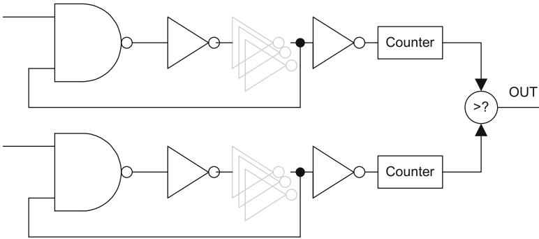
Fig. 1.8 Ring oscillator PUF
