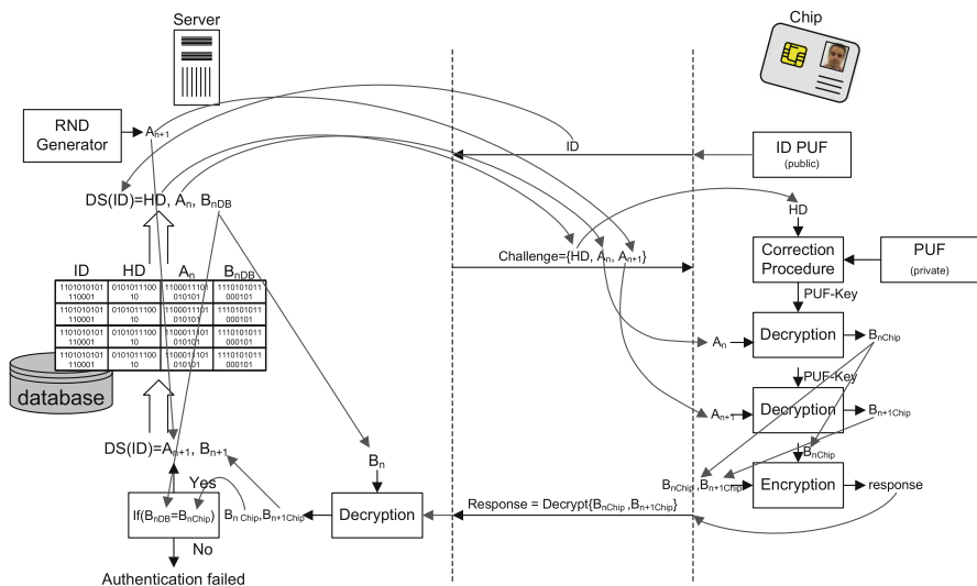
Fig. 3.15 Dynamic CRP updating: authentication phase
