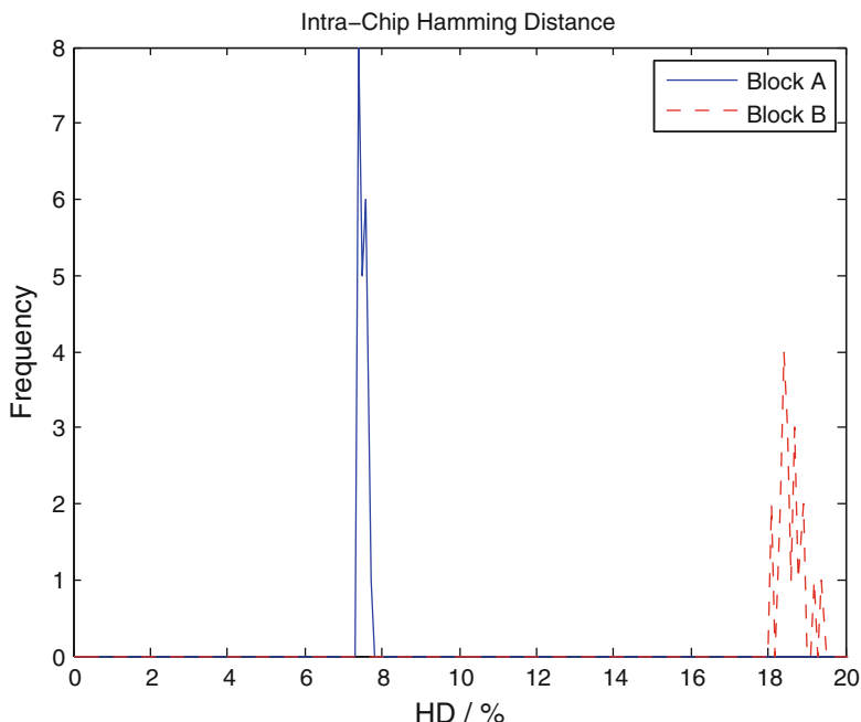
Fig. 15.6 Hamming distance of block A and block B at room temperature
