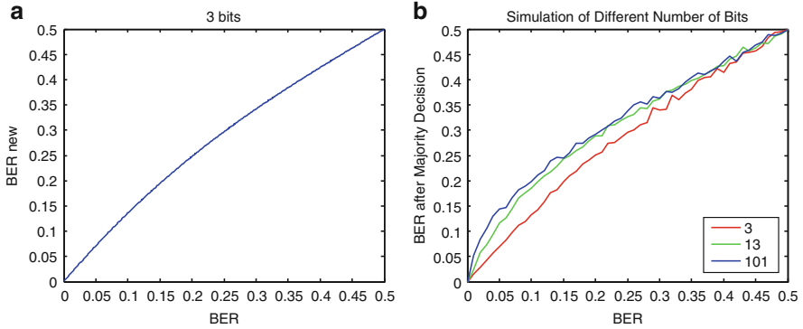
Fig. 5.5 BER after combining: (a) Calculation; (b) Simulation results
