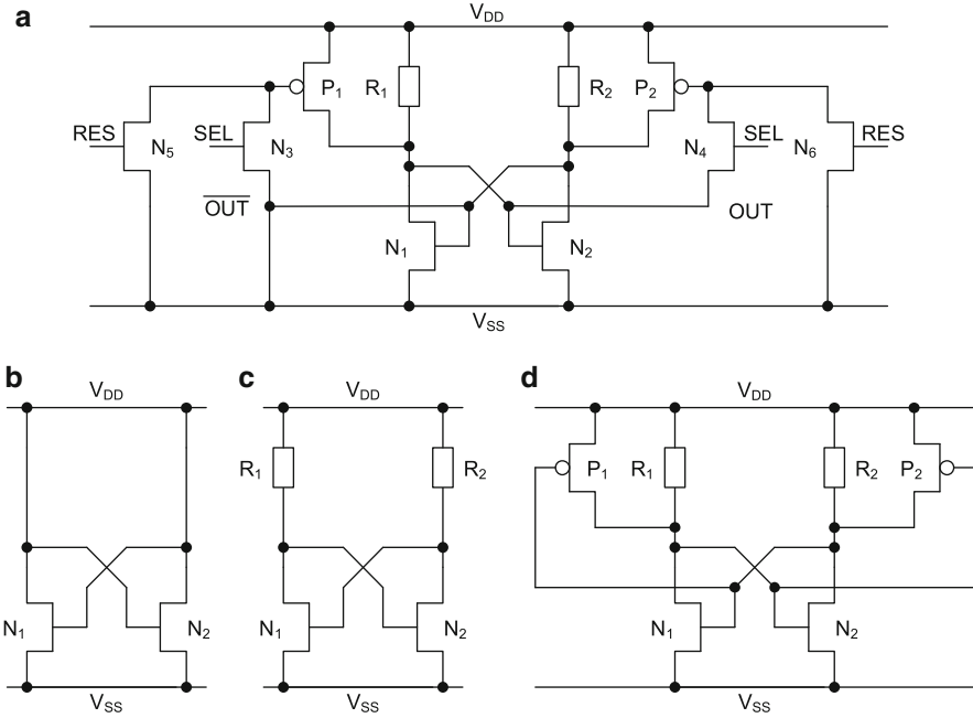
Fig. 6.21 Resistor-based PUF: (a) Complete circuit; (b) Reset; (c) Amplification; (d) Evaluation
