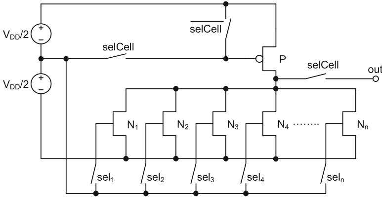
Fig. 1.13 Inverter-based PUF
