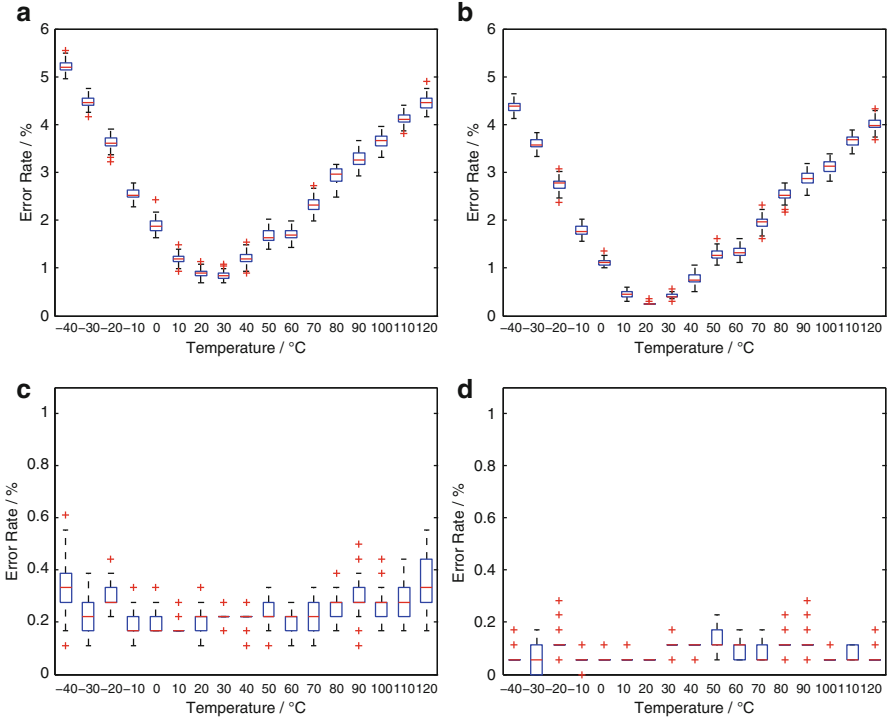
Fig. 13.10 BER of preselection multiple readout in dependence of the temperature (a) 1 temperature, 10 readouts; (b) 1 temperature, 50 readouts; (c) 3 temperature, 10 readouts (d) 3 temperature, 50 readouts
