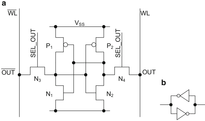
Fig. 1.17 (a) Regular 6T-SRAM cell; (b) Equivalent circuit
