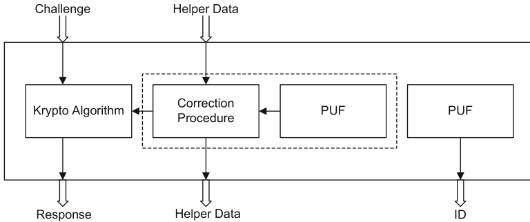
Fig. 3.11 Authentication with the software-based CRPs
