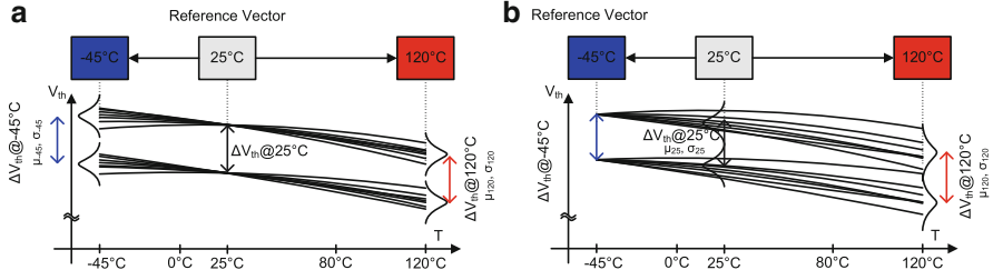
Fig. 4.1 Enrollment at different temperatures; (a) Enrollment at 25 °C; (b) Enrollment at -45 °C
