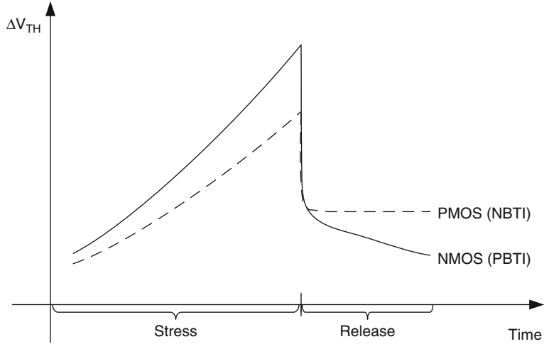
Fig. 6.5 The above figure shows the change in threshold voltage of an NMOST and a PMOST if the transistors are stressed for a certain time. After the stress the original V_{TH} is partly recovered [13]
