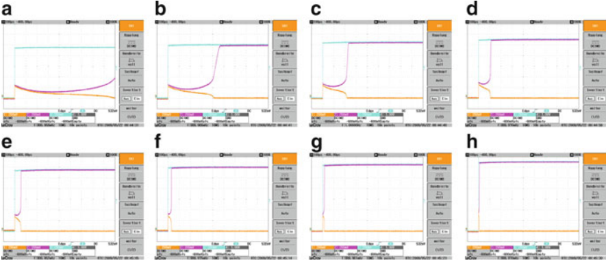
Fig. 1.19 The figure shows the decision process of a discrete implemented SRAM cell applying different supply voltages: (a) V_{DD} = 0.95 V; (b) V_{DD} = 1 V; (c) V_{DD} = 1.05 V; (d) V_{DD} = 1.1 V; (e) V_{DD} = 1.15 V; (f) V_{DD} = 1.2 V; (g) V_{DD} = 1.25 V; (h) V_{DD} = 1.3 V
