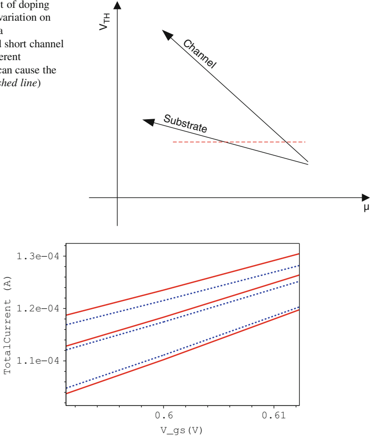
Fig. 7.8 TCAD: Current output of two different transistors at three different temperatures (bottom-up: -50^{\circ}\text{C} , 27^{\circ}\text{C} , 120^{\circ}\text{C} ). At -50^{\circ}\text{C} , the sign of the ratio between the currents changes which would lead to an erroneous PUF-cell output
