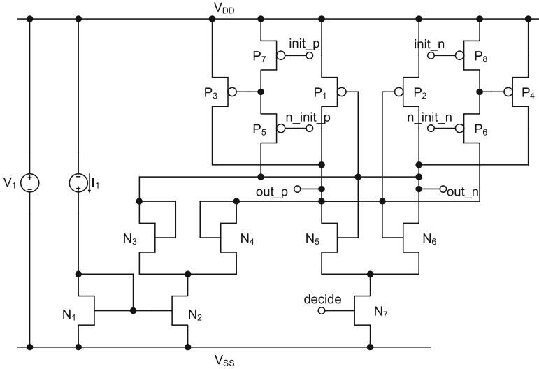
Fig. 10.13 Implementation example of an SRAM-like PUF with preselection transistors P_3 and P_4
