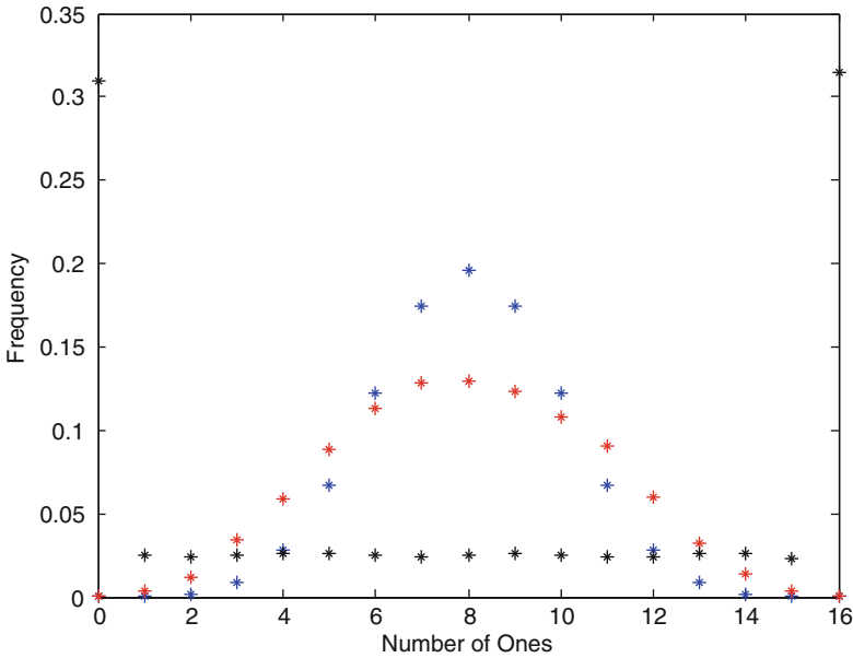
Fig. 13.6 Ideal ( blue ) distribution of ones in a block of 16 output bits. Small ( red ) and strong ( black ) influence of SA mismatch
