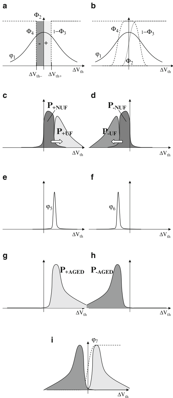
Fig. 11.7 (a) Ideal distributions \Phi_1 - \Phi_4 ; (b) Real distributions \Phi_1 - \Phi_4 ; (c) Useful positive PUF-cells(UF+); (d) Useful negative PUF-cells(UF-); (e) Positive increase \phi_5 ; (f) Negative increase \phi_6 ; (g) Positive increased area P_{+AGED} ; (h) Negative increased area P_{-AGED} ; (i) Distribution of all cells
