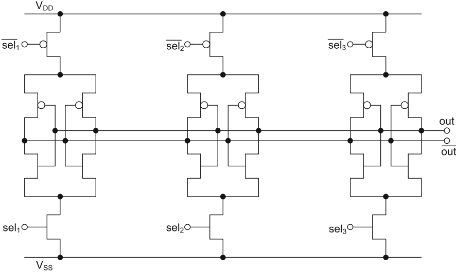
Fig. 9.8 Practical realization of majority parallelization
