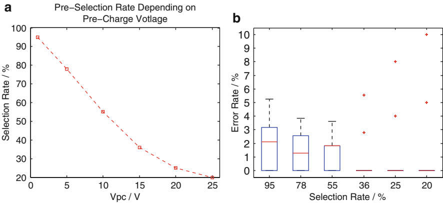
Fig. 10.28 Simulation results BLPS (a) Preselection rate vs pre-charge voltage; (b) Error rate vs preselection rate
