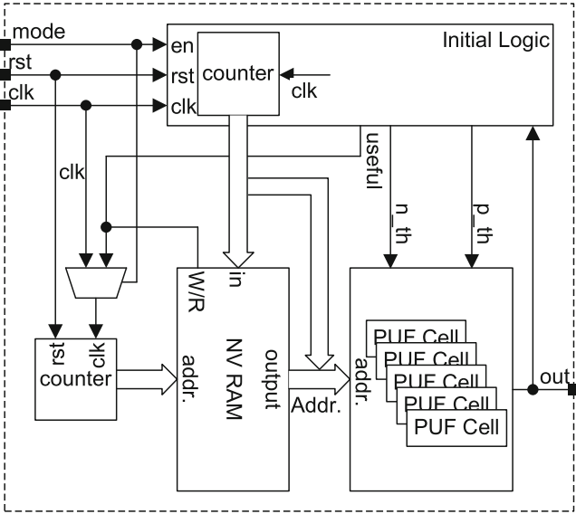
Fig. 10.15 Diagram of PUF system including preselection
