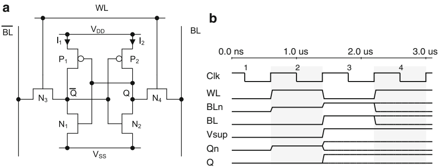
Fig. 10.26 Preselection using BL pins (a) Schematic. E_{med} ; (b) Timing diagram
