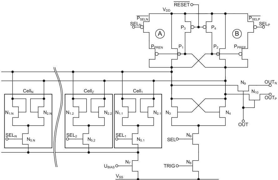
Fig. 14.10 Circuit with preselection and shared sense amplifier
