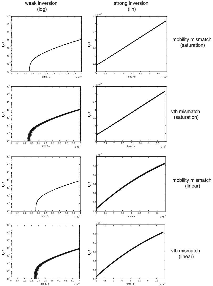
Fig. 6.11 The influence of \mu and V_{TH} variability on I_D is shown for different regions of operation. It illustrates the dominant effect of V_{TH} variability on circuit mismatch. The data are from simulation using the BSIM3 model
