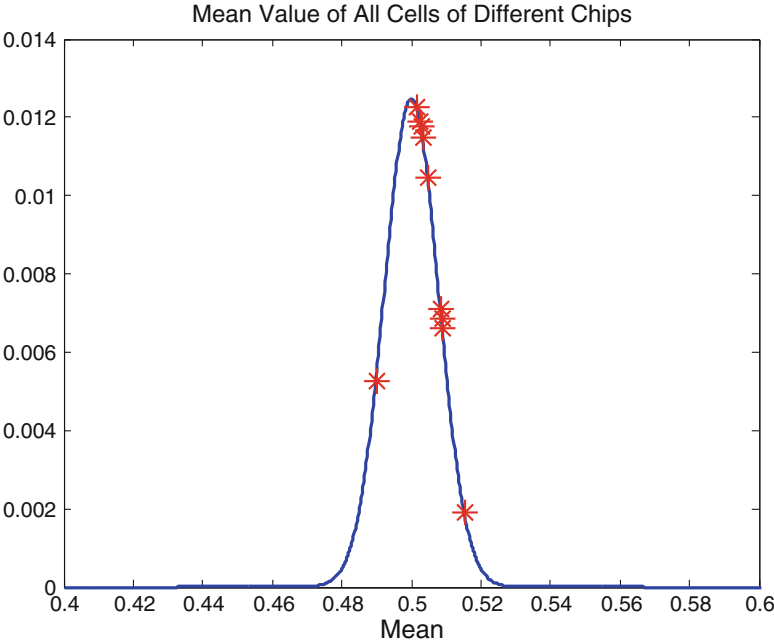
Fig. 12.4 Mean value \bar{x} of the different chips of the two-stage PUF
