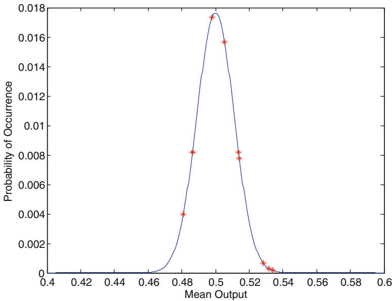
Fig. 13.3 Mean values of the different chips (PUF with shared sense amplifier)
