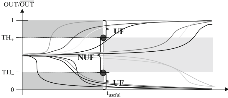
Fig. 10.17 Decision phase of PUF cells
