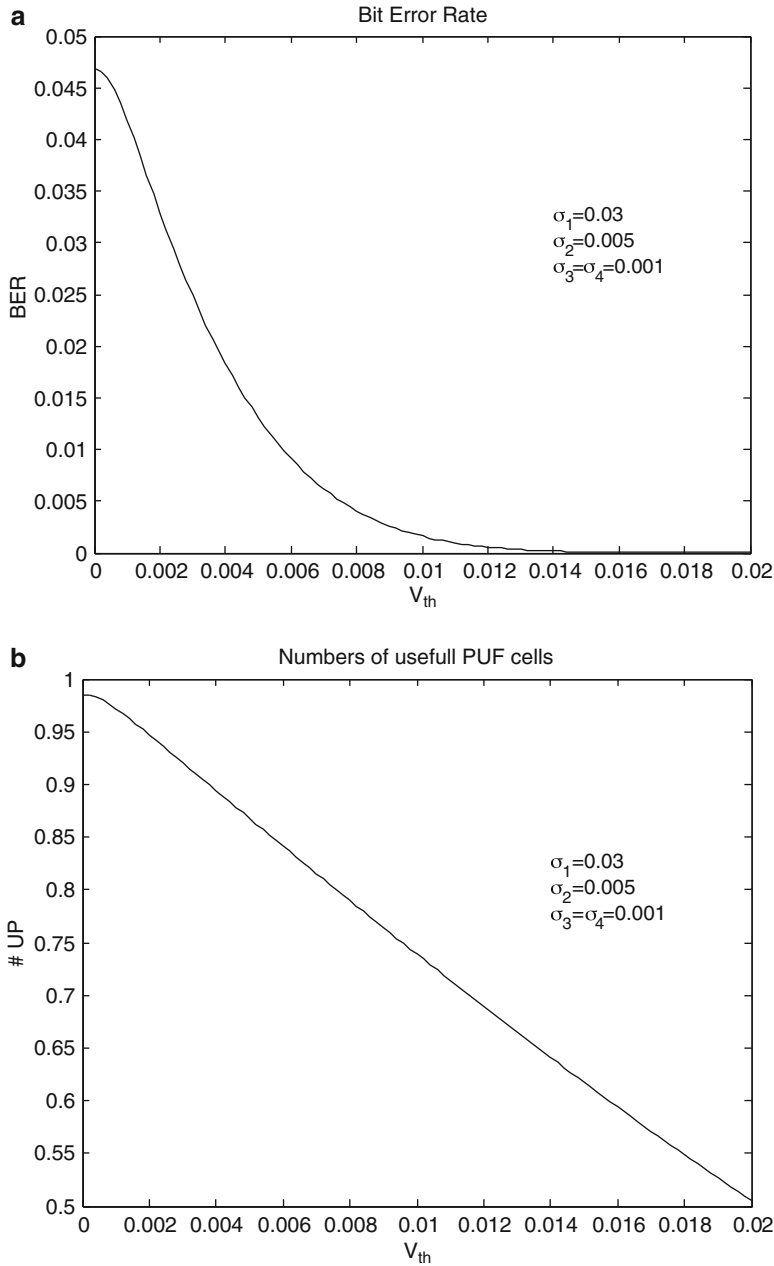
Fig. 10.10 Influence of the preselection threshold value ( \mu_{3,4} ): (a) On error rate e ; (b) On ratio of useful PUF-cells \alpha
