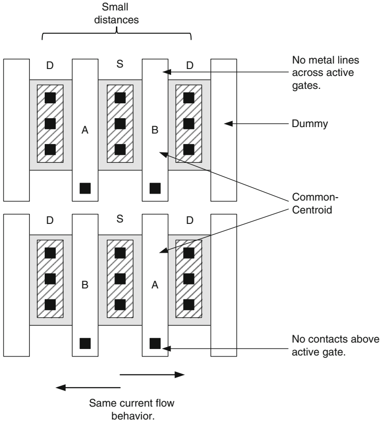
Fig. 6.9 Some of the basic layout rules are shown to minimize the effect of the global mismatches on a pair of transistors
