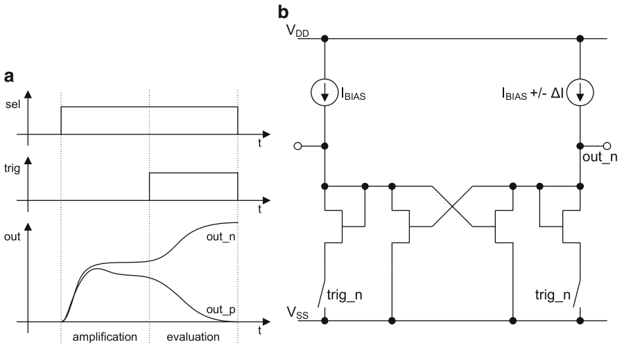
Fig. 12.2 Two stage PUF (a) Timing diagram; (b) Concept
