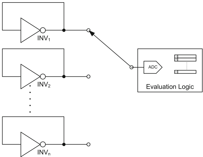
Fig. 1.24 Example of identification cell from [86]
