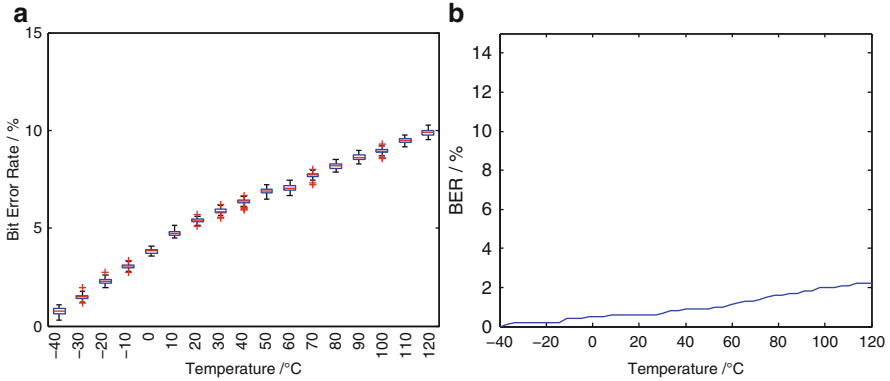
Fig. 7.1 Huge differences between the BER vs. temperature of a real chip (a) and a simulated circuit (b). The reference vector was chosen at -40^{\circ}\text{C}
