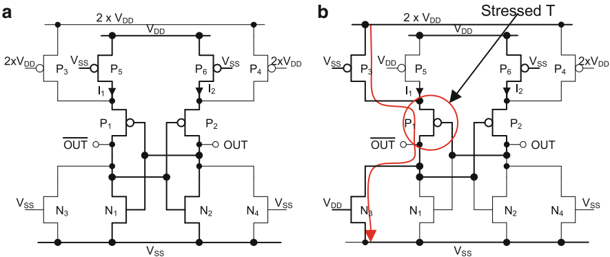
Fig. 11.11 (a) Circuit to stress the transistors with HCI; (b) Ageing of the cell
