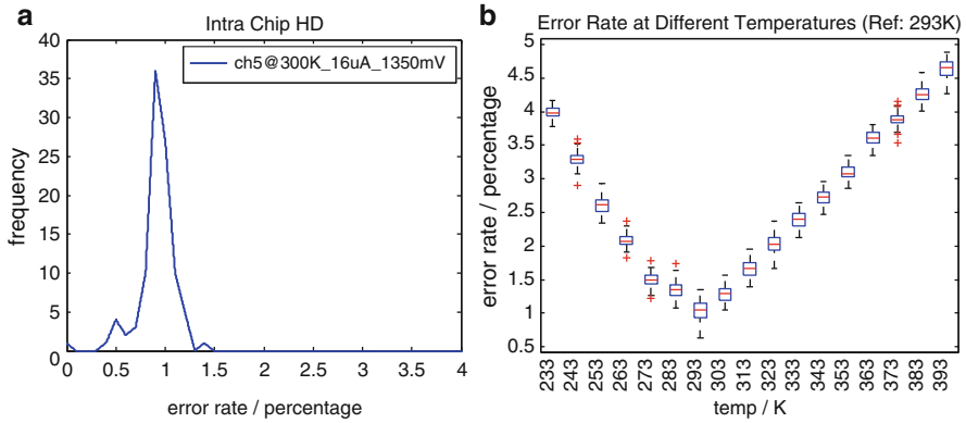
Fig. 4.4 Error rate of PUFs: (a) Intra-chip Hamming distance HD_{intra} at room temperature; (b) HD_{intra} at different temperatures
