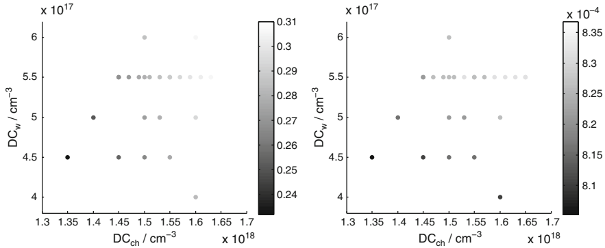
Fig. 7.11 (a) V_{TH} (gray scale) vs channel and well doping concentration. (b) \frac{dV_{TH}}{dT} (gray scale) vs channel and well doping concentration
