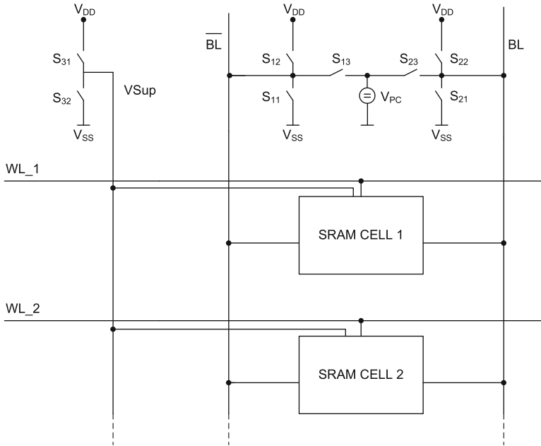
Fig. 10.27 The concept of preselection using BL pins
