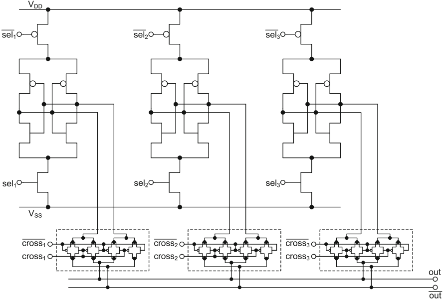
Fig. 9.7 Practical realization of full parallelization
