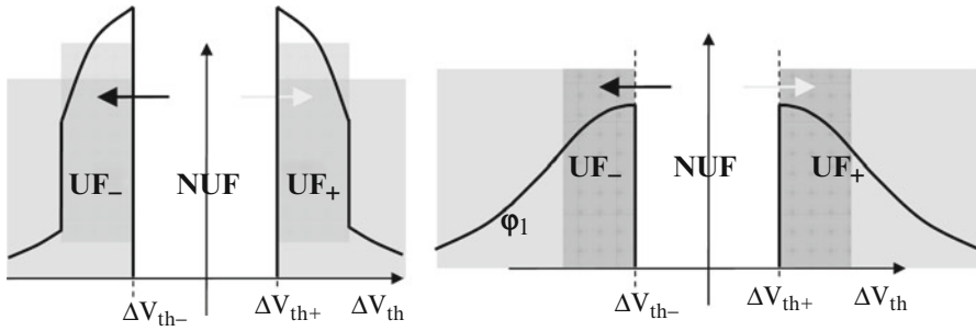
Fig. 11.2 (a) Increase the mismatch of only useless PUF cells; (b) Increase the mismatch of all cells
