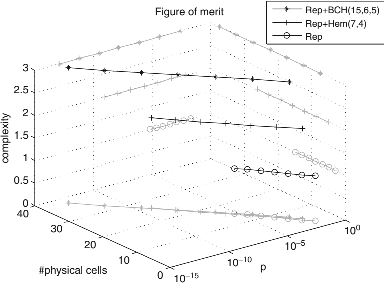
Fig. 5.10 The figure of merit shows the relation between complexity of the ECCs, the number of required PUF-cells and the error rate
