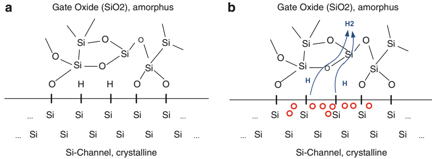
Fig. 6.3 Example of channel-oxide interface with H atoms at the boundary (a). If negative bias voltage is applied, charge carriers (holes (o)) weaken bonds and H 2 molecules diffuse (b). (Inspired by [1])
