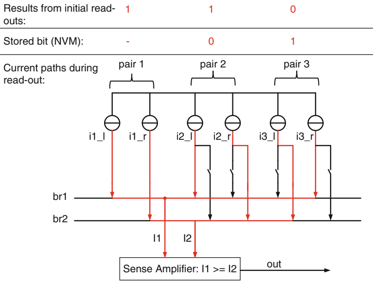
Fig. 9.6 Read-out using the data stored in the NVM
