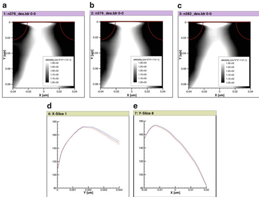
Fig. 7.16 Electron Mobility vs DC_{ch} at -73^{\circ}\text{C} : (a) nominal (green), (b) low (blue), (c) high (red). (d) Y-cut @ x = -0.001\ \mu\text{m} , (e) X-cut @ y = 0.002\ \mu\text{m}
