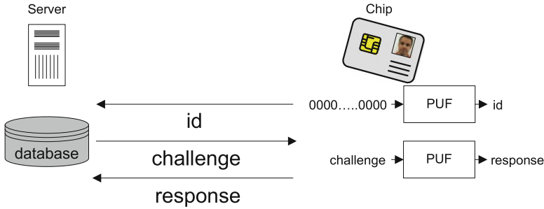
Fig. 3.10 Authentication with hardware-based CRP generation
