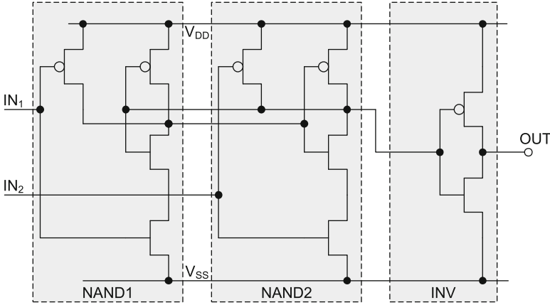
Fig. 10.22 Arbiter transistor level
