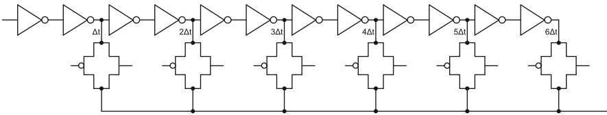
Fig. 10.19 Delay line
