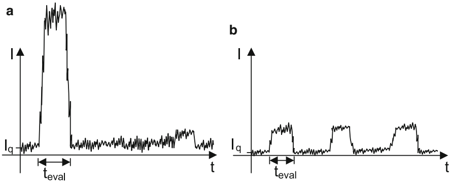
Fig. 4.9 Power consumption: (a) Parallel read-out; (b) Serial read-out
