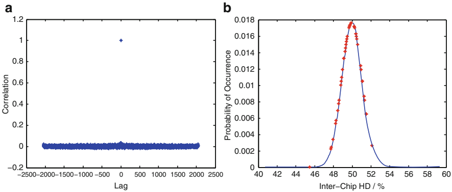
Fig. 13.5 PUF with shared sense amplifier: (a) Correlation between bits; (b) Correlation between chips
