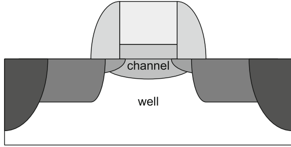
Fig. 7.6 For short channel transistors, the halo implants touch/overlap and a homogeneous channel doping concentration is formed
