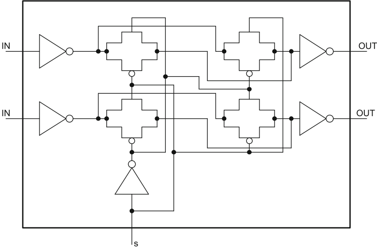
Fig. 1.10 Circuit of a switch box
