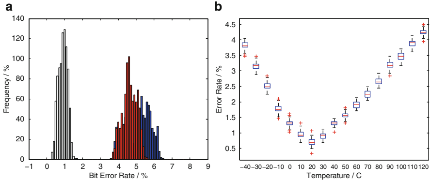
Fig. 14.5 PUF test chip 3: (a) Intra-chip Hamming distance HD_{intra} (100 runs); (b) HD_{intra} at different temperatures
