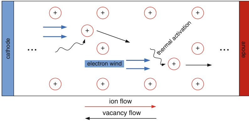
Fig. 6.8 Electromigration happens due to the interaction between electrons and metal atoms. According to the electron wind, the ions flow toward the anode
