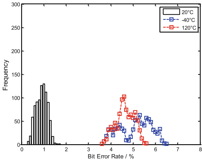
Fig. 7.21 The BER at three different temperatures for different chips is shown. The reference temperature is at 20°C. For -40°C and 120°C the error rate increases up to 7% which is too much for simple error correction codes
