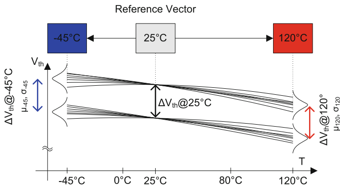
Fig. 4.5 Influence of temperature on the threshold voltage of transistors
