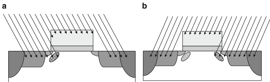
Fig. 7.5 Introducing the halo implant during processing [2]
