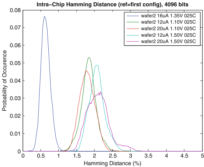
Fig. 4.10 Influence of different currents and voltages
