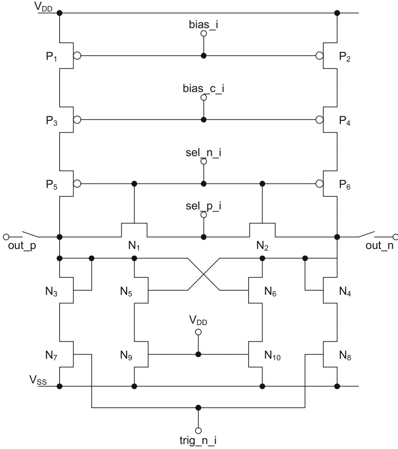
Fig. 12.3 Circuit of the two stage PUF
