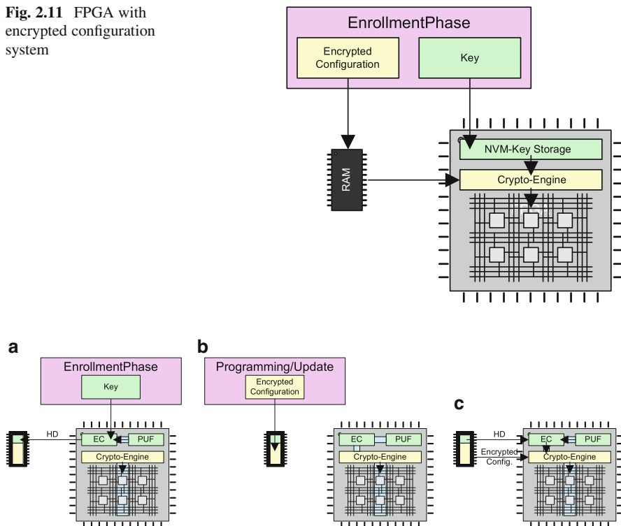
Fig. 2.12 FPGA with PUF code protection: (a) Enrollment phase: generating the helper data; (b) Storing the encrypted configuration data; (c) FPGA configuration
