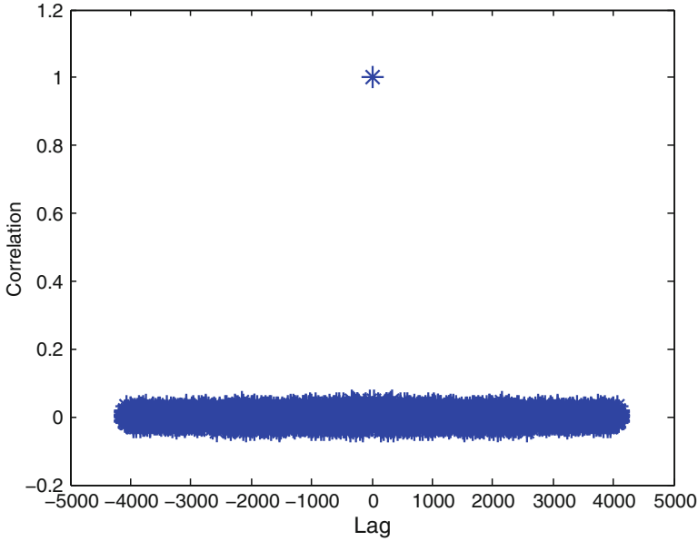
Fig. 4.6 Autocorrelation of the PUF
