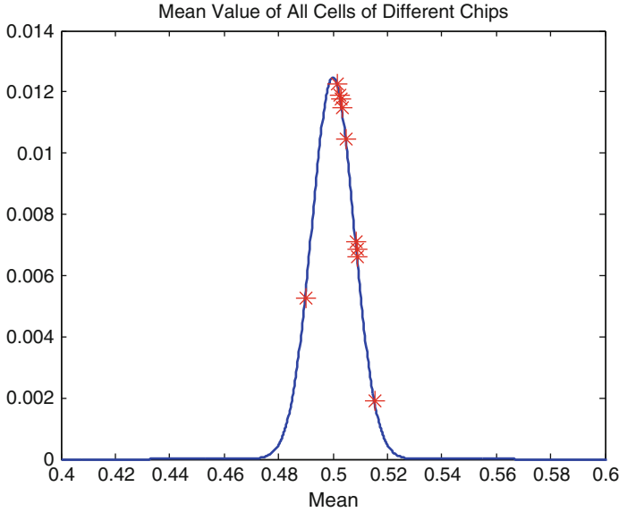
Fig. 4.3 Measured mean values on top of a binomial distribution
