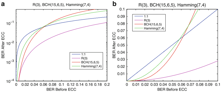
Fig. 5.6 Comparison of R, BCH and Hamming code. (a) Logarithmic scale; (b) Linear scale
