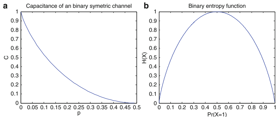
Fig. 5.2 (a) Channel capacity; (b) Binary entropy
