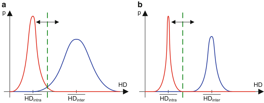
Fig. 3.3 (a) Small number of PUF cells; (b) Large number of PUF cells
