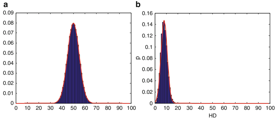
Fig. 4.2 (a) Binomial distribution: n = 100 , p = 0.5 , q = 0.5 (blue bars); Gaussian distribution: \mu = 50 , \sigma = 5 (red curve); (b) Binomial distribution: n = 100 , p = 0.08 , q = 0.92 (blue bars); Gaussian distribution: \mu = 8 , \sigma = 2.713 (red curve)
