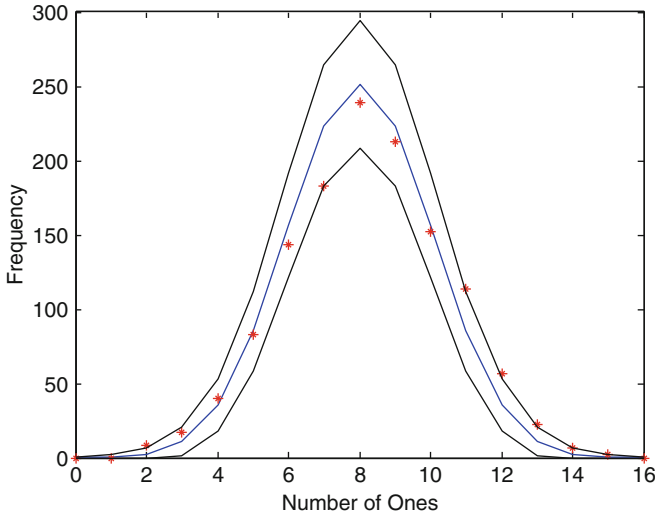
Fig. 4.13 Distribution of mean of blocks of 16 cells
