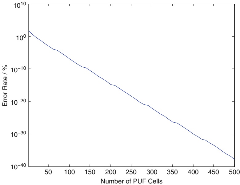
Fig. 3.4 Relation between n , FAR, and FRR
