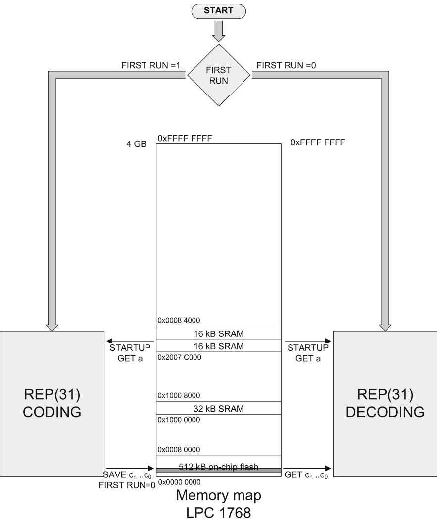
Fig. 15.2 Memory map and concept of the microcontroller SRAM PUF
