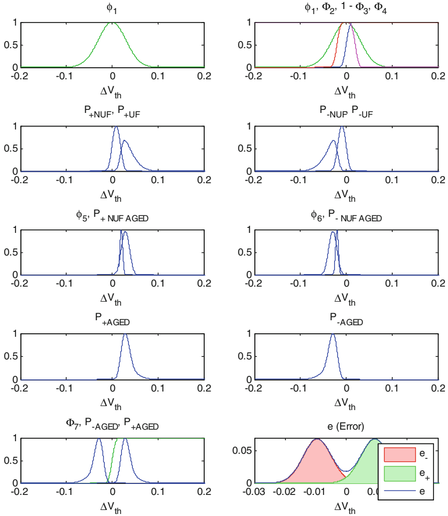
Fig. 11.8 Matlab simulation of increasing only NUF cells
