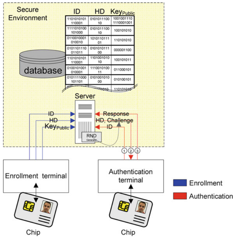
Fig. 3.12 Software-based CRPs with public-key cryptography
