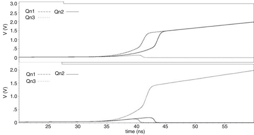
Fig. 1.18 Three different (Monte Carlo simulation) SRAM cells are powered-up (slow increase of V_{DD} ). The latching takes place as soon as the dominant transistor reaches V_{TH}
