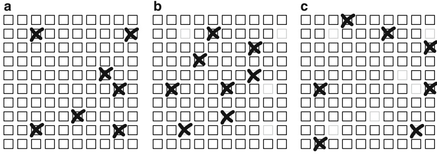
Fig. 10.3 (a) Unstable PUF cells at 25 °C; (b) Unstable PUF cells at −40 °C (c) Unstable PUF cells at 120 °C
