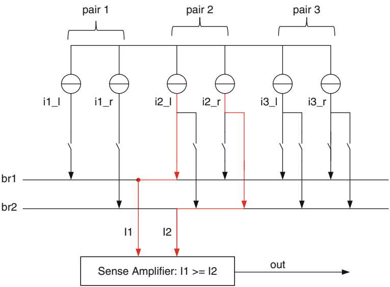
Fig. 9.5 Initial read-out of pair2
