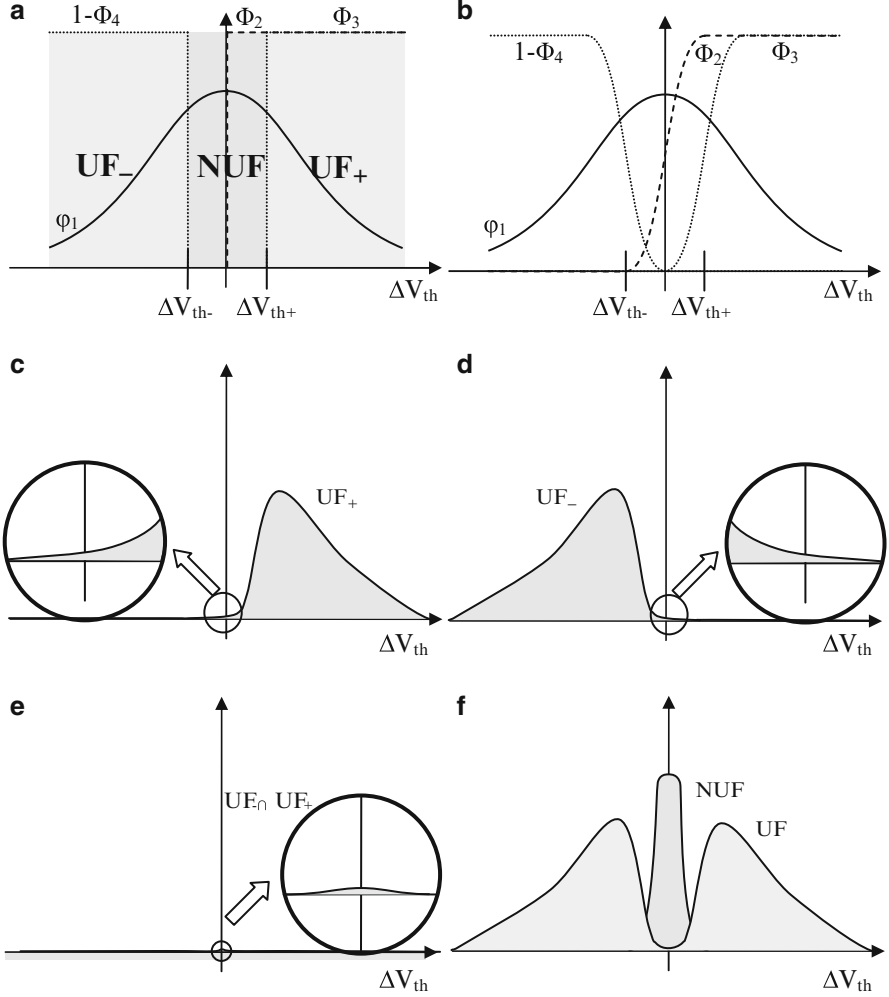
Fig. 10.9 (a) Ideal distributions \Phi_1 - \Phi_4 . (b) Real distributions \Phi_1 - \Phi_4 . (c) Useful PUF-cells with positive mismatch ( UF_+ ). (d) Useful PUF-cells with negative mismatch ( UF_- ). (e) PUF-cells which occur in UF_+ and UF_- . (f) Useful PUF-cells ( UF ) and not-useful PUF-cells ( NUF )
