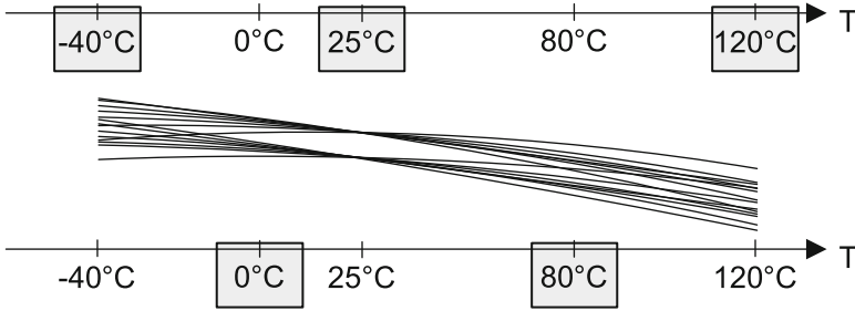
Fig. 10.4 Temperature dependence of mismatch components
