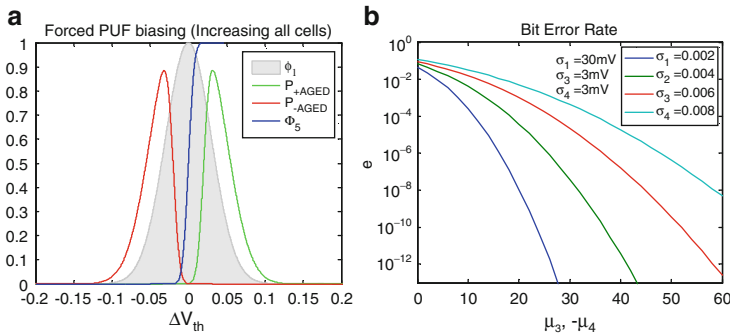
Fig. 11.6 (a) Matlab simulation results for mismatch increase of all cells; (b) Error rate
