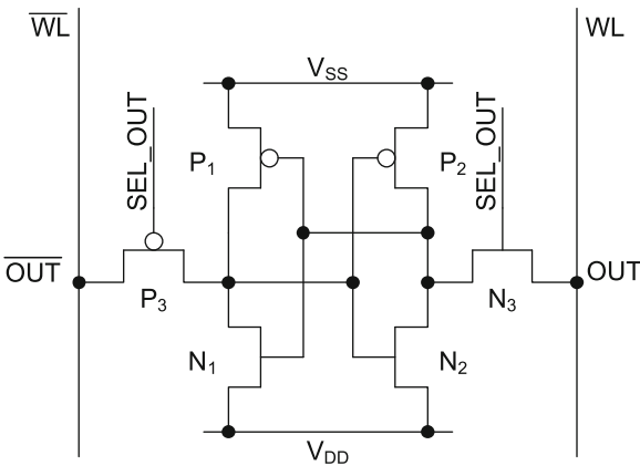
Fig. 1.21 Asymmetrical layout (see P_3 and N_3 ) of the CDP1822R SRAM cell
