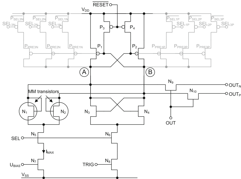
Fig. 14.2 Circuit of test chip 3
