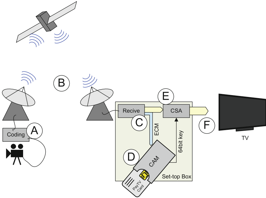
Fig. 2.3 Transmission system and conditional access system
