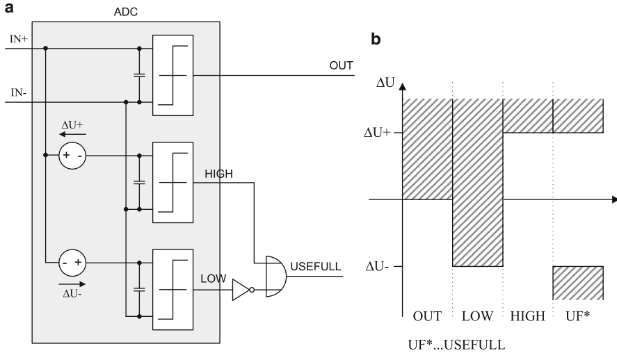
Fig. 10.8 (a) Three step ADC; (b) Diagram to illustrate the function of the ADC (gray: voltages where output gets ‘1’)
