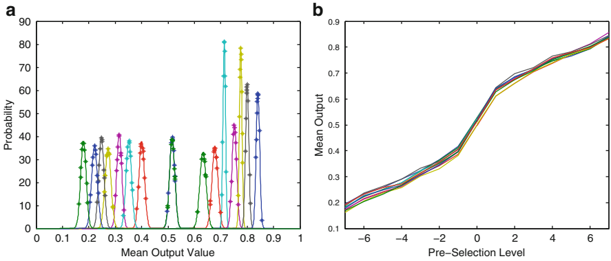
Fig. 14.8 Mean of the test chip with preselection: (a) Distribution of mean output at different preselection levels; (b) Mean output in dependence of the preselection level
