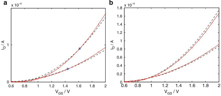
Fig. 7.3 Sources of temperature-dependent errors. (a) The crossing (blue marker) moves depending on the temperature. (b) I_{D1} (solid) and I_{D2} (dashed) at two different temperatures
