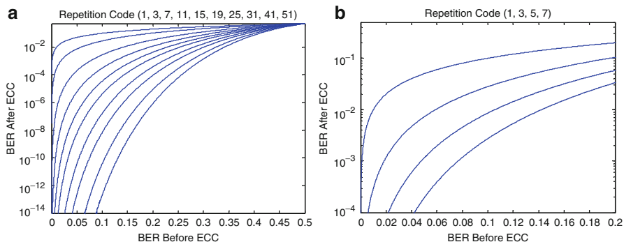
Fig. 5.8 BER of the repetition code; (a) Rep(1) - Rep(51); (b) Rep(1) - Rep(7)
