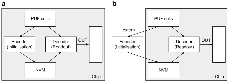
Fig. 5.4 ECC encoder: (a) On chip encoder; (b) External encoder
