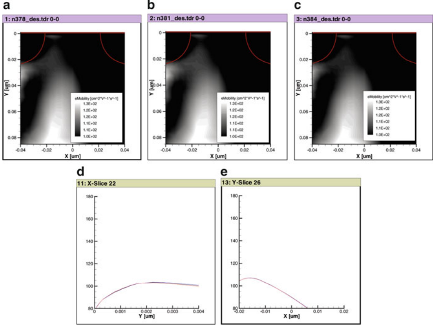
Fig. 7.15 Electron Mobility vs DC_{ch} at 27°C: (a) nominal (green), (b) low (blue), (c) high (red). (d) Y-cut @ x = -0.001\mu , (e) X-cut @ y = 0.002\mu m
