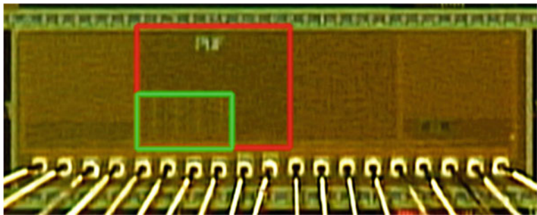
Fig. 13.1 Photograph of the test chip
