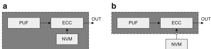
Fig. 5.3 PUF with error correction (a) On chip NVM; (b) External NVM
