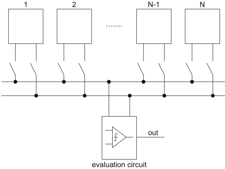
Fig. 4.11 Cells with shared sense amplifier circuitry
