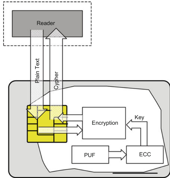
Fig. 3.5 Basic concept of encryption with PUFs
