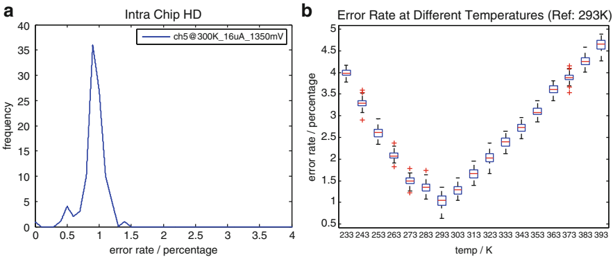
Fig. 12.5 Two stage PUF; (a) Intra chip Hamming distance HD_{intra} (100 runs); (b) HD_{intra} at different temperatures
