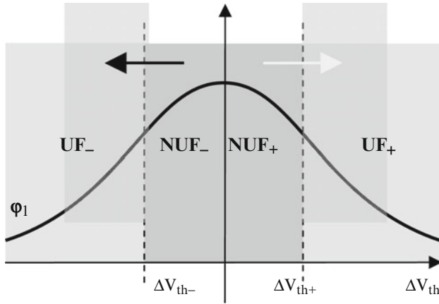
Fig. 11.1 Increasing the mismatch of the PUF cells
