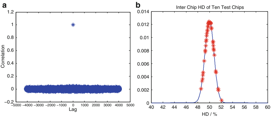
Fig. 12.6 Two stage PUF; (a) Correlation between bits; (b) Correlation between chips
