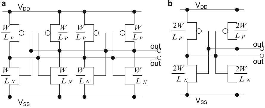
Fig. 9.1 Parallelization of PUF cells; (a) Parallelization of two SRAM cells; (b) Equivalent circuit of two parallelized SRAM cells
