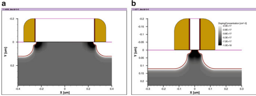
Fig. 7.9 (a) Long channel device (1 \mu\text{m} ) and (b) minimum channel device (60 nm) with halo implants
