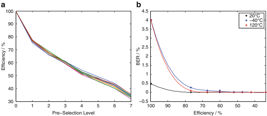
Fig. 14.9 Effects of preselection on test chips: (a) Level vs. efficiency; (b) Efficiency vs. BER at different temperatures
