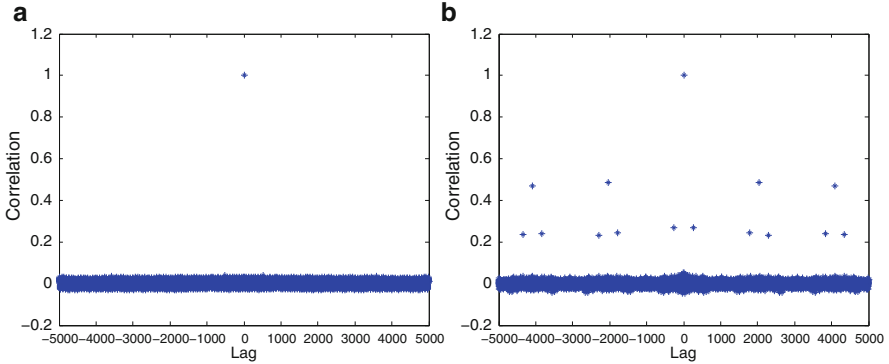
Fig. 15.7 (a) Autocorrelation of block A; (b) Autocorrelation of block B
