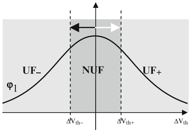
Fig. 10.6 The mismatch is divided into three classes: Useful PUF cells with positive mismatch ( UF_+ ), useful PUF cells with negative mismatch( UF_- ) and not useful PUF cells (NUF)
