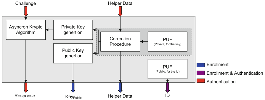
Fig. 3.13 Block diagram of a chip with public key-based CRP generation
