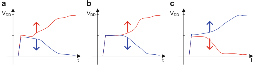
Fig. 1.16 Bistable electronic circuit (e.g., SRAM): (a) Bias toward “0”; (b) 50/50 chance; (c) Bias toward “1”
