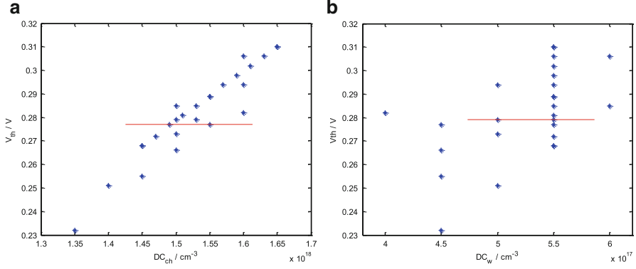
Fig. 7.12 (a) V_{TH} vs. channel doping concentration. (b) V_{TH} vs. substrate doping concentration
