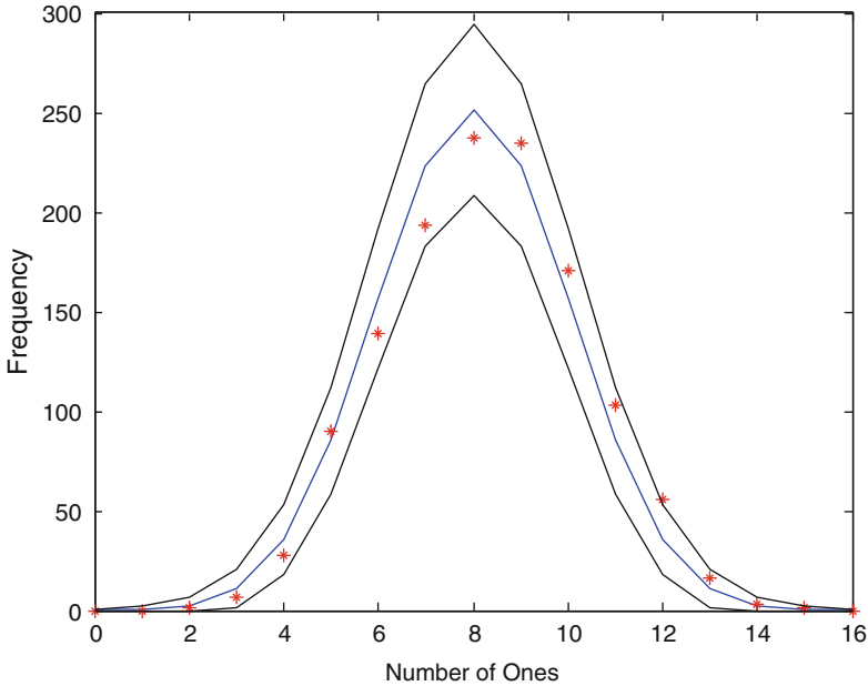
Fig. 13.9 Distribution from second block of second test chip
