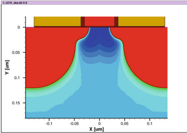
Fig. 7.10 Doping profile of a halo-doped minimum channel device
