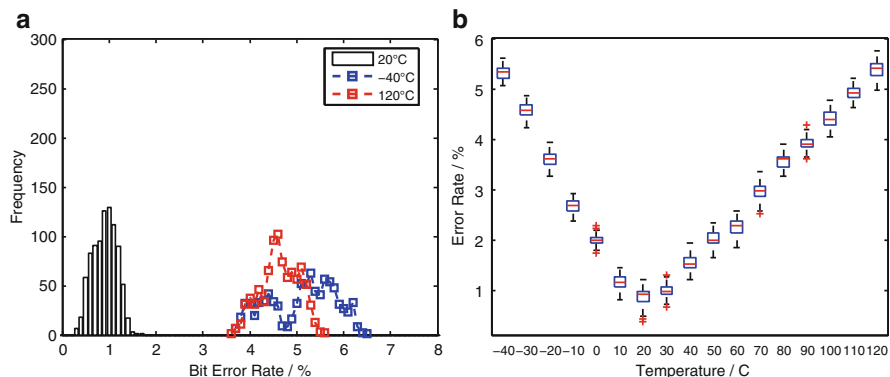
Fig. 13.4 PUF with shared sense amplifier: (a) Intra-chip Hamming distance HD_{intra} (100 runs); (b) HD_{intra} at different temperatures
