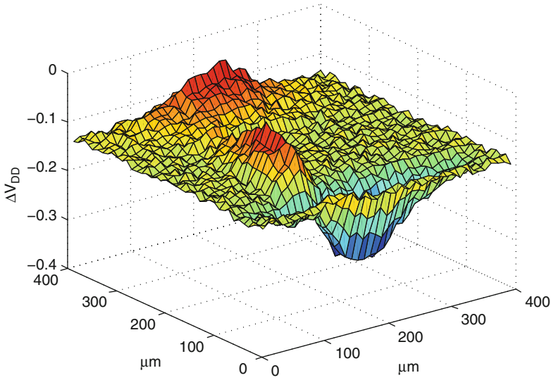
Fig. 6.2 The figure shows the V_{DD} values at different regions of a chip. These values come from a simulation
