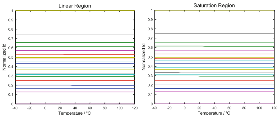
Fig. 6.13 The normalized I_D vs temperature in linear ( left ) and saturation ( right ) region is shown. In the used BSIM model no temperature coefficient mismatch is included and thus no crossings occur
