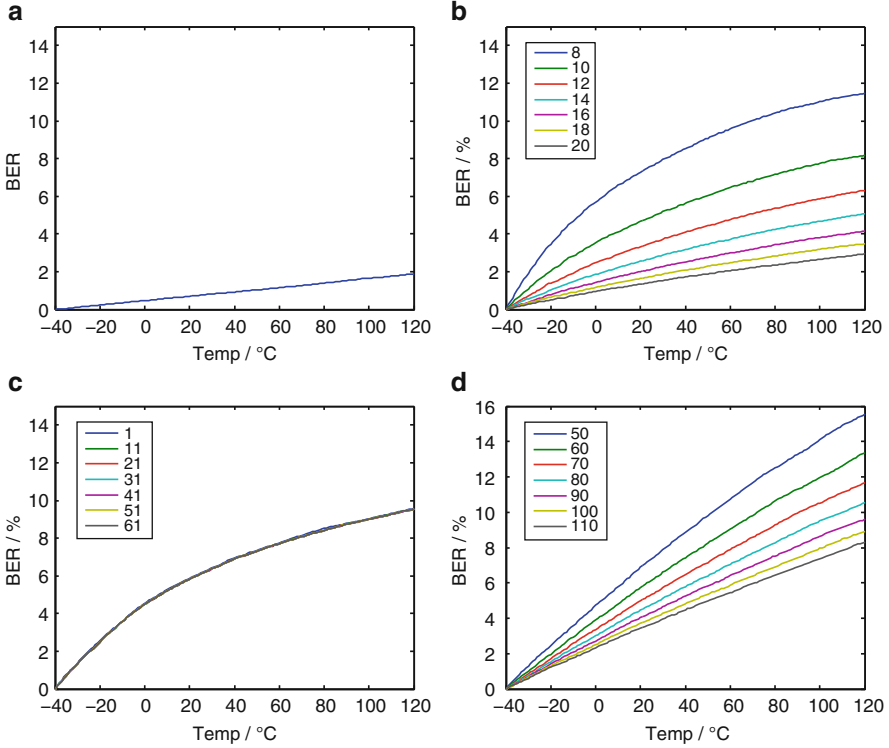
Fig. 7.23 (a) Regular mismatch model. (b) Correlated (w.r.t. VTH0 mismatch) KT1 mismatch (different fact_kt1). (c) Uncorrelated (w.r.t. VTH0 mismatch) KT1 mismatch (different fact_kt1) added to correlated KT1 mismatch. (d) Correlated (w.r.t. U0 mismatch) UTE mismatch (different fact_ute)
