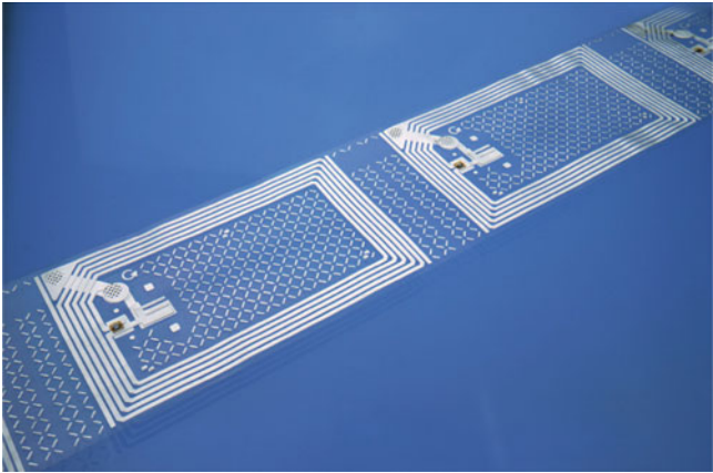
Fig. 1.25 My-d tags from Infineon Technologies (carrier frequency = 13.56 Mhz)
