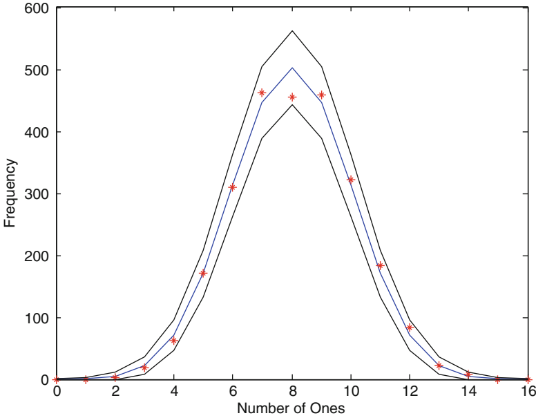
Fig. 13.8 Distribution of ones in a block of 16: First test chip (two-stage PUF)
