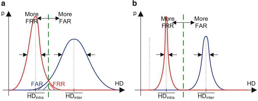
Fig. 4.14 False acceptance rate (FAR) and false rejection rate (FRR): (a) Small number of PUF cells; (b) Large number of PUF cells
