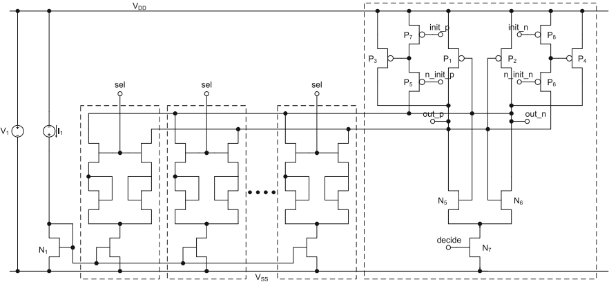
Fig. 10.14 PUF-cells with shared sense amplifier
