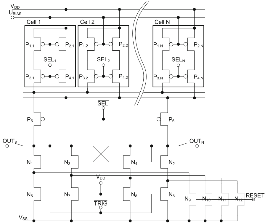
Fig. 13.2 PUF circuit with shared sense amplifier
