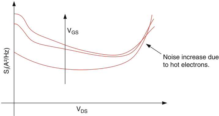
Fig. 6.18 In short channel devices thermal noise increases for high values of V_{DS} caused by occurrence of hot electrons. The figure is inspired by [16]
