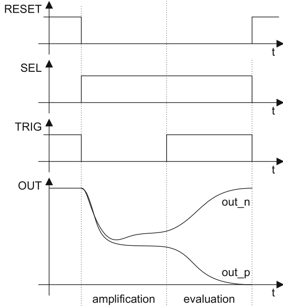
Fig. 14.3 Timing diagram of the different control signals
