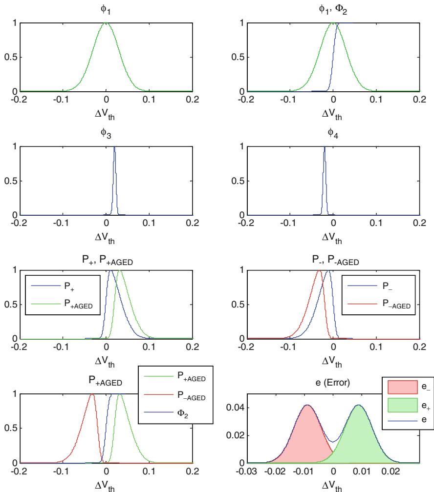
Fig. 11.5 Matlab simulation of increasing all cells
