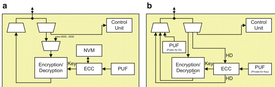
Fig. 3.6 (a) Helper data stored on the chip; (b) Helper data stored on a external database
