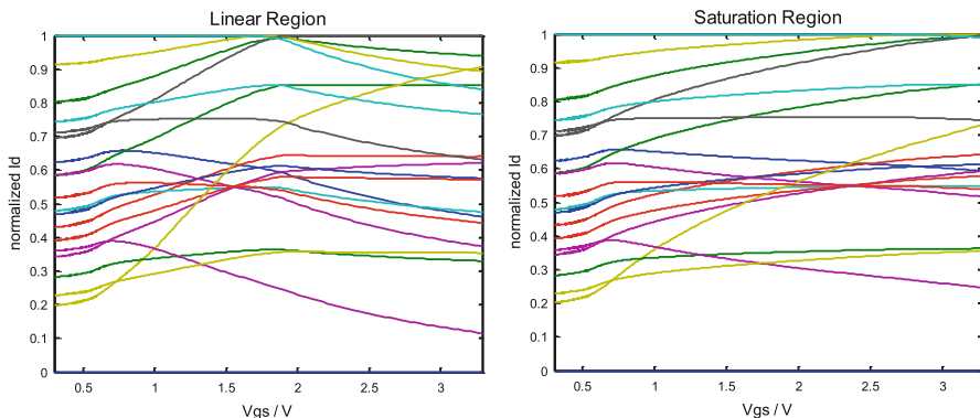
Fig. 6.12 The normalized I_D vs V_{GS} in linear ( left ) and saturation ( right ) region is shown. This graph is important to show the occurrence of crossings at different V_{GS} . These crossings may produce errors at the PUF's output if V_{GS} changes during operation
