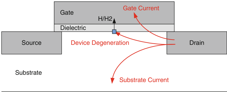
Fig. 6.6 The hot charge carriers have different effects on the transistor which result in leakage current and device degeneration
