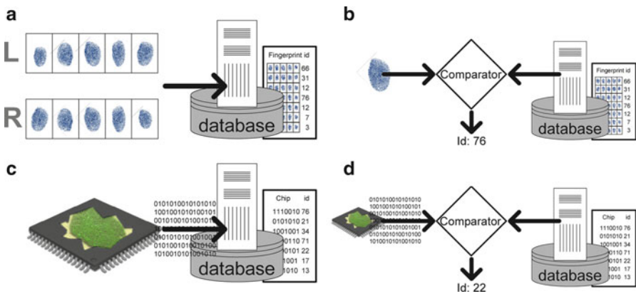
Fig. 1.30 Comparison of Biometric and PUF identification: (a) Enrollment fingerprint; (b) Identification fingerprint; (c) Enrollment PUF; (d) Identification PUF
