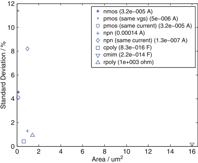
Fig. 6.24 Typical mismatch of different components
