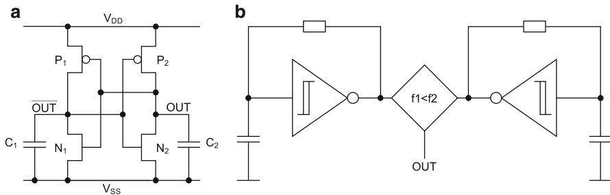
Fig. 6.22 Examples of capacitor-based PUFs: (a) SRAM with mismatch capacitors; (b) Capacitor-based PUF using Schmitt-Triggers
