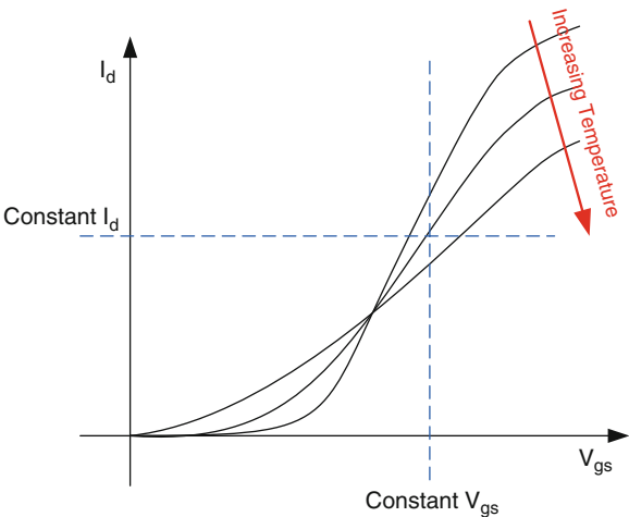
Fig. 6.16 The temperature behavior of MOS transistors is shown. If I_D is fixed over temperature, V_{GS} will change and the other way round. Since PUFs are sensitive to V_{GS} changes, it is helpful to fix V_{GS} in current source driven PUFs
