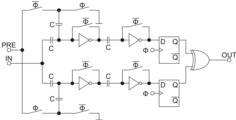
Fig. 1.14 Stable cell detector
