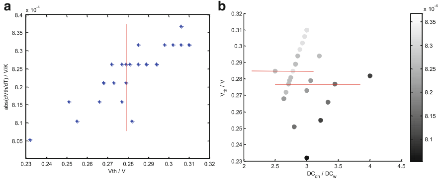
Fig. 7.13 (a) V_{TH} vs. \left| \frac{dV_{TH}}{dT} \right| . Red line: Same V_{TH} , different \frac{dV_{TH}}{dT} . (b) \left| \frac{dV_{TH}}{dT} \right| (gray scale) vs. doping ratio and V_{TH} . The lines show transistors of the same V_{TH} but different temperature coefficients
