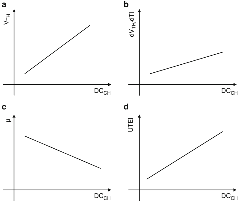
Fig. 7.20 The overview of the TCAD simulation results shows the behavior of different parameters versus a change of doping concentration
