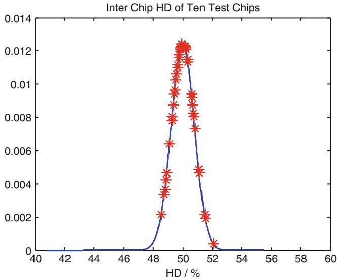
Fig. 4.7 Inter-chip Hamming distance of the ten test chips on binomial distribution
