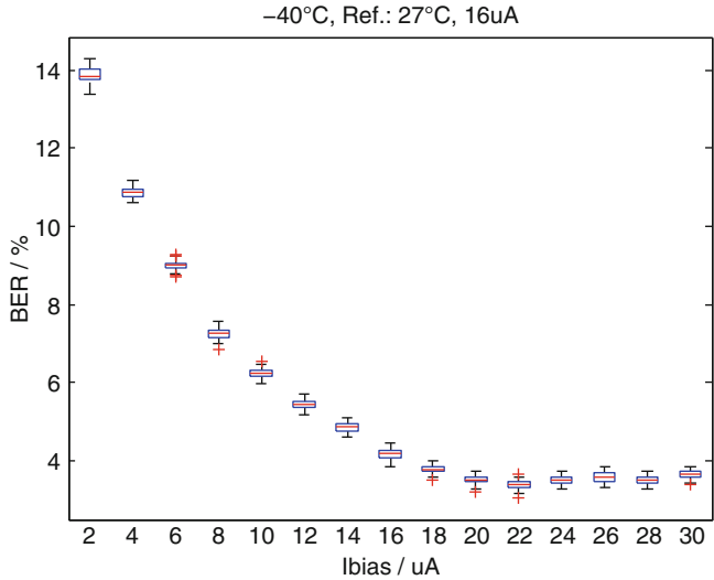
Fig. 6.17 If the bias current is adjusted, the error rate can be reduced. At -40^\circ C the minimum error rate appears not at 16 \mu A but at 22 \mu A
