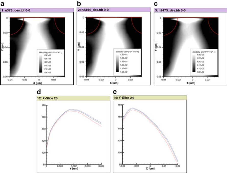
Fig. 7.18 Electron Mobility vs DC_{sub} at -73^{\circ}\text{C} : (a) nominal (green), (b) low (blue), (c) high (red). (d) Y-cut @ x = -0.001\text{ }\mu\text{m} , (e) X-cut @ y = 0.002\text{ }\mu\text{m}
