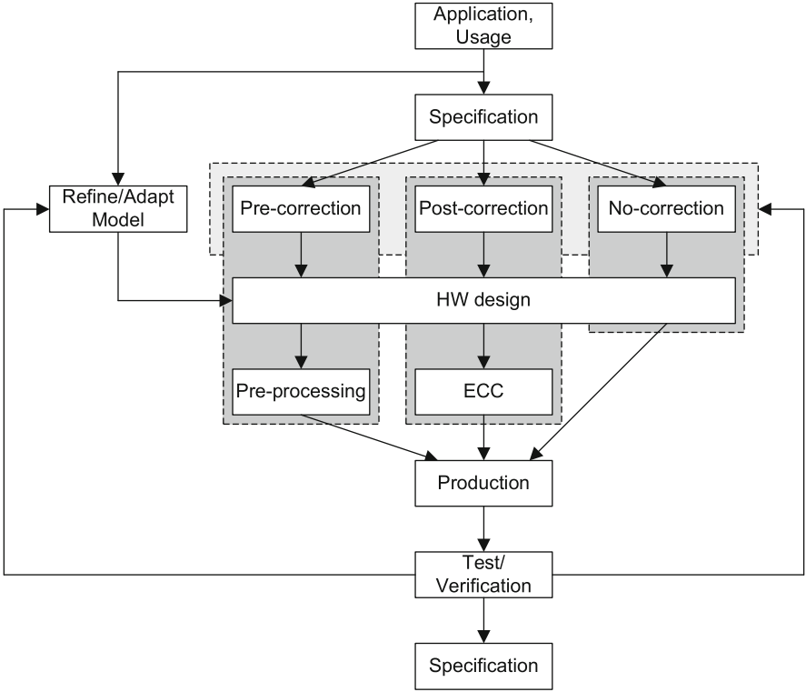
Fig. 16.1 PUF-design workflow
