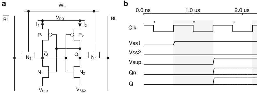
Fig. 10.23 Preselection using V_{SS} pins E_{med} (a); Timing diagram (b)
