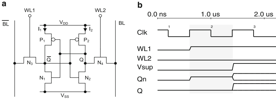
Fig. 10.25 Preselection using WL pins (a) Schematic. E_{med} ; (b) Timing diagram
