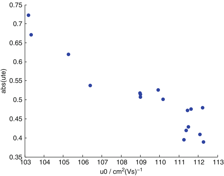
Fig. 7.19 | UTE | vs electron mobility for different doping concentrations
