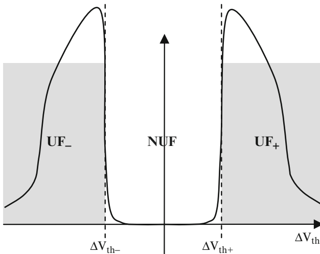
Fig. 11.3 Increase of the mismatch
