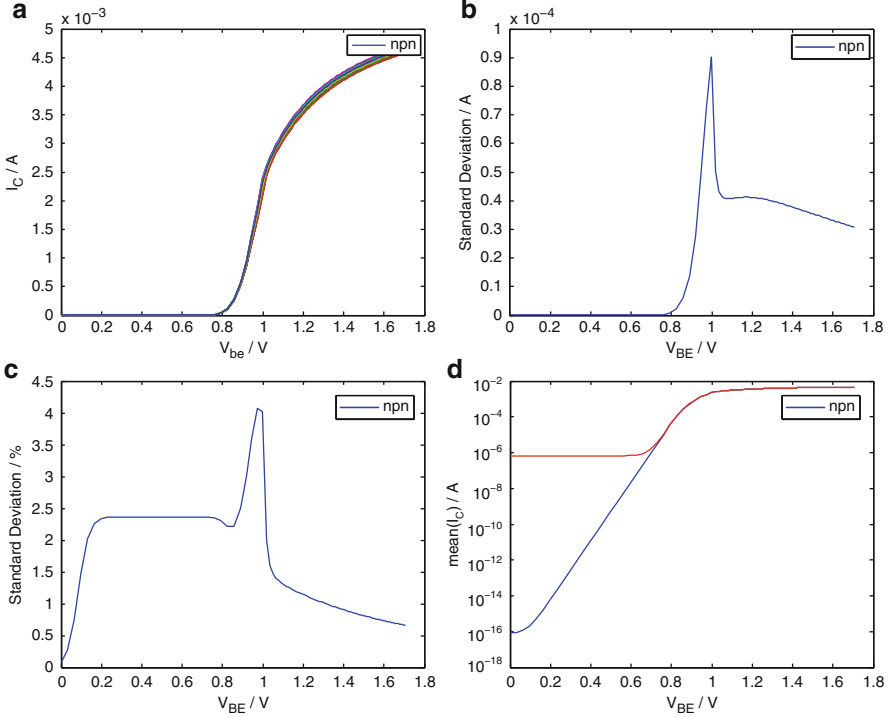
Fig. 6.23 Influence of mismatch at different V_{BE} : (a) I_C vs. V_{BE} of different Monte Carlo runs. (b) Standard deviation of I_C vs. V_{BE} in A. (c) Standard deviation of I_C vs. V_{BE} in %. (d) I_C (blue) and I_C plus standard deviation caused by transient noise (red curve)
