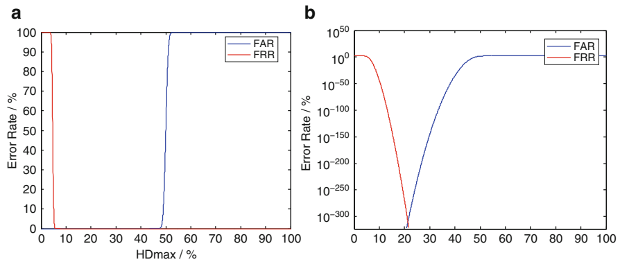
Fig. 4.16 False acceptance rate (FAR), false rejection rate (FRR) in dependence of HD_{MAX} (a) Linear scale; (b) Logarithmic scale
