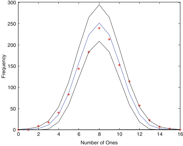
Fig. 13.7 Ideal (blue) distribution of ones in a block of 16 output bits. The red curve shows the results from the test ships. The black curves mark the 3\sigma (99,73 %) confidential interval
