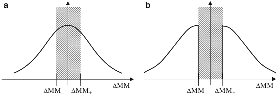
Fig. 8.2 (a) Normal distribution; (b) Desired distribution
