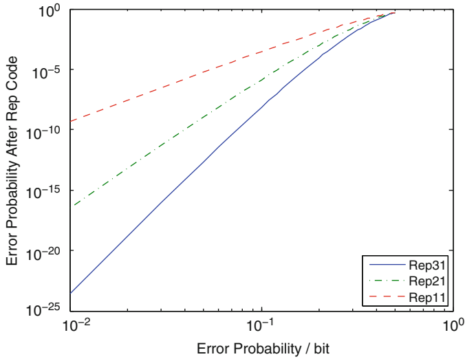
Fig. 15.4 Performance of different repetition code lengths
