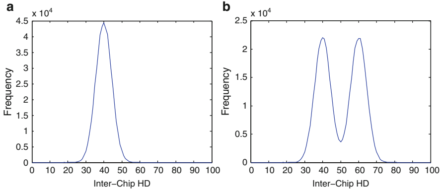
Fig. 4.8 HD_{inter} : (a) 20 % of the cells of a chip tend to “1”; (b) 20 % of the cells of a chip correlate
