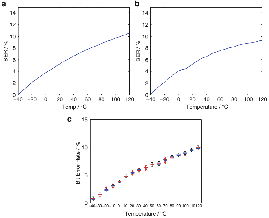
Fig. 7.24 (a) Matlab model (KT1 and UTE mismatch). (b) Adapted Spectre model (KT1 and UTE mismatch, 5000 Monte Carlo runs). (c) Measurement results
