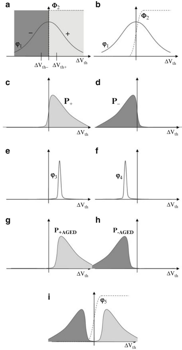
Fig. 11.4 (a) Ideal distributions \Phi_1, \Phi_2 ; (b) Real distributions \Phi_1, \Phi_2 ; (c) Positive PUF-cells ( P_+ ); (d) Negative PUF-cells ( P_- ); (e) Positive increase \phi_3 ; (f) Negative increase \phi_4 ; (g) Positive increased area P_{+AGED} ; (h) Negative increased area P_{-AGED} ; (i) Distribution of all cells after aging
