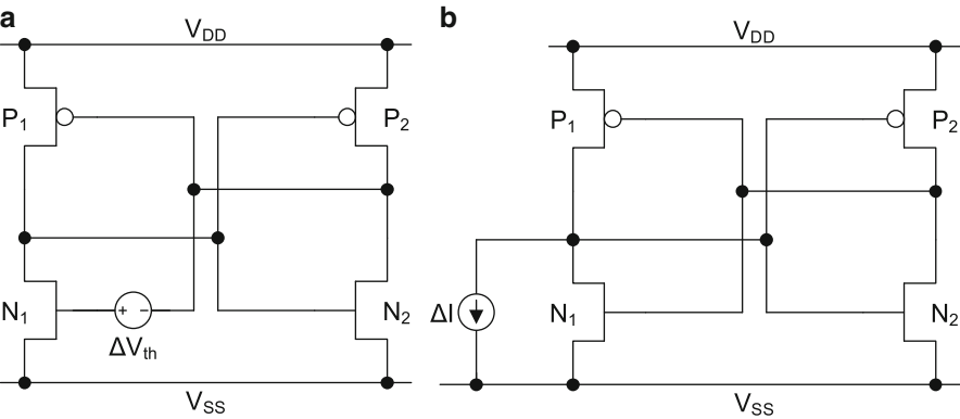
Fig. 10.11 (a) SRAM cell with additional voltage source at the gate of N_1 ; (b) SRAM cell with additional current source at the drain of N_1
