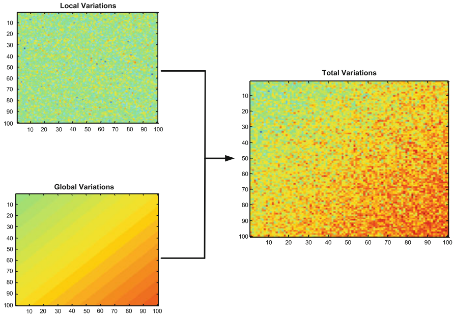
Fig. 6.1 The figure above shows the influence of local and global mismatches. The global mismatch introduces a gradient on the parameter which leads to an overall (see right hand side) non-Gaussian variability distribution. This can lead to a biased PUF output
