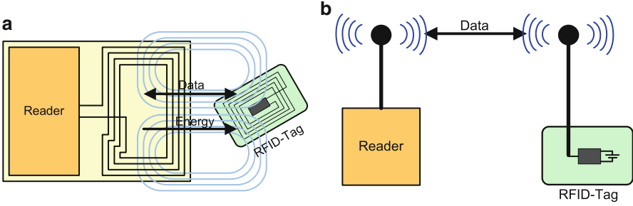
Fig. 1.26 (a) Passive RFID tag; (b) Active RFID tag
