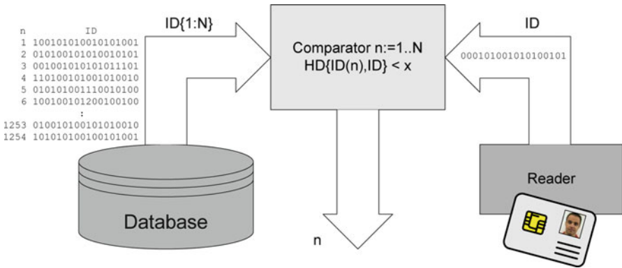
Fig. 3.2 Identification process with a PUF
