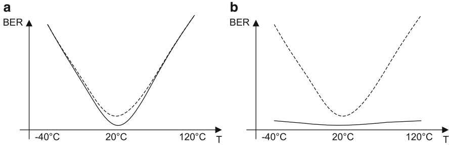
Fig. 10.5 BER in dependence of the temperature before ( dotted line ) and after preselection multiple readout ( solid line ) (a) At one temperature (20 °C); (b) At three temperatures (-40 °C, 20 °C and 120 °C)
