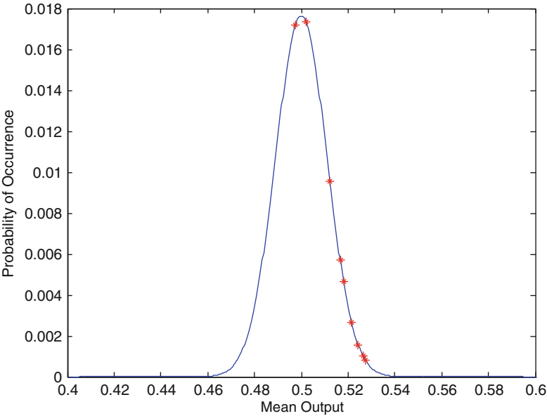
Fig. 14.4 Mean output values of 10 packaged test chips
