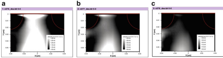
Fig. 7.14 Electron mobility at (a) -73^{\circ}\text{C} , (b) 27^{\circ}\text{C} , (c) 117^{\circ}\text{C}
