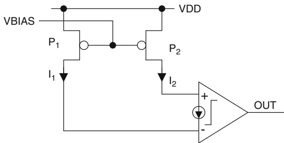
Fig. 7.2 Circuit which describes the functionality of a two transistor PUF using an ideal current comparator
