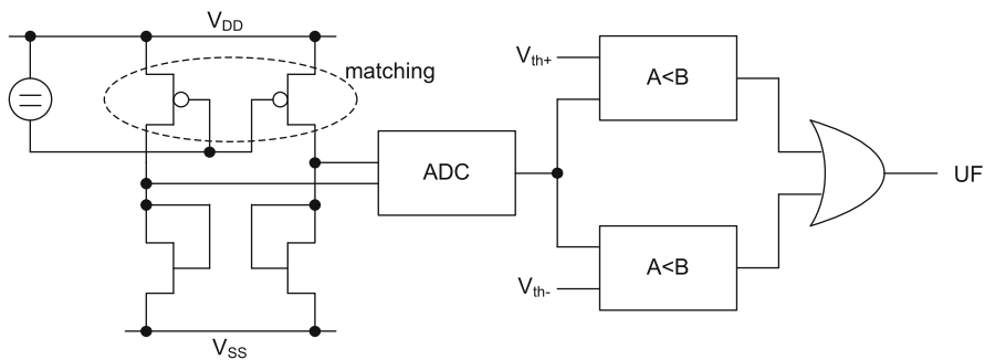
Fig. 10.7 Mismatch measurement using an ADC
