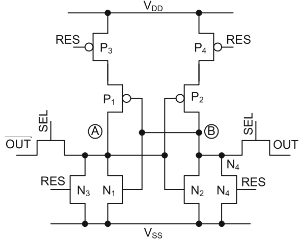
Fig. 1.12 Resettable SRAM PUF
