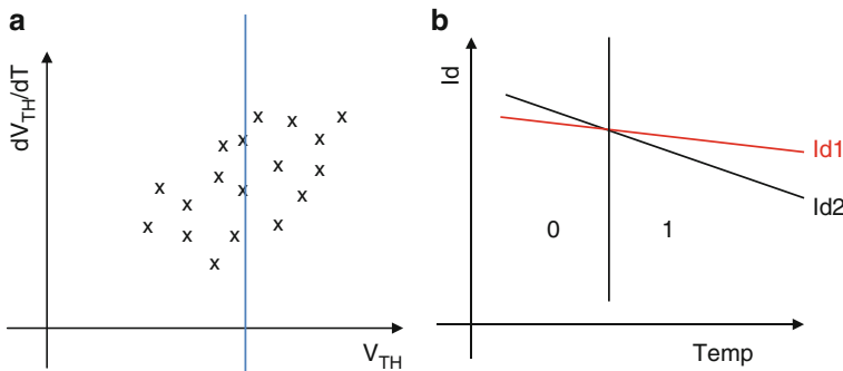
Fig. 7.4 (a) Sketch of measurement results: same V_{TH} but different temperature coefficients. (b) If the temperature coefficients differ, crossings cause errors: OUT = 0 (left), OUT = 1 (right)
