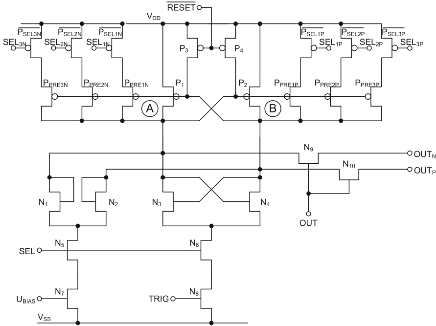
Fig. 14.7 PUF cell with preselection circuitry
