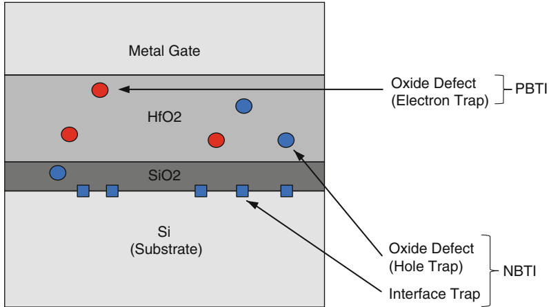
Fig. 6.4 Part of transistor with HfO 2 high-k dielectric and metal gate. The interface traps and the negative oxide defects lead to hole traps and thus NBTI. The positive oxide defects lead to electron traps and thus to the reversible PBTI
