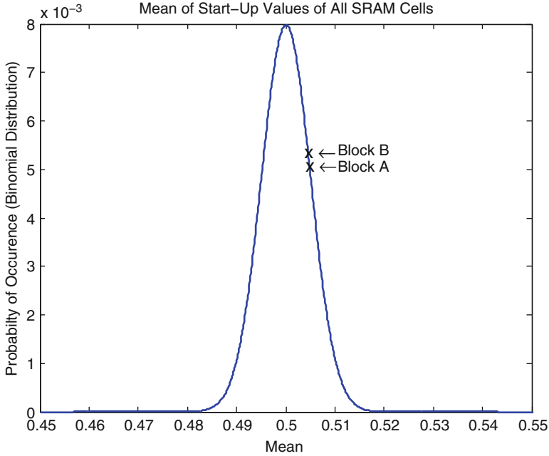
Fig. 15.5 Mean of SRAM blocks A and B on binomial pdf
