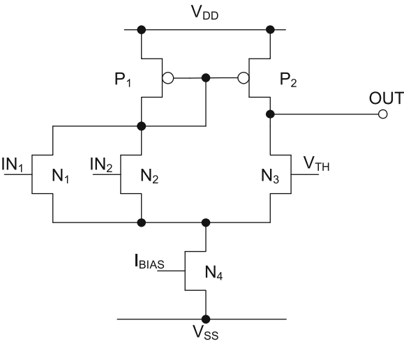
Fig. 10.20 Comparator with maximum selector
