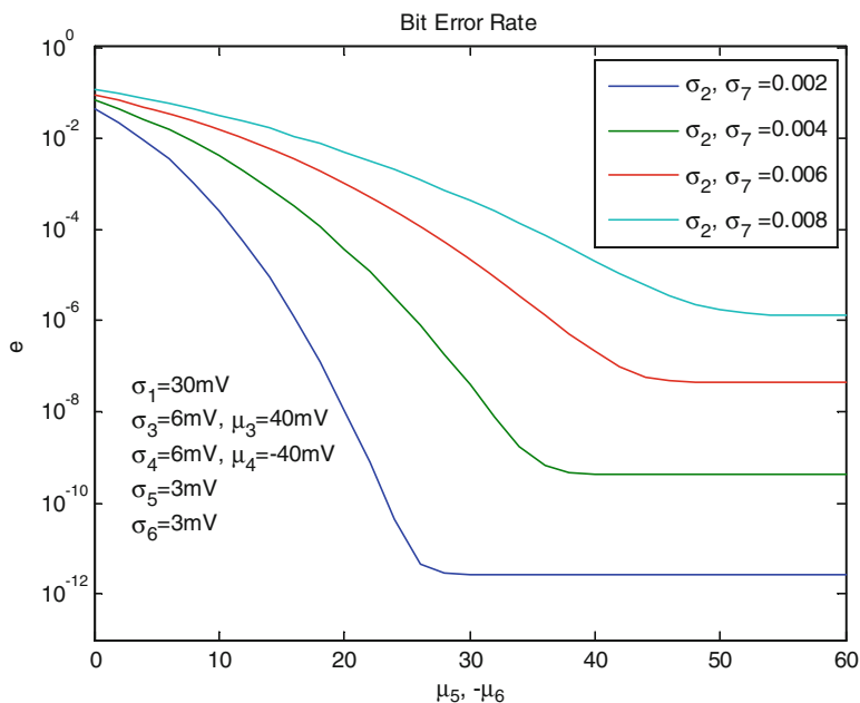
Fig. 11.10 Error rate after partial biasing
