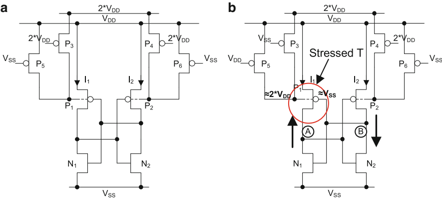
Fig. 11.12 (a) Circuit to stress the transistors with NTBI; (b) Stress of P 1
