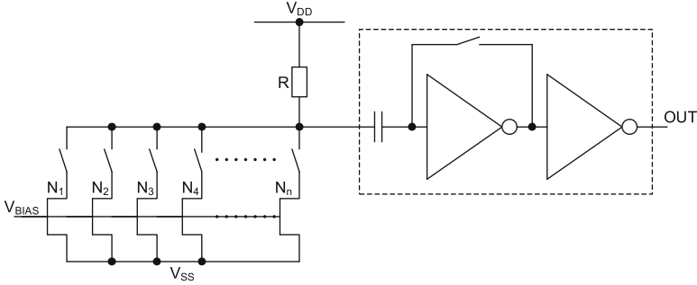
Fig. 1.6 Approach from Lofstrom
