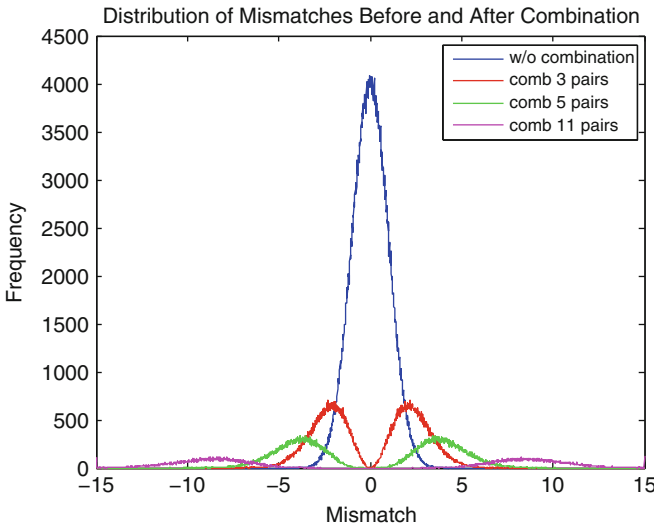
Fig. 9.2 Distribution of mismatches for different degrees of parallelization
