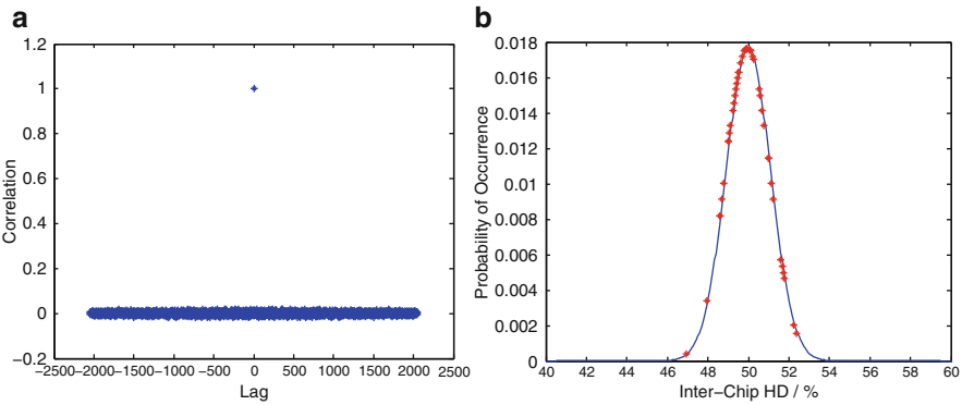
Fig. 14.6 PUF chip 3; (a) Correlation between bits; (b) Correlation between chips
