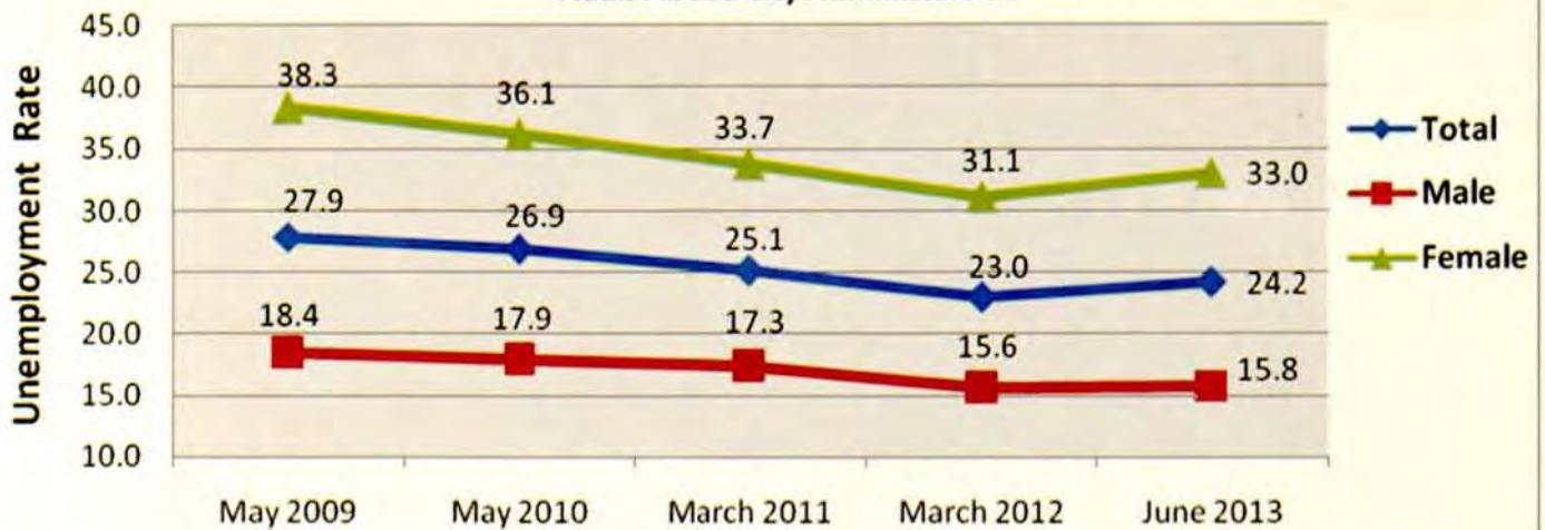
Figure 4 : Trends of Unemployment Rate by Sex During the Five Survey Periods, Addis Ababa City Administration
