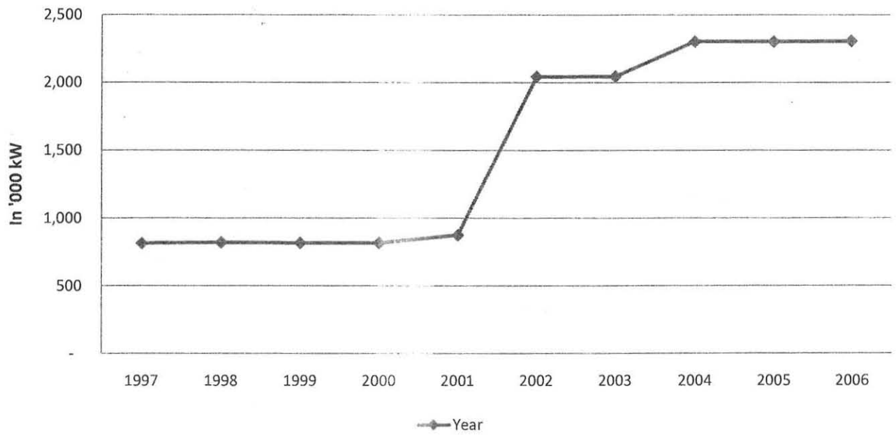
FIG VI: Installed Generating Capacity of Electricity (Hydro, Thermal, Geothermal & Wind), 1997-2006 EFY (2004/05-2013/14)
