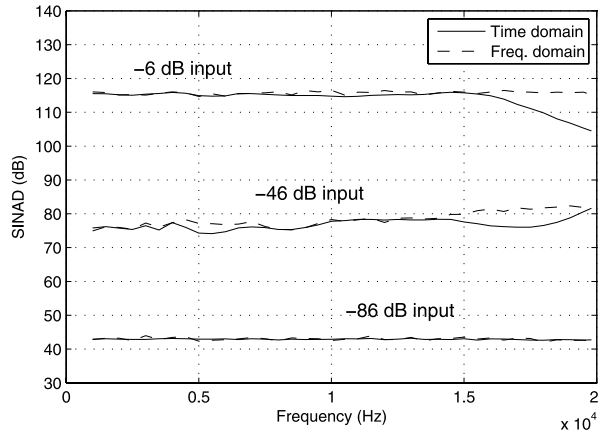
Fig. 3.6 SINAD as a function of the input frequency, measured in the time domain and in the frequency domain. For all the three time domain measurements a linearized STF with an effective quantizer gain of 1.7 is assumed. The input levels are -86 dB, -46 dB, and -6 dB. The loop filter is 5th order feed-forward filter with 100 kHz corner frequency and resonators at 12 and 20 kHz
