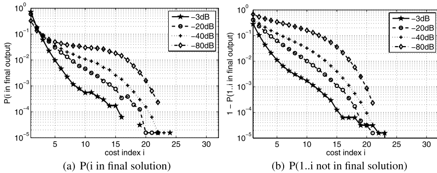
Fig. 8.2 Probability that a path is selected for the final solution as a function of its cost index (a) and the probability that the first n paths are not within the final solution (b) for SDM configuration SDM2 with N = 8 . The input signals are 1 kHz sine waves at various levels
