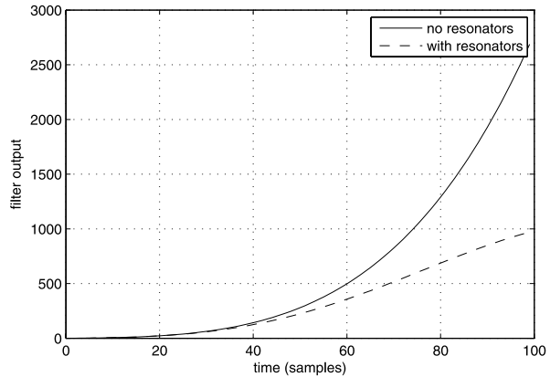
Fig. 6.4 First 100 samples of the impulse response of a fifth order loop filter with a corner frequency of 100 kHz, once with and once without resonator sections (12 kHz and 20 kHz)
