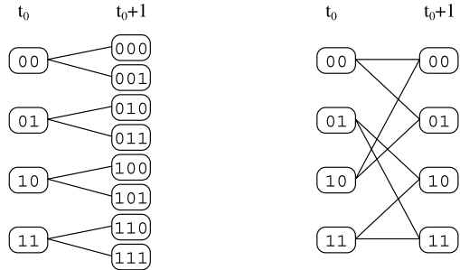
Fig. 7.2 Relationship between the Trellis depth L and the Trellis order N . The newest N bits of the 2^N sequences are different. The converter output decision is made by tracing back L clock cycles
