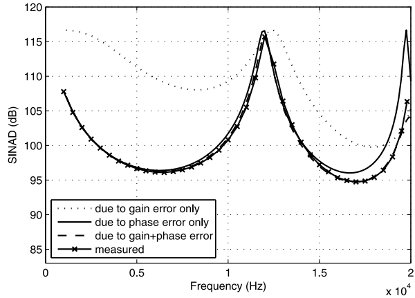
Fig. 3.4 Comparison of the predicted time domain SINAD measurement result, resulting from the individual, as well as from the combined, gain and phase deviations as predicted by the linear SDM model for a fitted quantizer gain of 1.7, with the measured time domain SINAD for a zero delay unity gain linearized STF ( -6 dB input signal)
