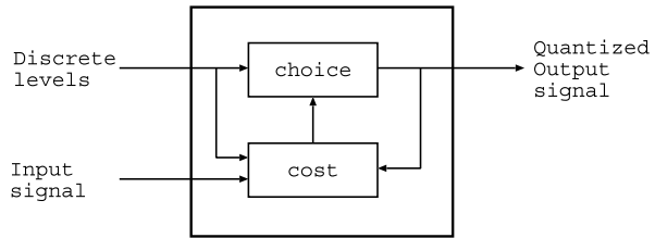
Fig. 5.2 Look-ahead enabled noise-shaping quantizer
