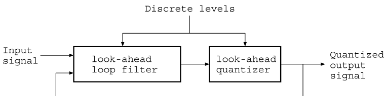
Fig. 5.3 Look-ahead enabled SDM
