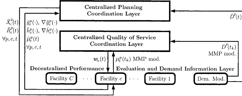
Figure 5.3. Information exchange amongst the coordination layers and the decentralized layer.
