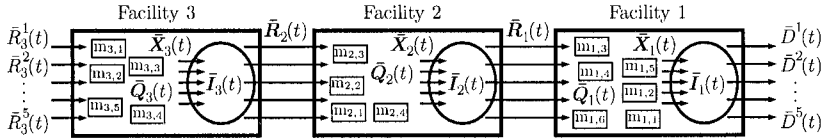
Figure 5.9. An example supply chain with 3 facilities producing 5 part types.
