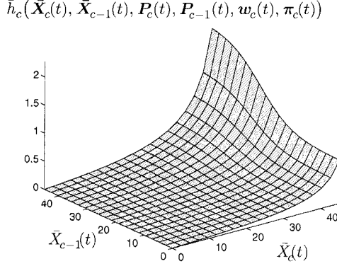
Figure 5.7. Horizontal coordination constraint function, \bar{h}_c(\bar{\mathbf{X}}_c(t), \bar{\mathbf{X}}_{c-1}(t), \bar{\mathbf{P}}_c(t), \bar{\mathbf{P}}_{c-1}(t), \mathbf{w}_c(t), \boldsymbol{\pi}_c(t)) , for a single part type system.
