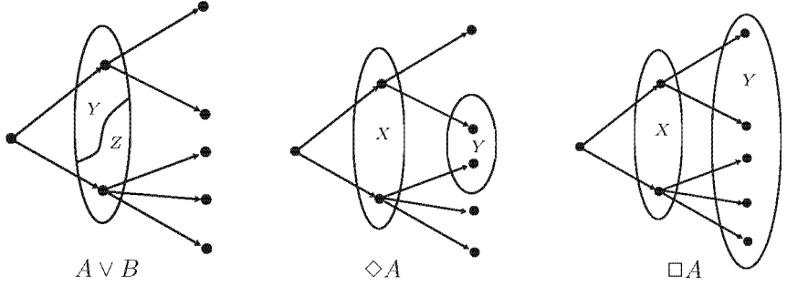
FIGURE 5. Truth definition.
