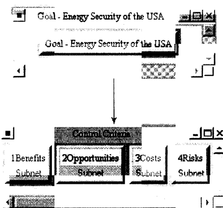
Figure 8. BOCR Model
