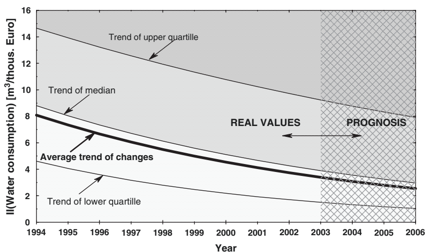
Fig. 7.7 Graphical presentation of CP Phenomenological Overall Industry Model, for water use
