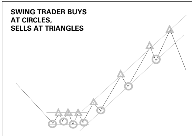
Figure 4-2: Swing trading.
