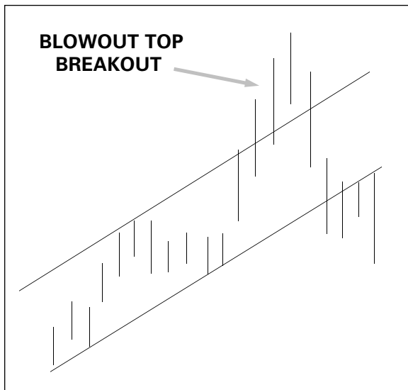
Figure 11-4: Upside breakout in an uptrend.
