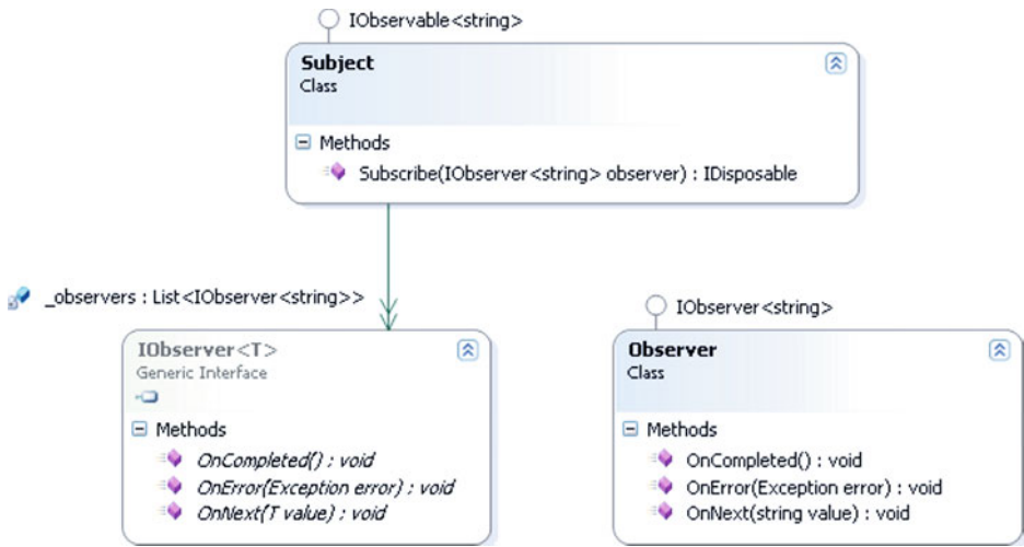
Figure 8-1. Observer-subject class relationship
