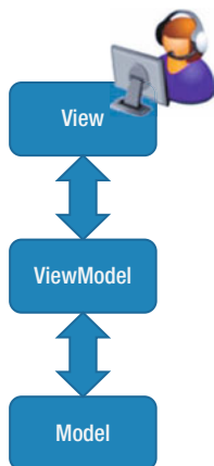
Figure 12-1. Simplified view of Model-View-ViewModel
