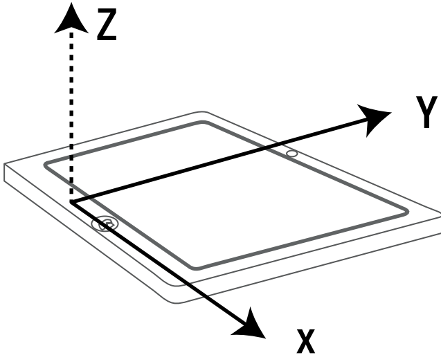
Figure 19-1. Accelerometer planes
