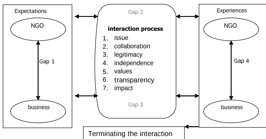
Figure 20.1. The BNI-model
